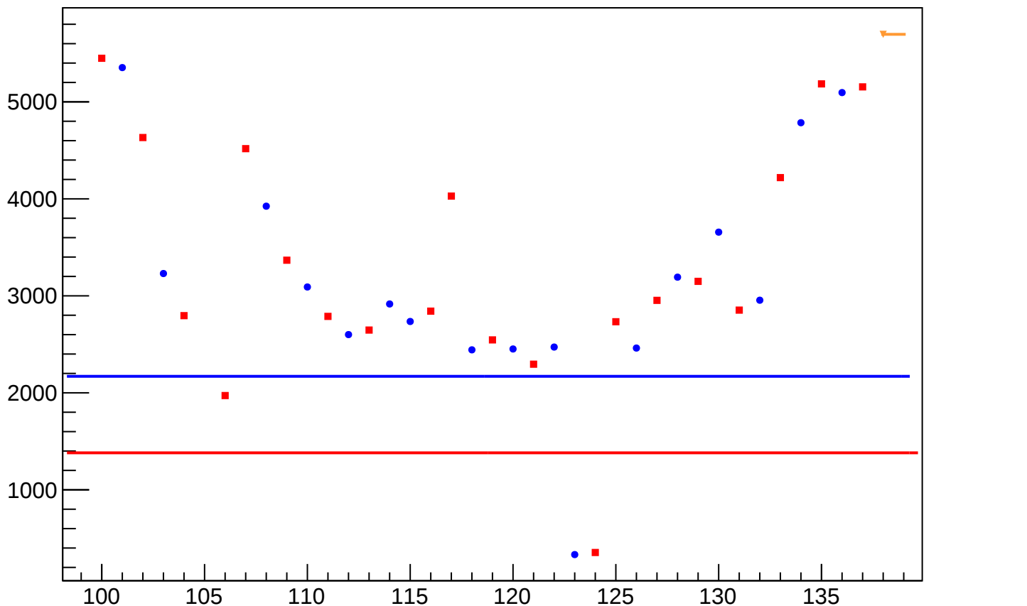
asym_atr1l2_avg_correction_rms vs Slug, Sign Corrected
