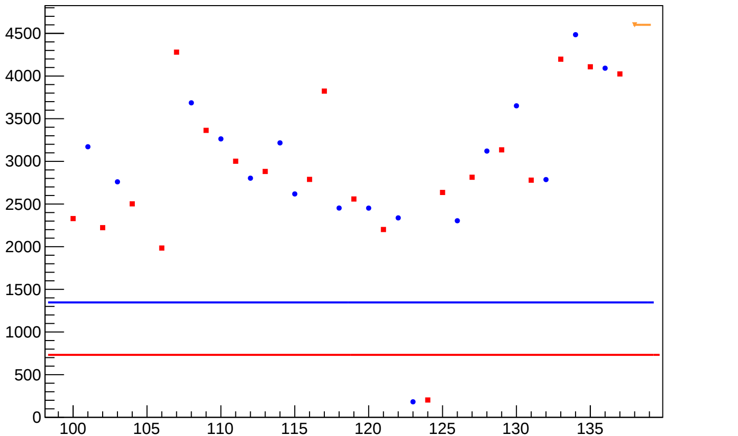
asym_atr1l2_dd_correction_rms vs Slug, Sign Corrected
