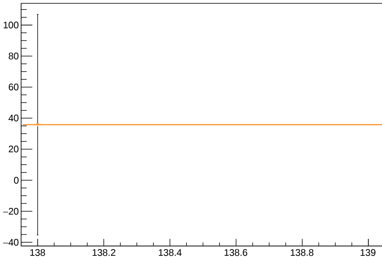
reg_asym_sam_15_26_dd_mean vs Slug, Sign Corrected
