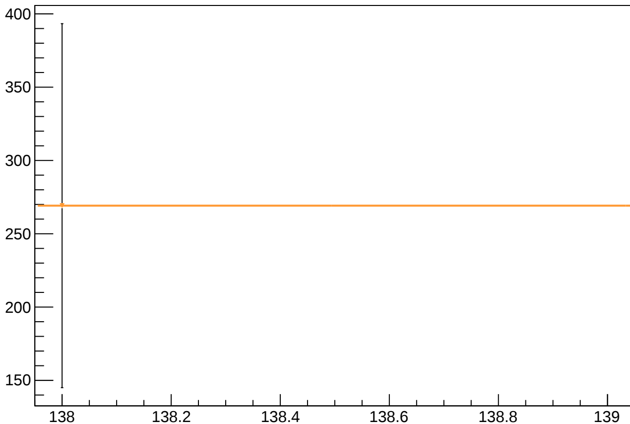
reg_asym_sam_1548_avg_mean vs Slug, Sign Corrected
