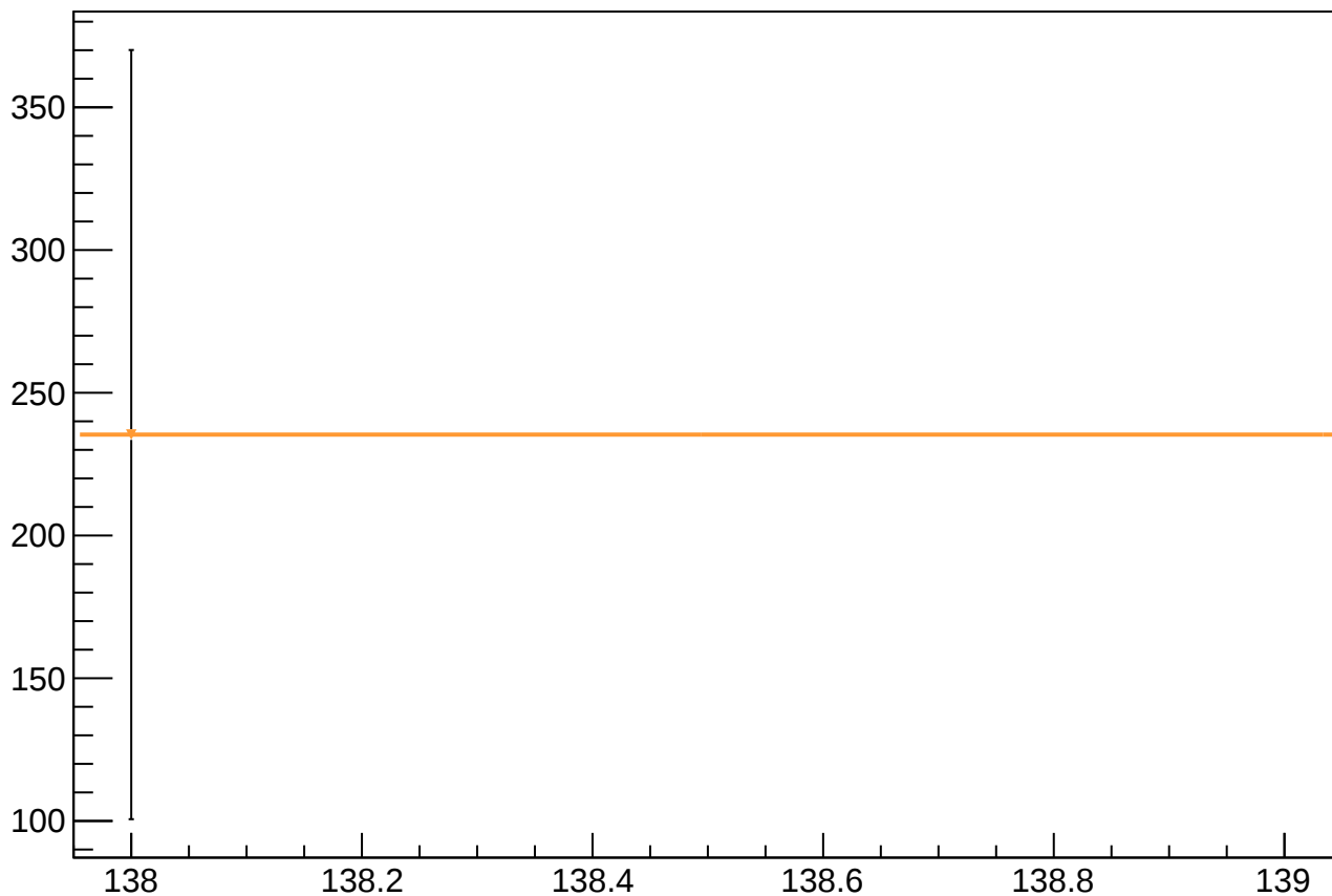
reg_asym_sam_3748_avg_mean vs Slug, Sign Corrected
