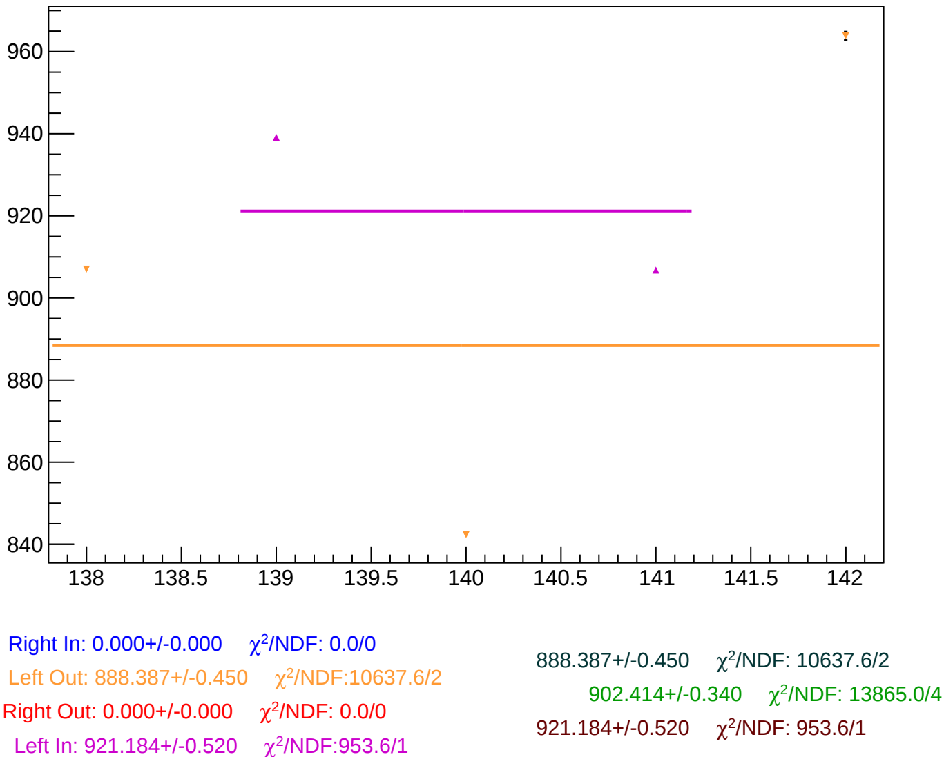
asym_sam6_correction_rms vs Slug, Sign Corrected
