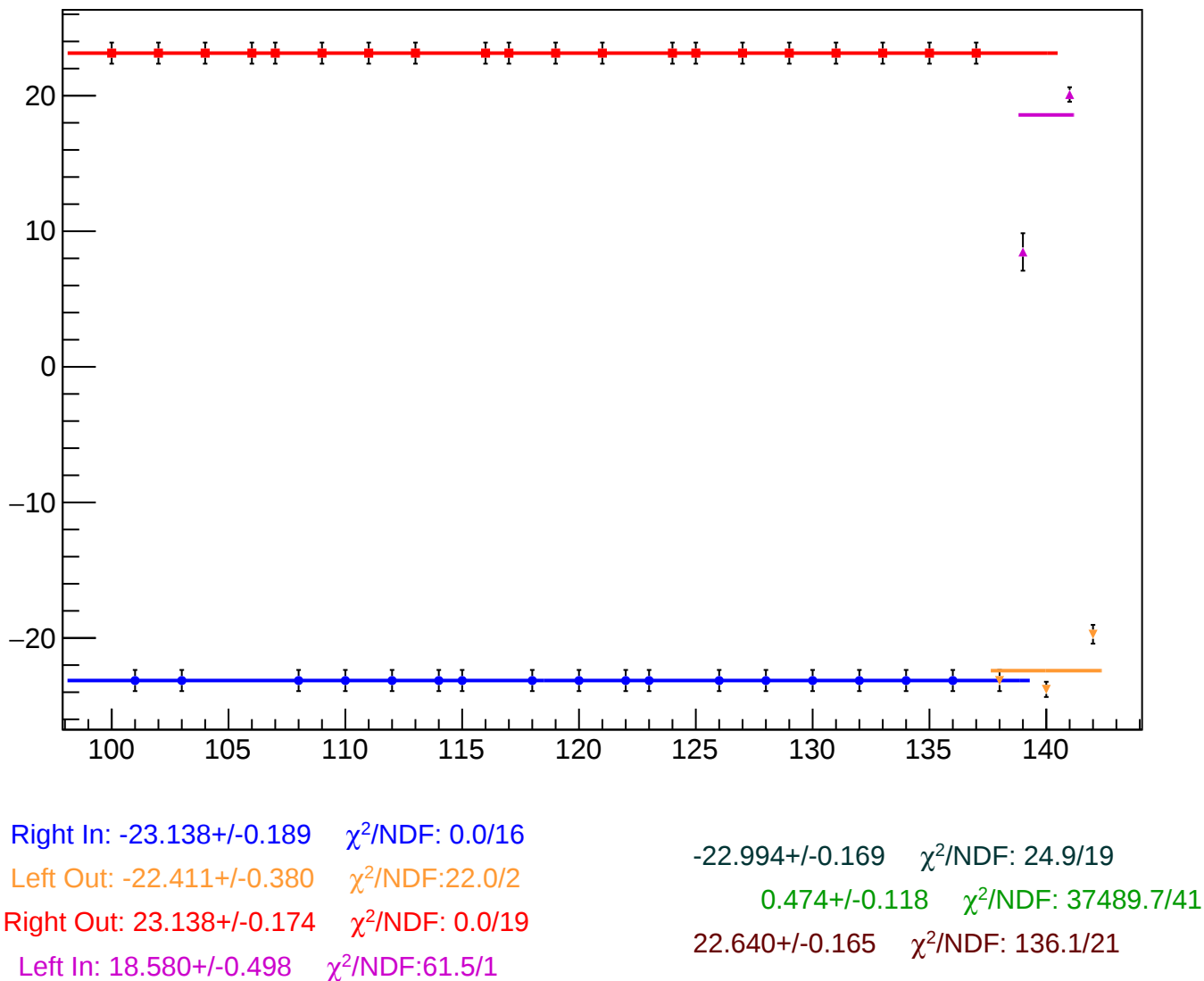
reg_asym_sam_3726_avg_diff_bpm4eY_slope vs Slug, Sign Corrected
