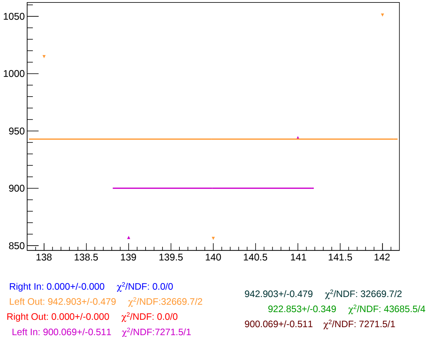
asym_sam5_correction_rms vs Slug, Sign Corrected
