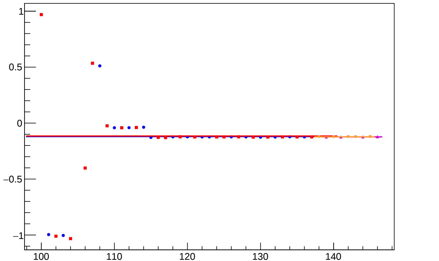
yield_cav4cY_mean vs Slug, Sign Corrected
