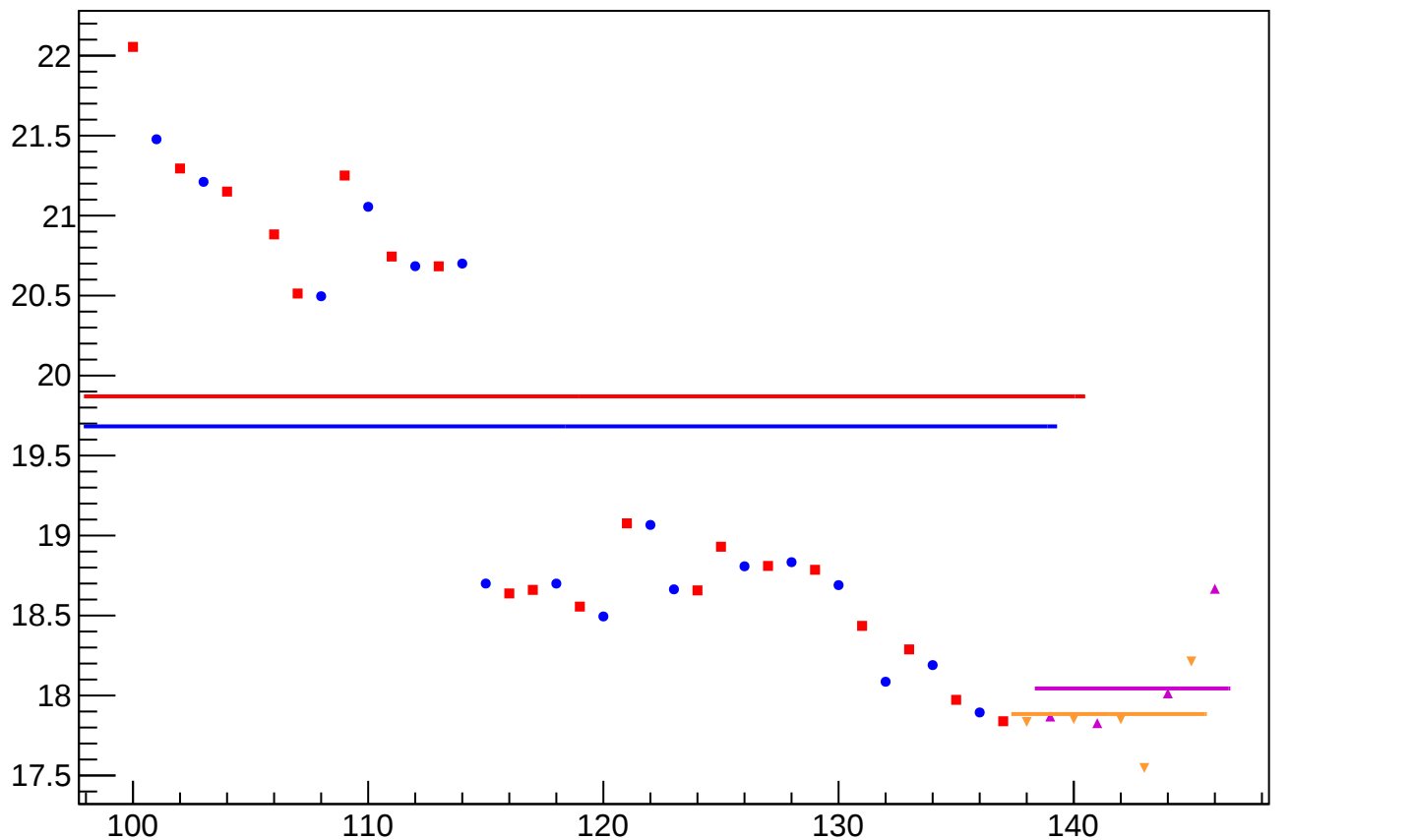
yield_sam5_mean vs Slug, Sign Corrected
