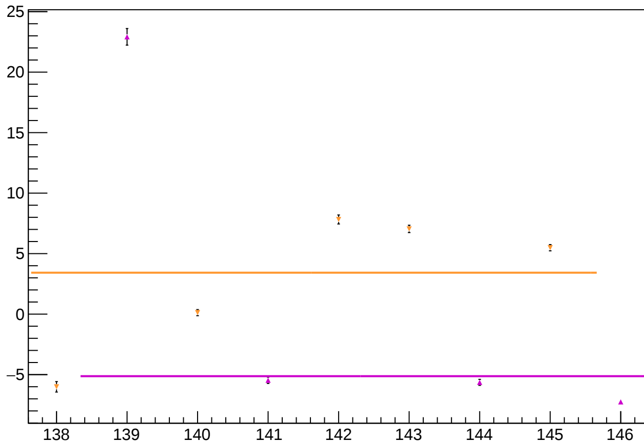
reg_asym_sam_37_48_dd_diff_bpm4aY_slope vs Slug, Sign Corrected
