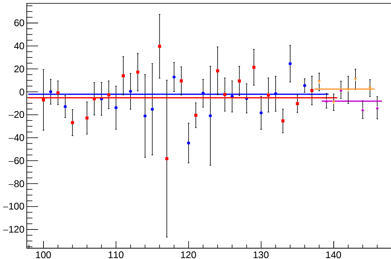
diff_bpm4acY_mean vs Slug, Sign Corrected
