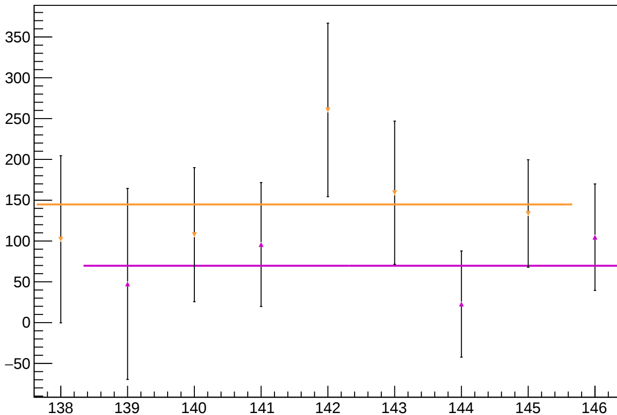
reg_asym_sam_3726_avg_mean vs Slug, Sign Corrected
