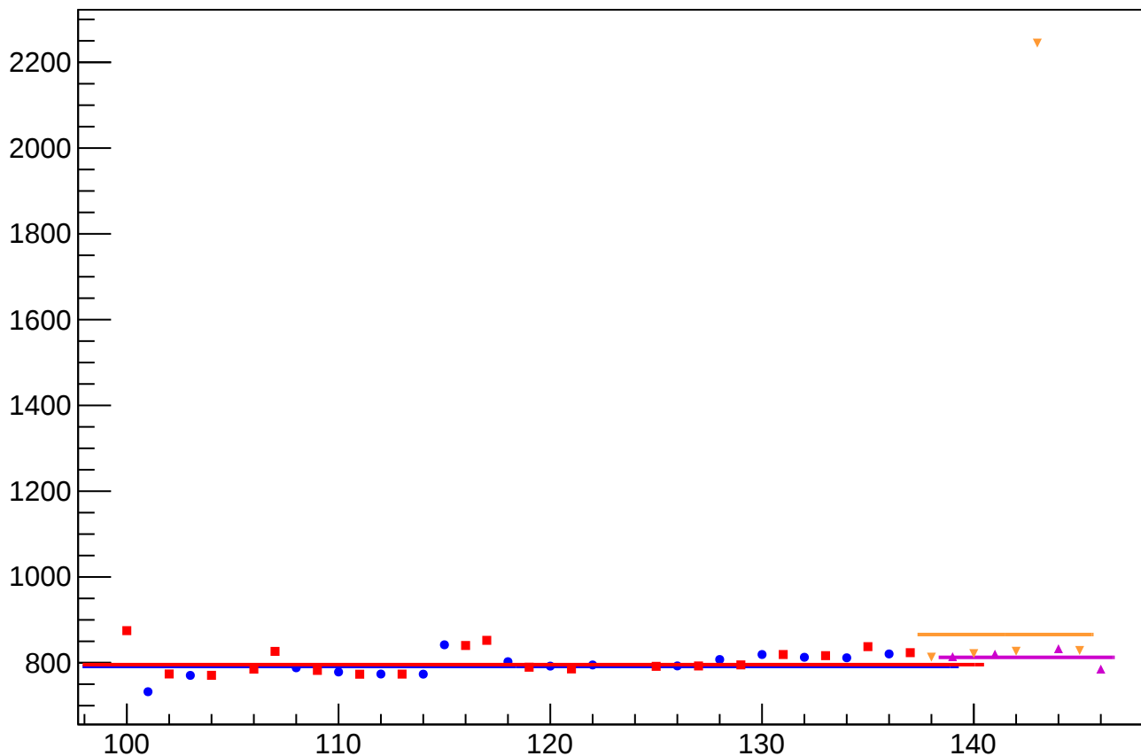
reg_asym_us_avg_rms vs Slug, Sign Corrected
