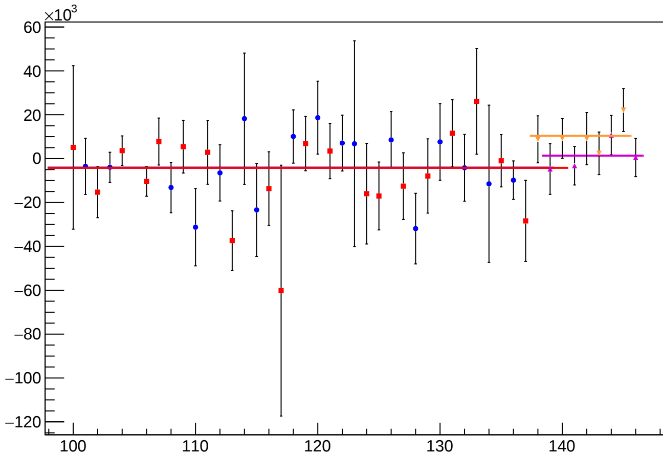
asym_atr2_correction_mean vs Slug, Sign Corrected
