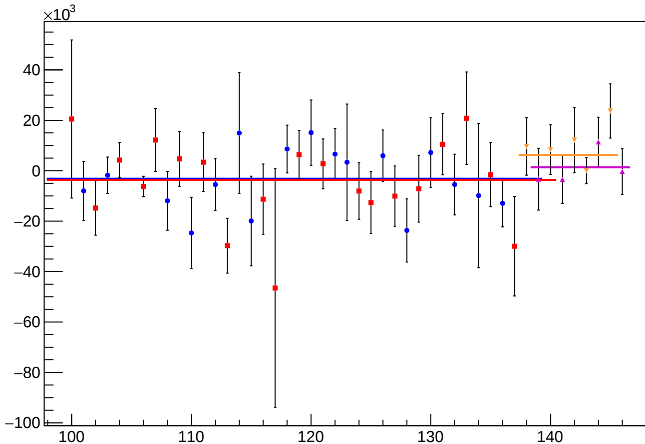
asym_at2_avg_correction_mean vs Slug, Sign Corrected
