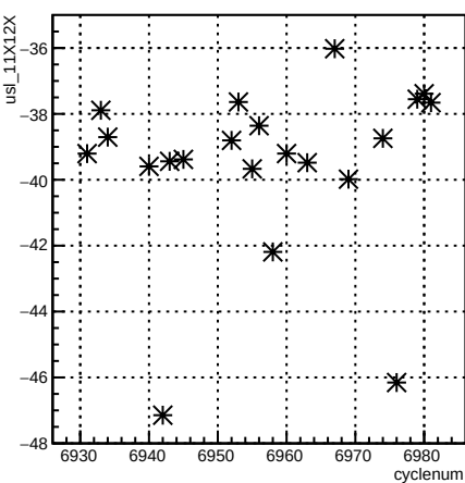
usl_11X12X:cyclenum
