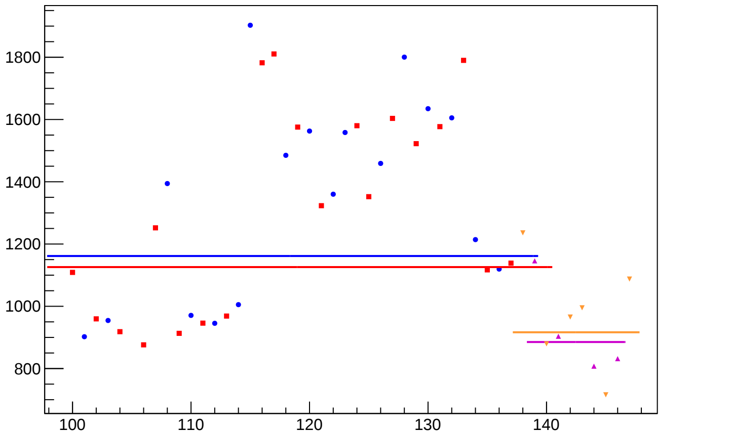
asym_sam_48_dd_correction_rms vs Slug, Sign Corrected
