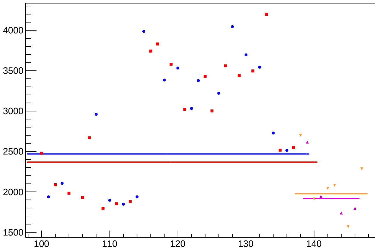
asym_sam4_rms vs Slug, Sign Corrected
