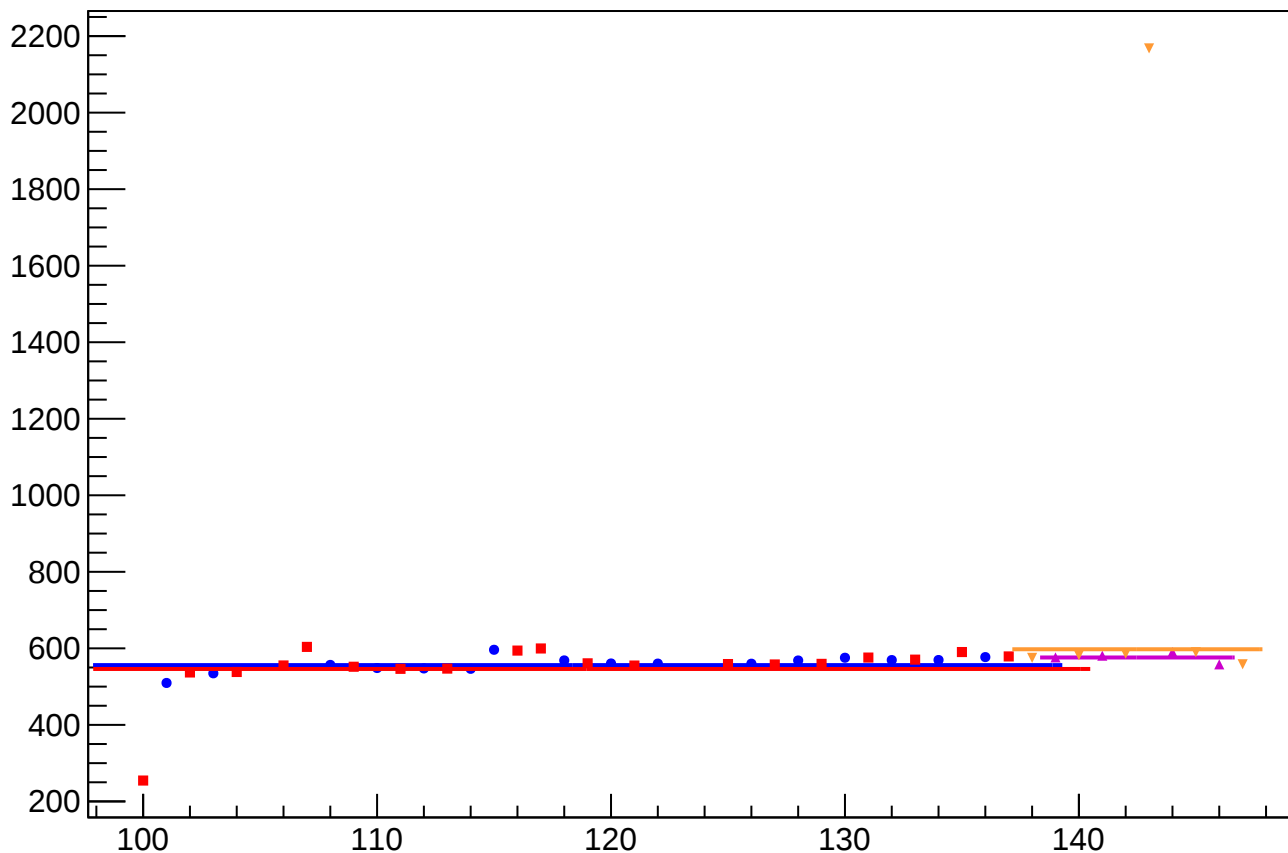
reg_asym_left_dd_rms vs Slug, Sign Corrected
