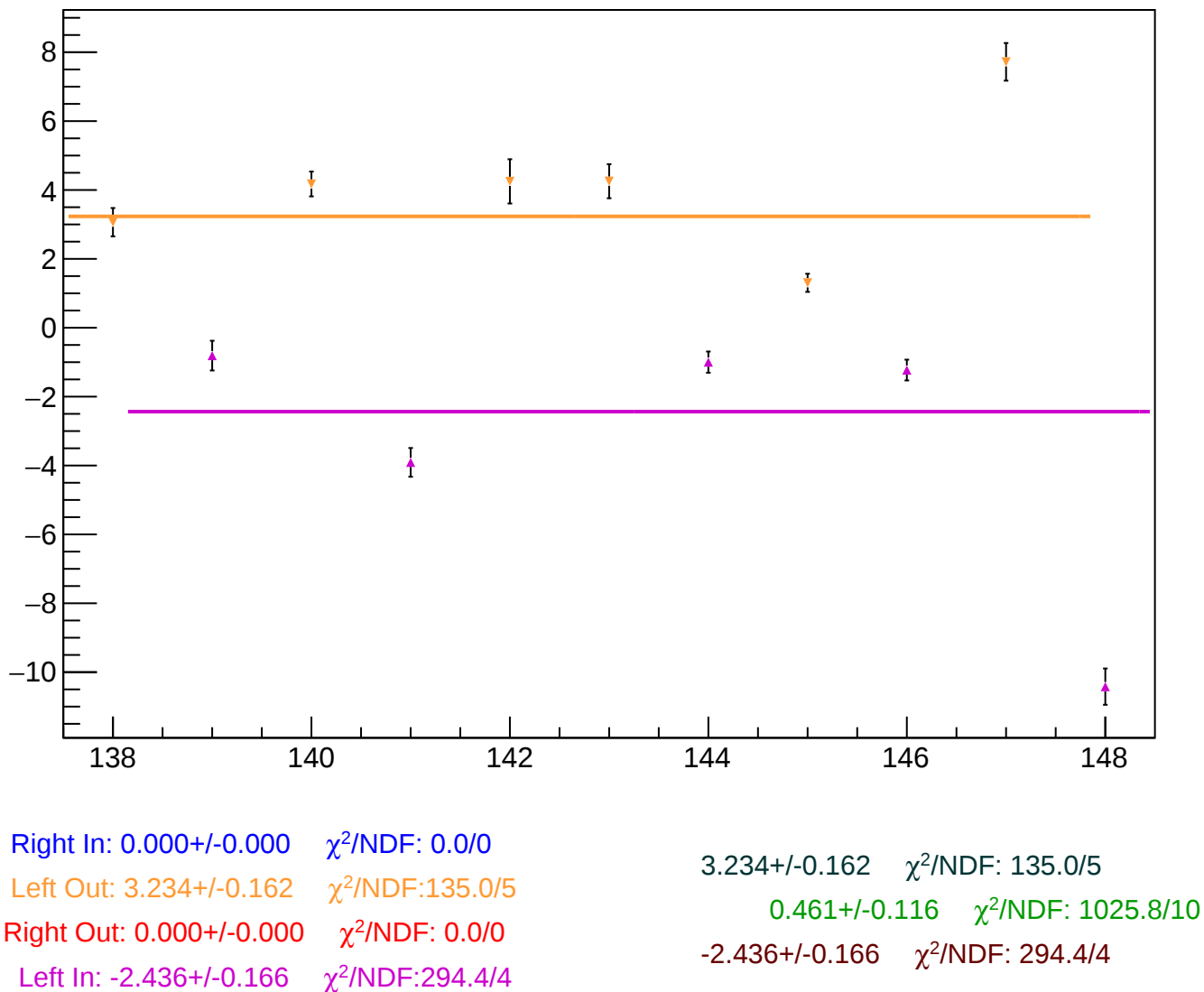
reg_asym_sam_15_26_dd_diff_bpm1X_slope vs Slug, Sign Corrected
