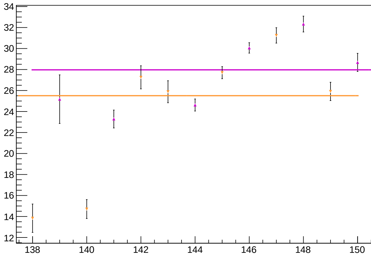
reg_asym_sam3_diff_bpm4eY_slope vs Slug, Sign Corrected
