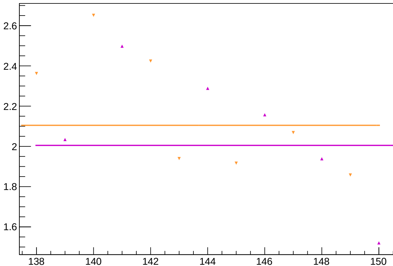
asym_dsr_correction_rms vs Slug, Sign Corrected
