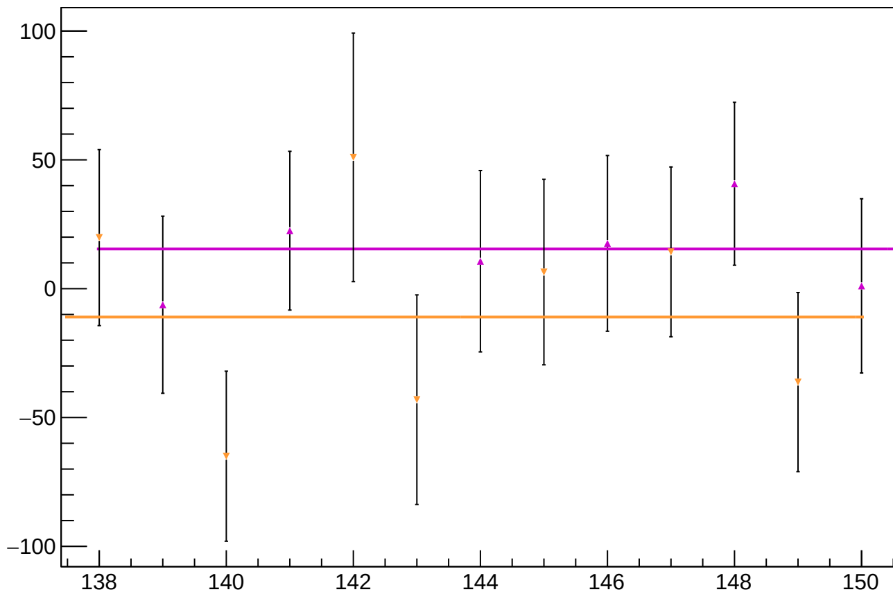
asym_bcm_cav4cQ_bcm_an_ds_agg_dd_mean vs Slug, Sign Corrected
