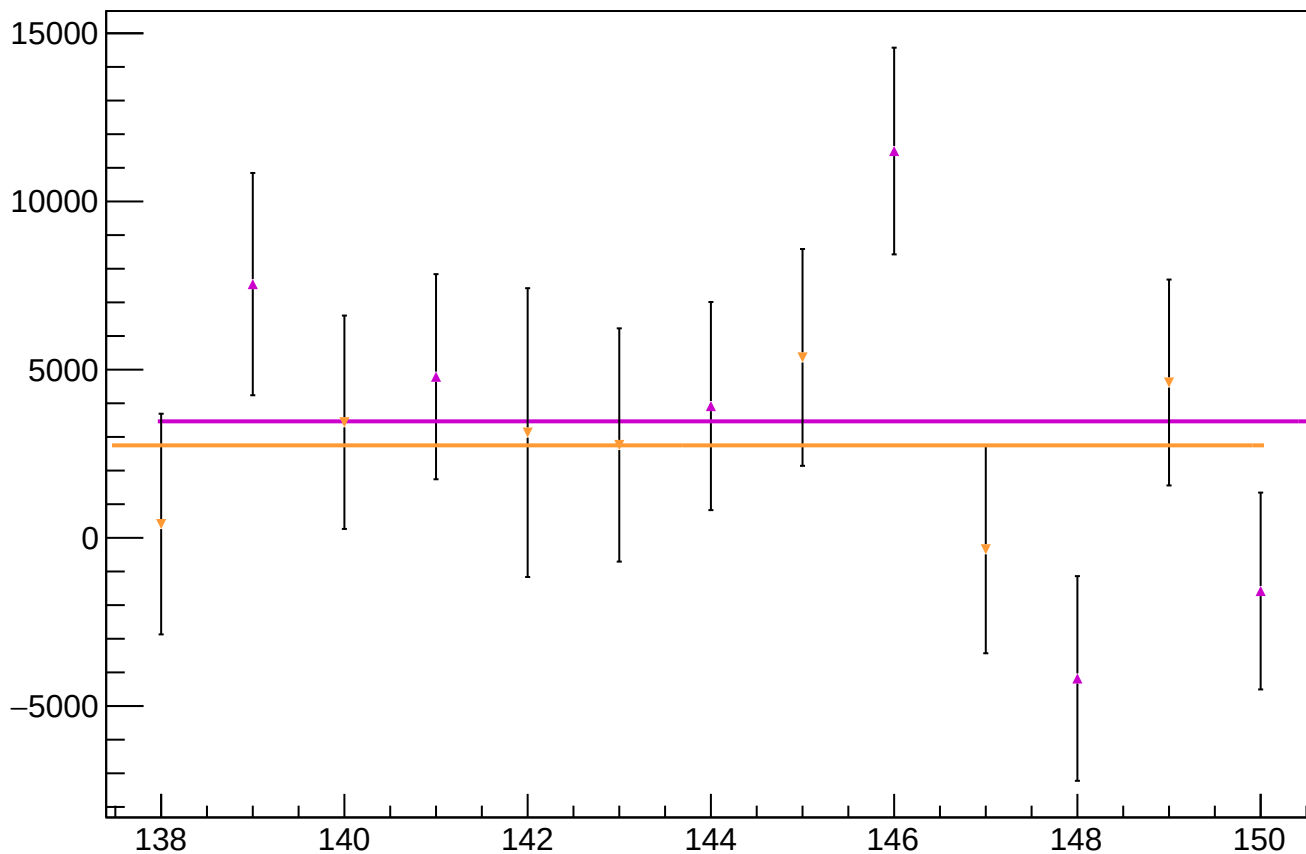
reg_asym_atr1_mean vs Slug, Sign Corrected
