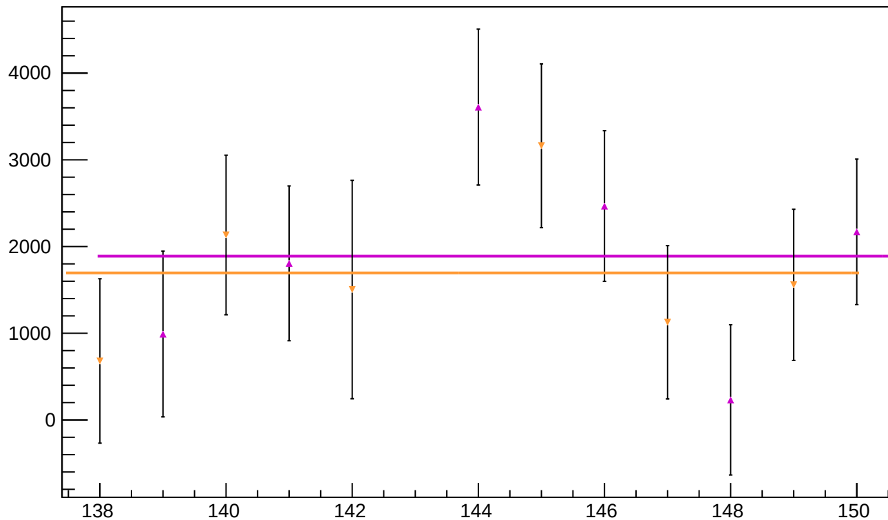
reg_asym_us_avg_mean vs Slug, Sign Corrected
