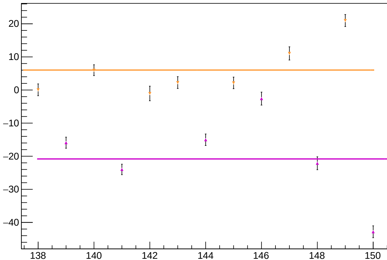
diff_bpm0l01Y_mean vs Slug, Sign Corrected
