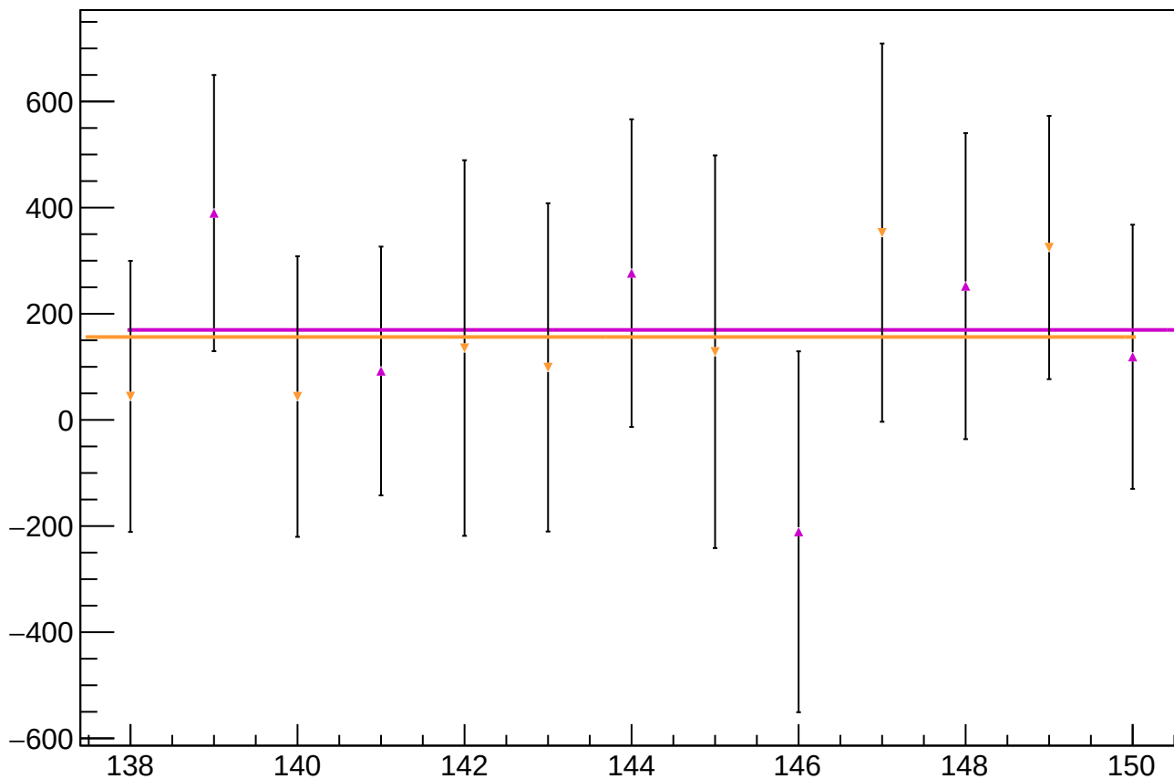
asym_bcm_an_ds_mean vs Slug, Sign Corrected
