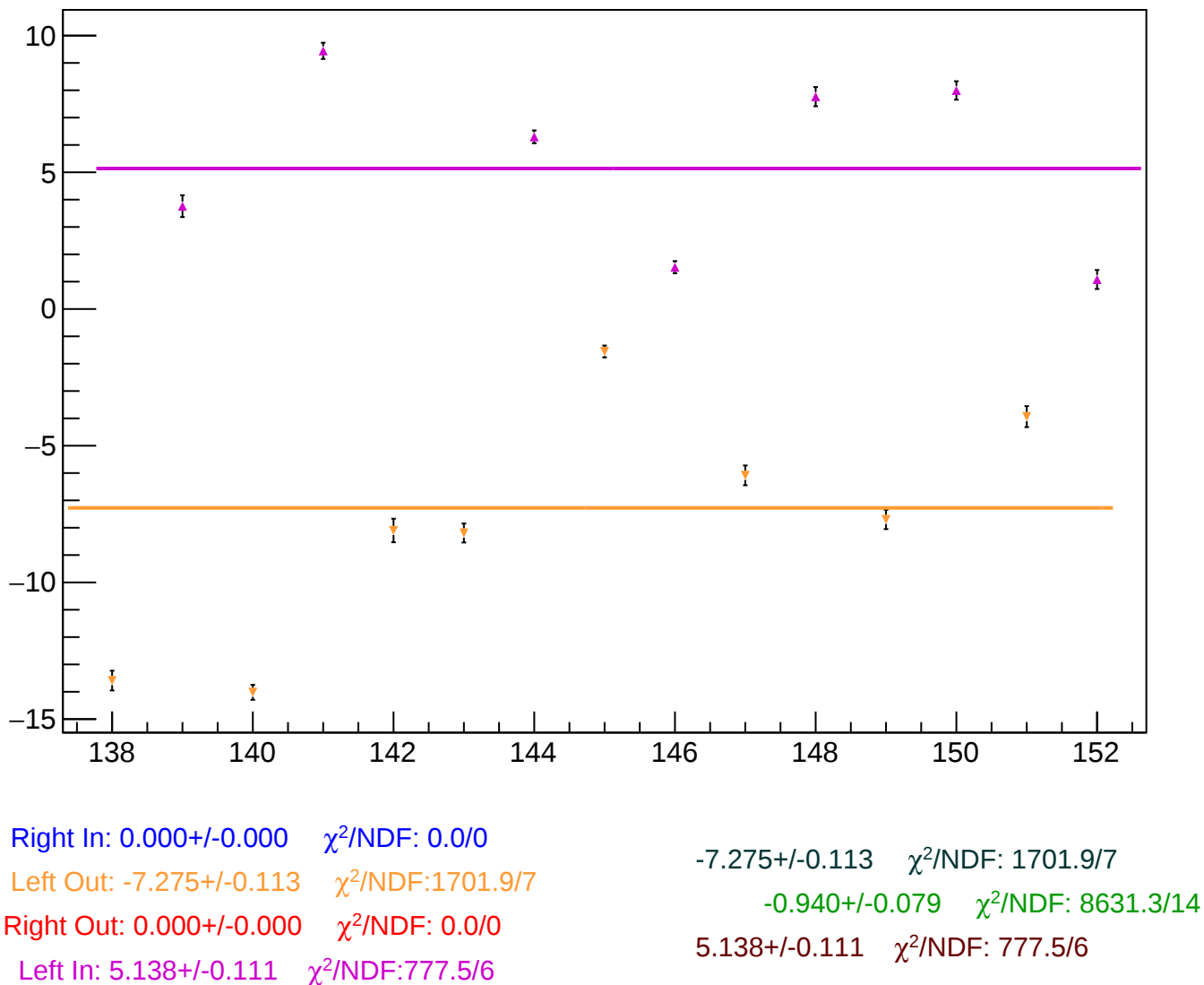
reg_asym_sam_1526_avg_diff_bpm1X_slope vs Slug, Sign Corrected
