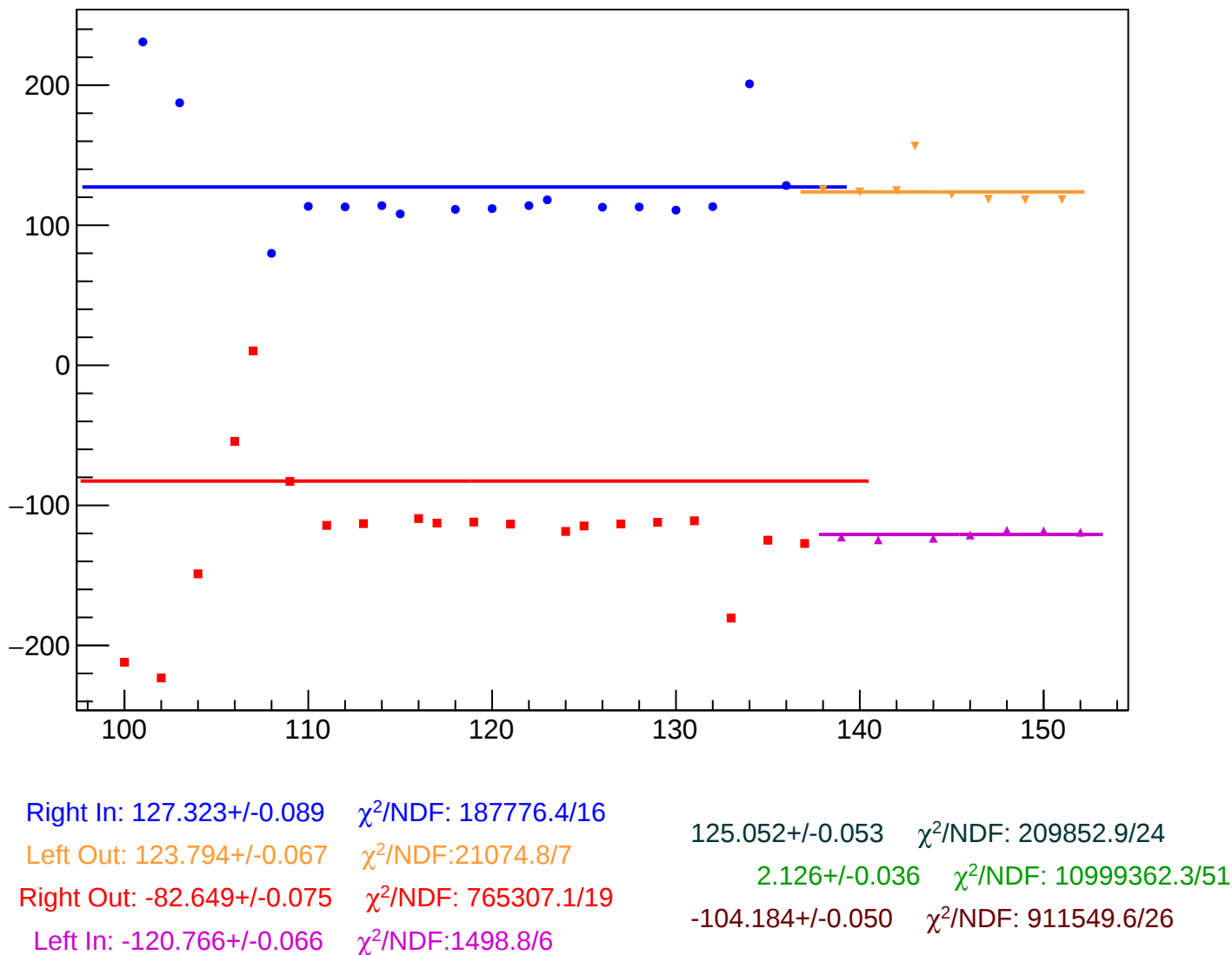
reg_asym_atl1r2_dd_diff_bpm12X_slope vs Slug, Sign Corrected
