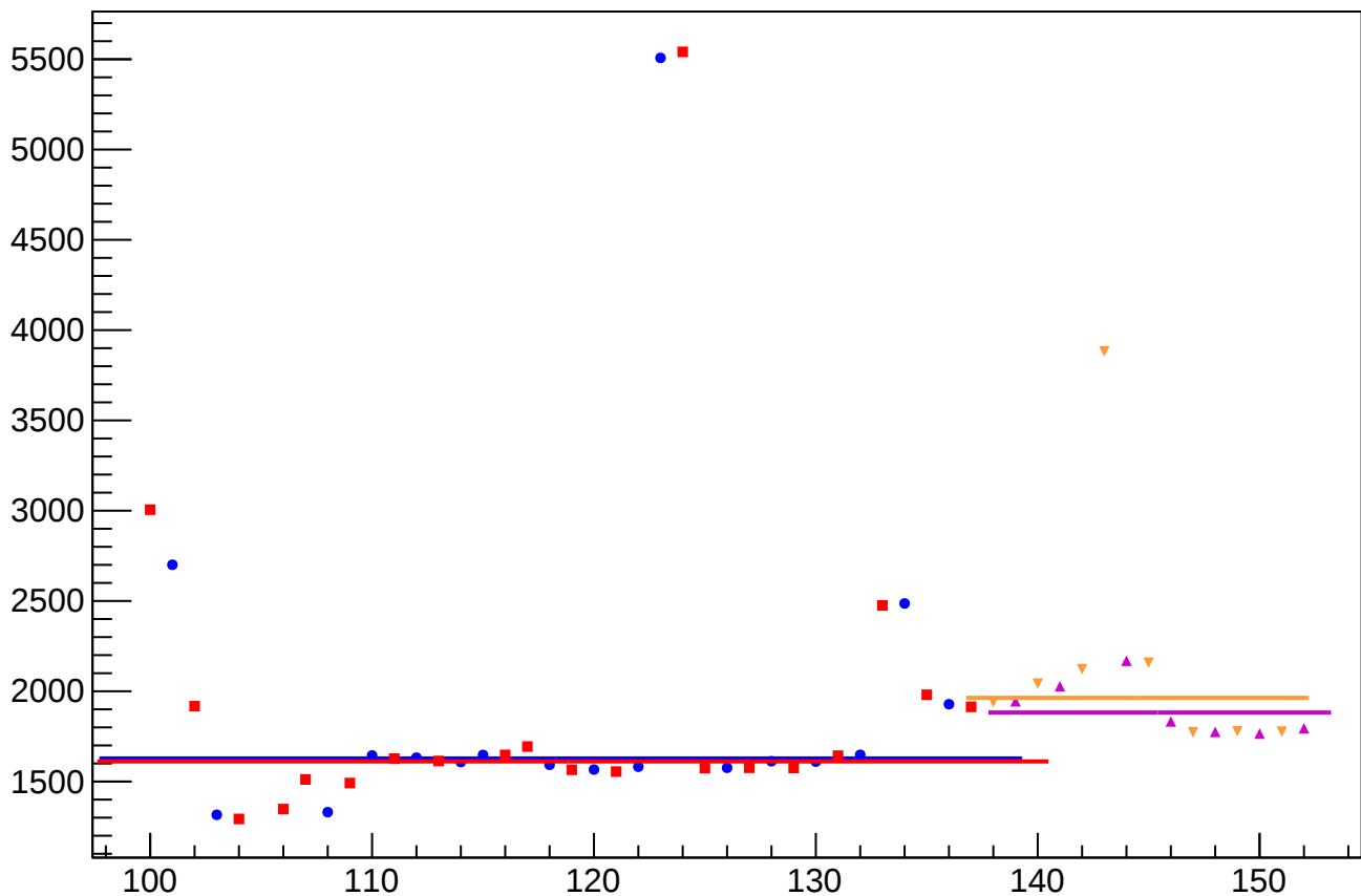
reg_asym_at2_dd_rms vs Slug, Sign Corrected
