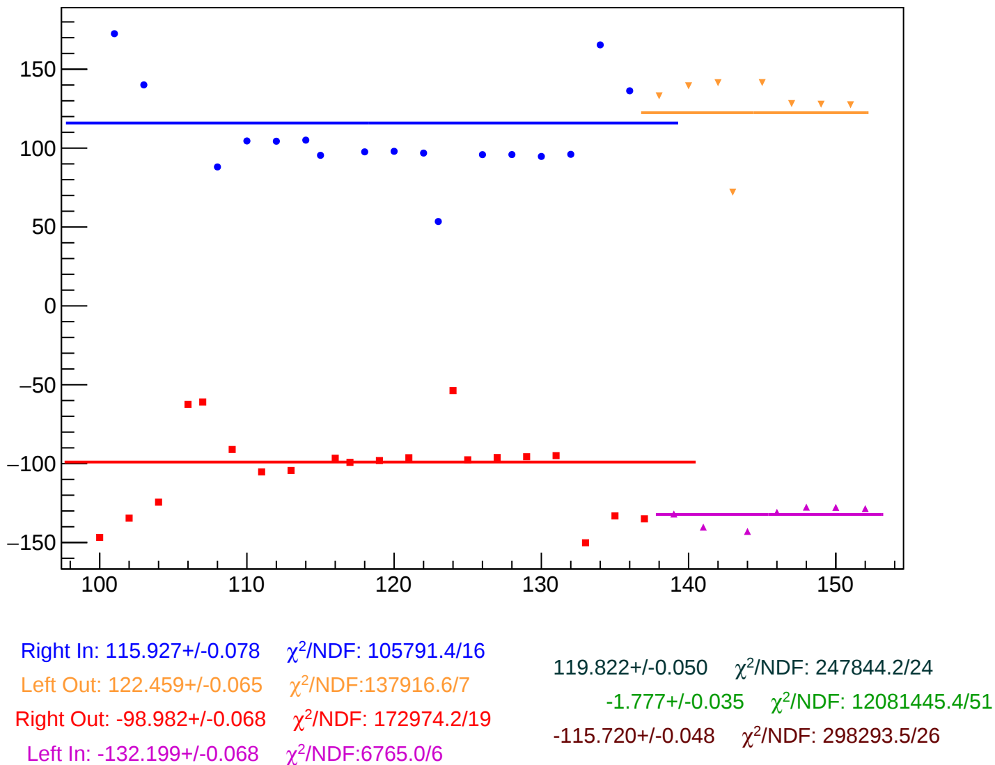
reg_asym_atl_dd_atr_dd_avg_diff_bpm12X_slope vs Slug, Sign Corrected
