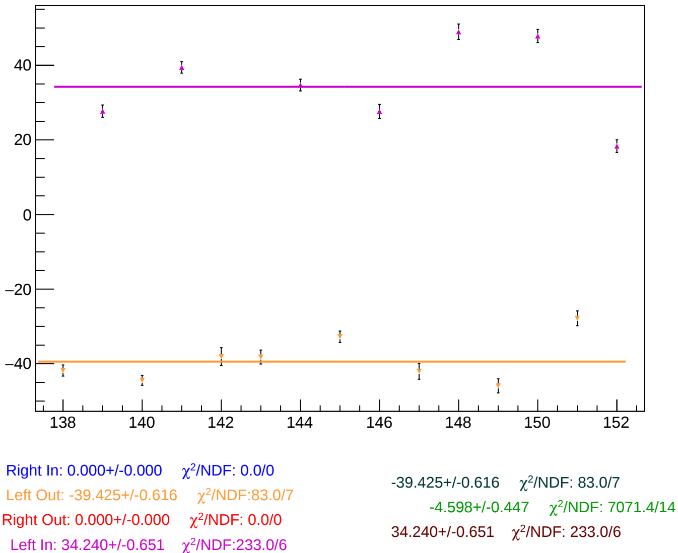
reg_asym_sam_26_dd_diff_bpm1X_slope vs Slug, Sign Corrected
