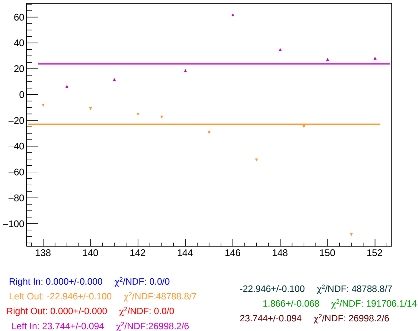
reg_asym_bcm_an_ds_diff_bpm1X_slope vs Slug, Sign Corrected
