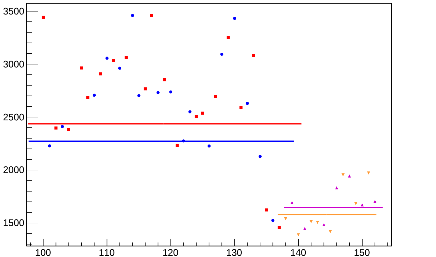
asym_sam_26_dd_correction_rms vs Slug, Sign Corrected
