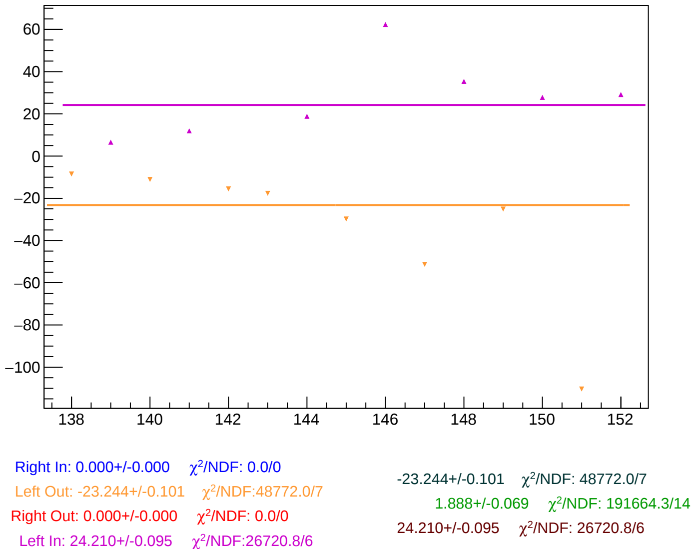
reg_asym_bcm_dg_ds_diff_bpm1X_slope vs Slug, Sign Corrected
