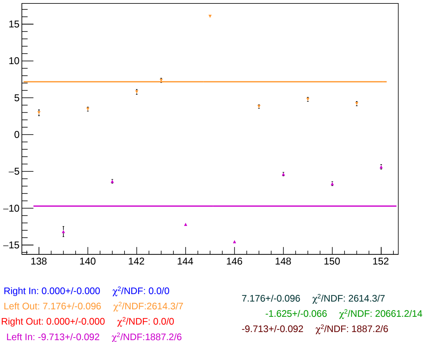
reg_asym_sam_1526_avg_diff_bpm4eY_slope vs Slug, Sign Corrected
