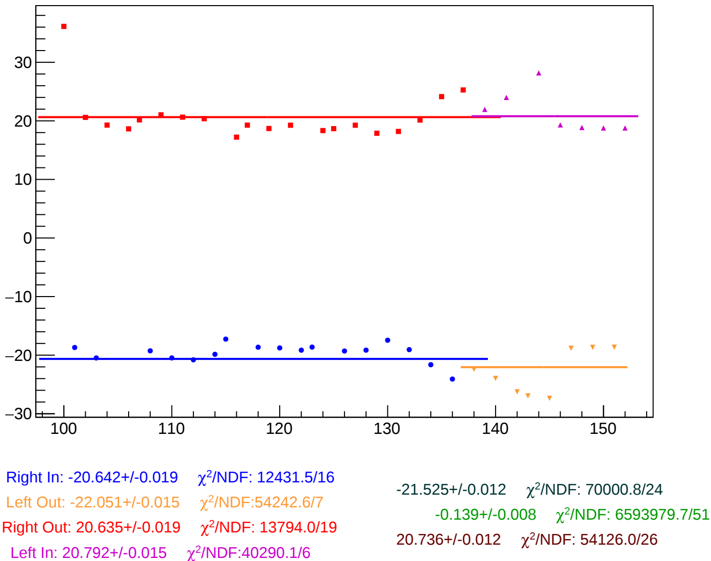
reg_asym_right_avg_diff_bpm12X_slope vs Slug, Sign Corrected
