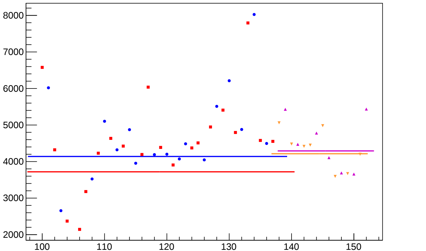
asym_atr_avg_correction_rms vs Slug, Sign Corrected
