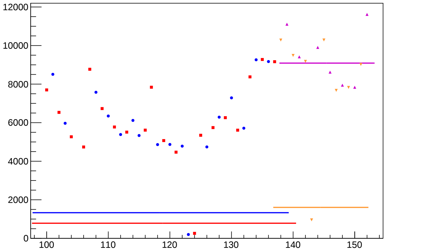
asym_atl2_correction_rms vs Slug, Sign Corrected
