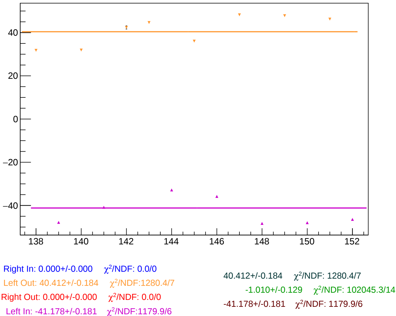
reg_asym_sam_15_48_dd_diff_bpm4eX_slope vs Slug, Sign Corrected
