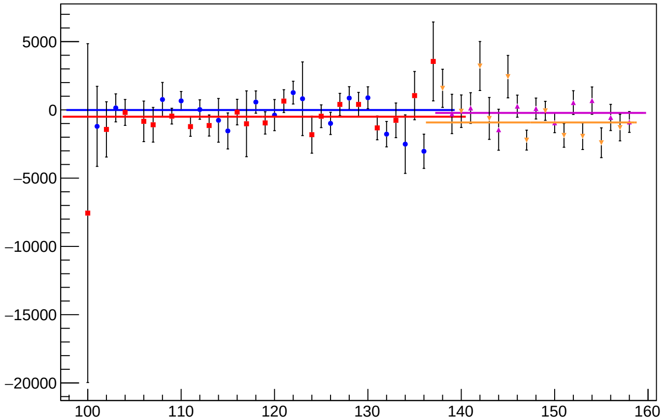
asym_atr1_correction_mean vs Slug
