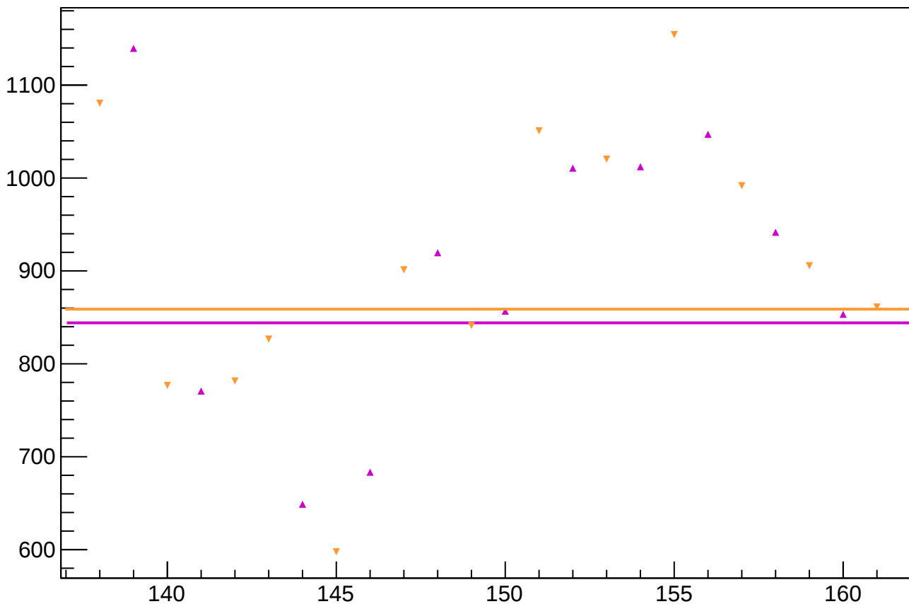
asym_sam_3748_avg_correction_rms vs Slug
