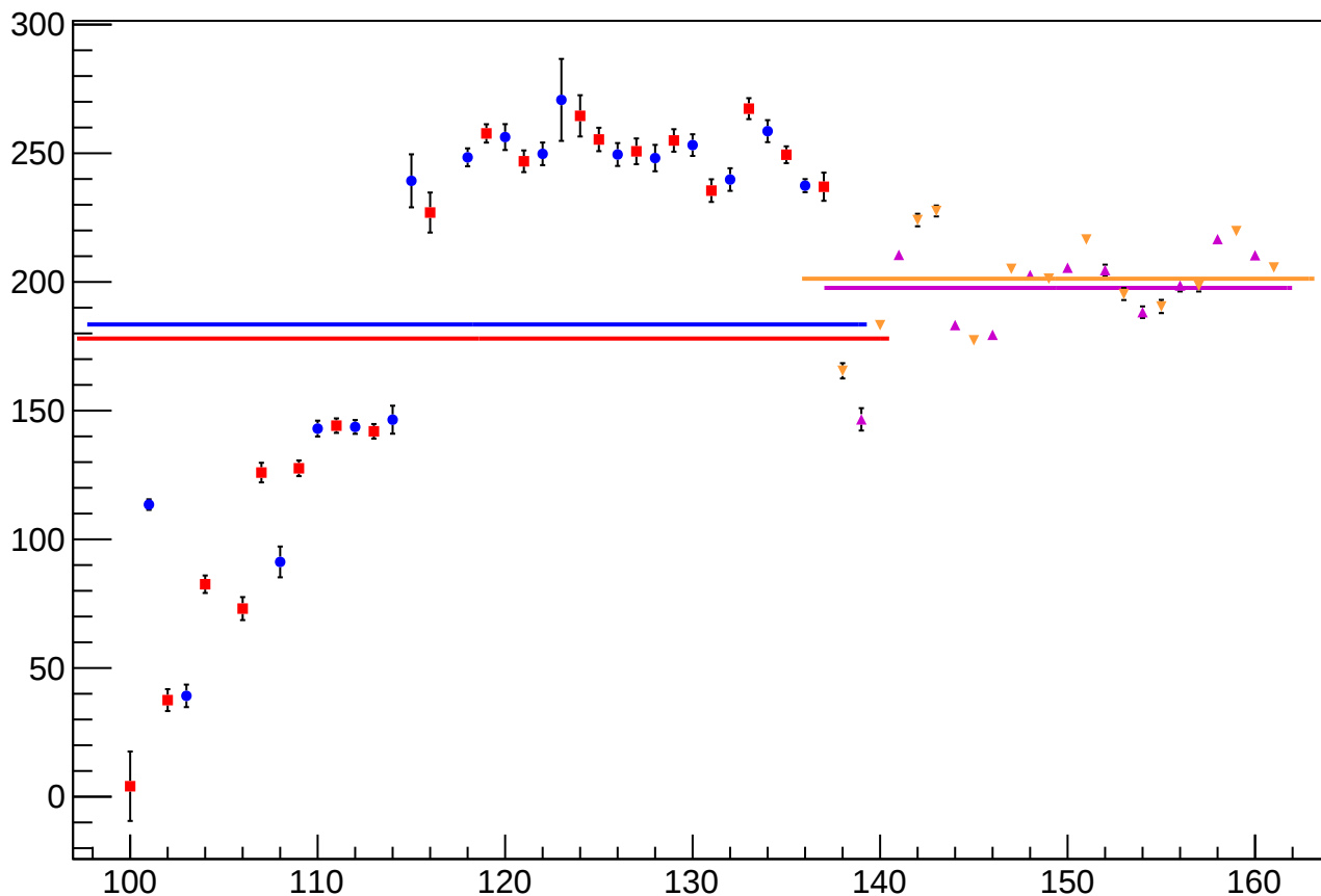
reg_asym_sam4_diff_bpm4eY_slope vs Slug
