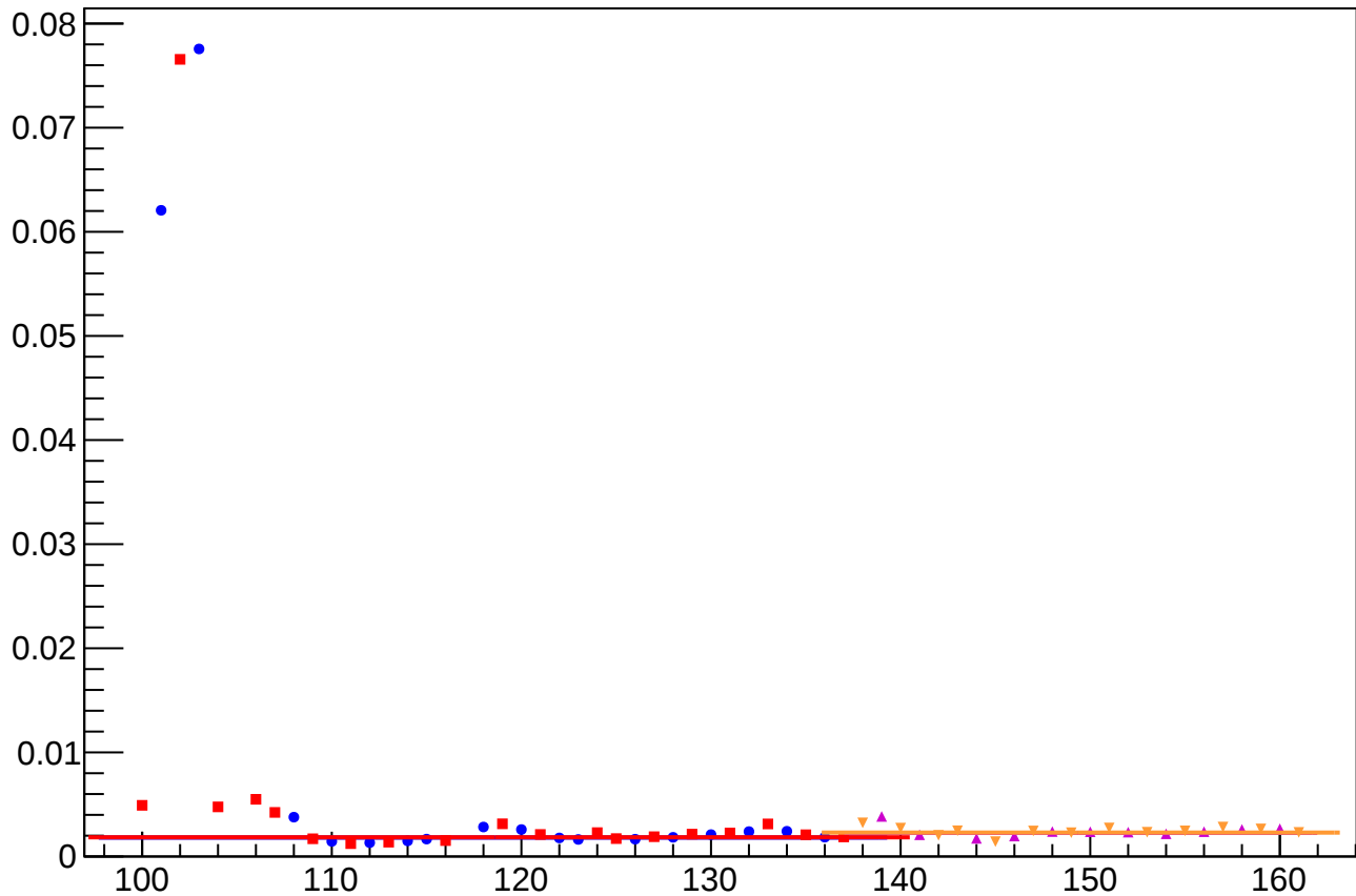
yield_sam7_rms vs Slug
