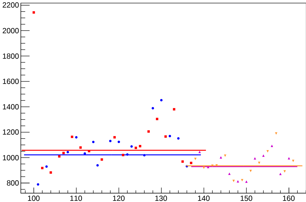
asym_right_avg_rms vs Slug
