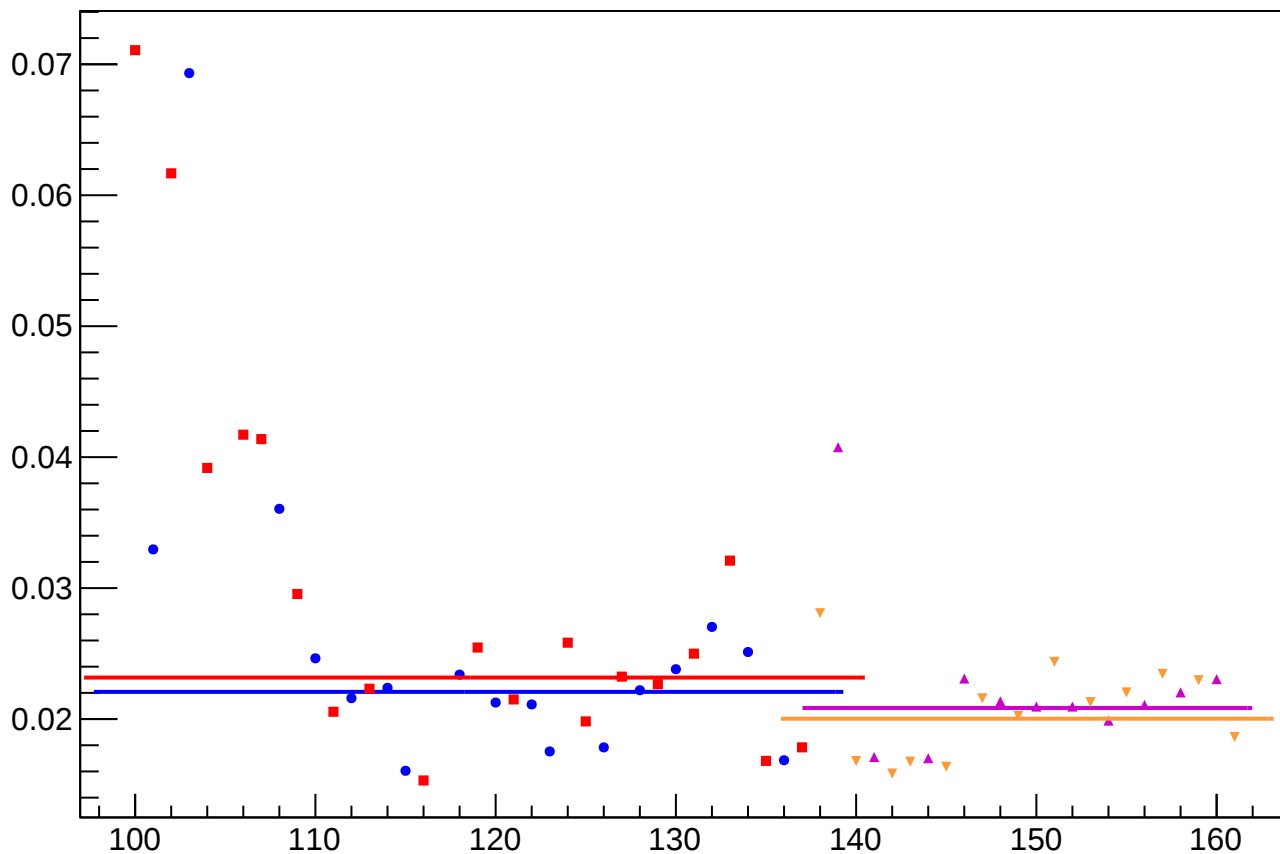
yield_bpm4aX_rms vs Slug
