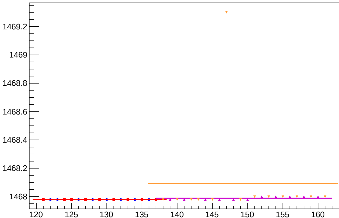
psub_pl_pos_mean vs Slug
