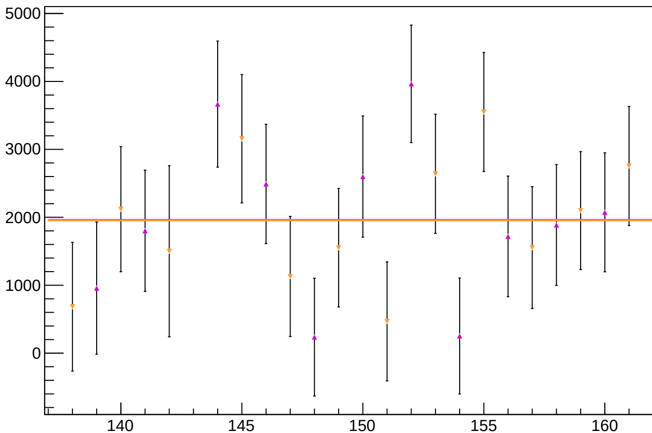
cor_asym_us_avg_mean vs Slug, Sign Corrected
