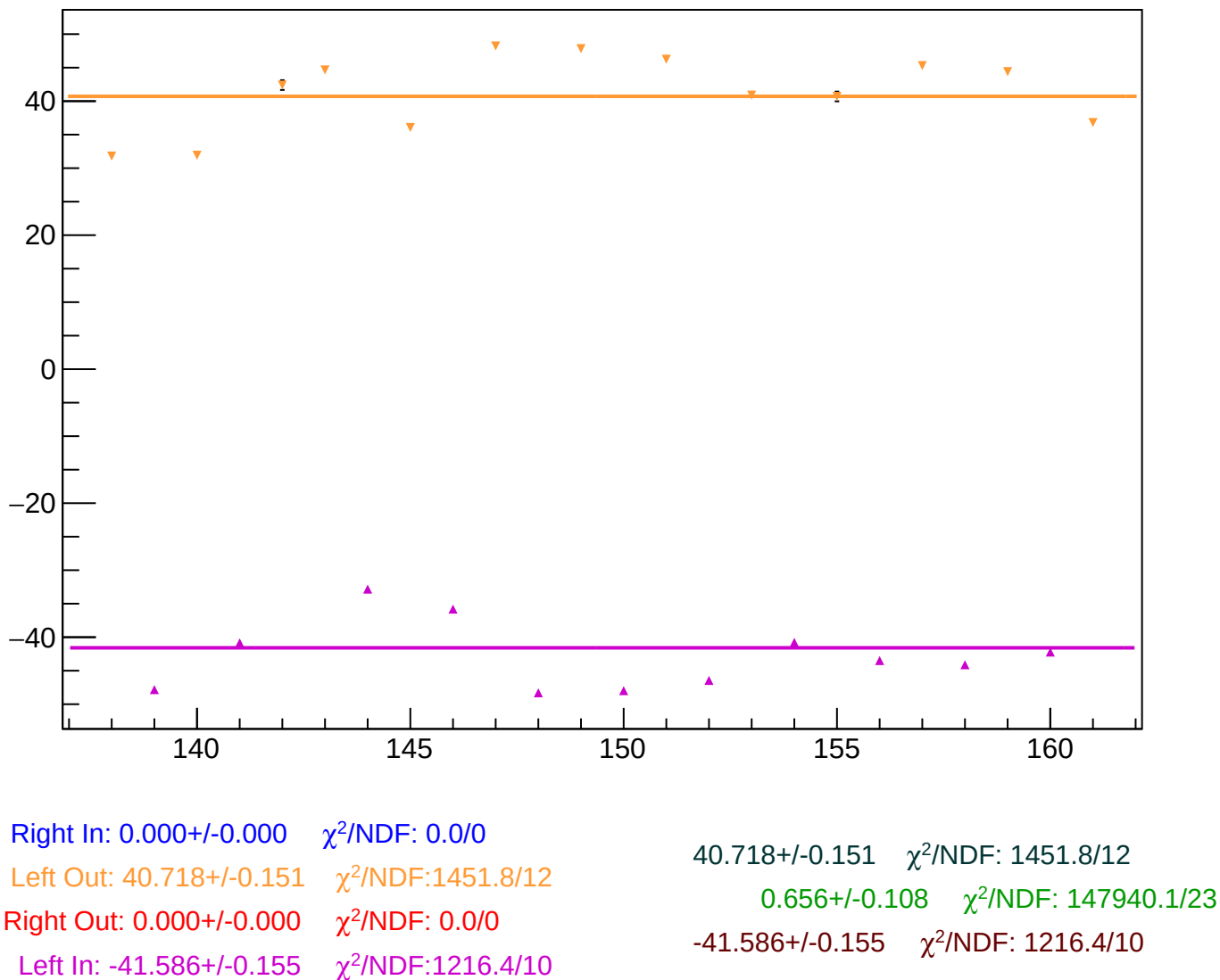
reg_asym_sam_15_48_dd_diff_bpm4eX_slope vs Slug, Sign Corrected
