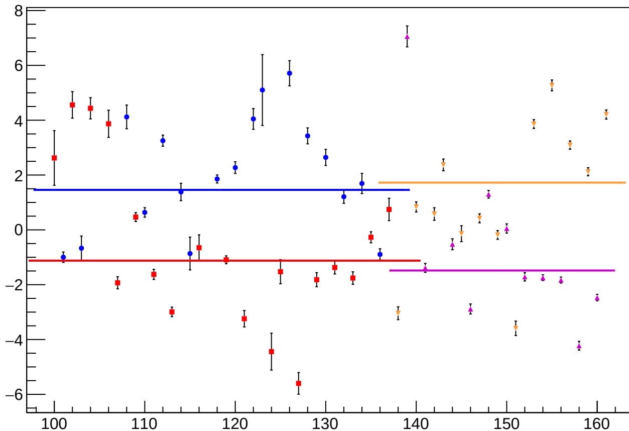
reg_asym_bcm_an_ds3_diff_bpm4aY_slope vs Slug, Sign Corrected
