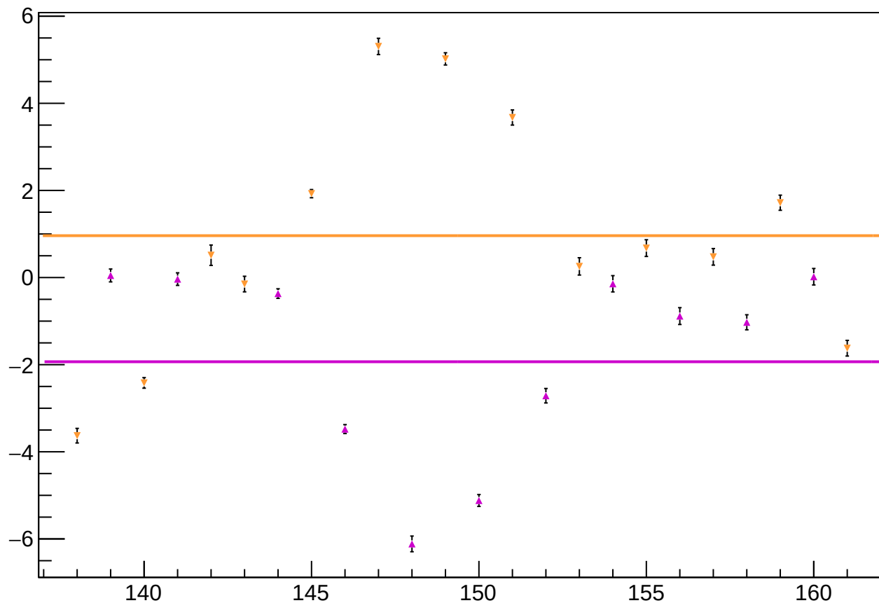
reg_asym_sam_37_26_dd_diff_bpm1X_slope vs Slug, Sign Corrected
