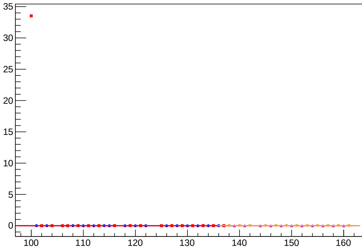
reg_asym_ds_avg_diff_bpm12X_slope vs Slug, Sign Corrected
