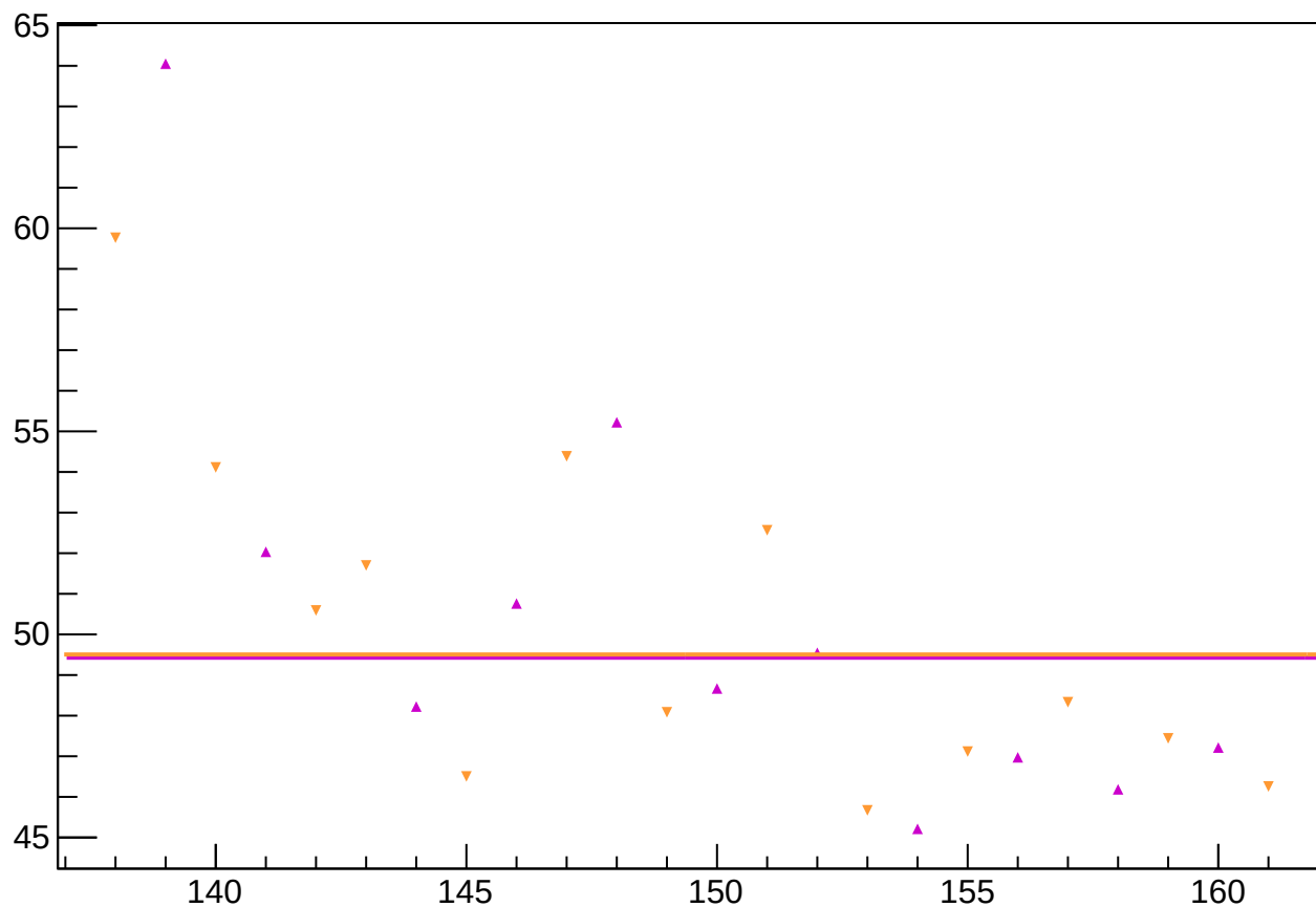
reg_asym_sam_1526_avg_rms vs Slug, Sign Corrected
