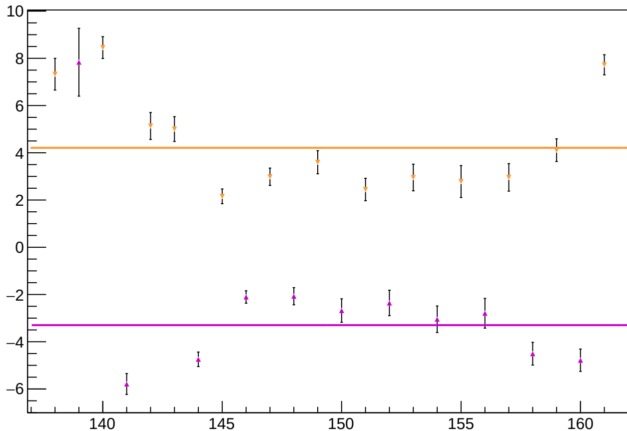
reg_asym_sam_3726_avg_diff_bpm4aY_slope vs Slug, Sign Corrected
