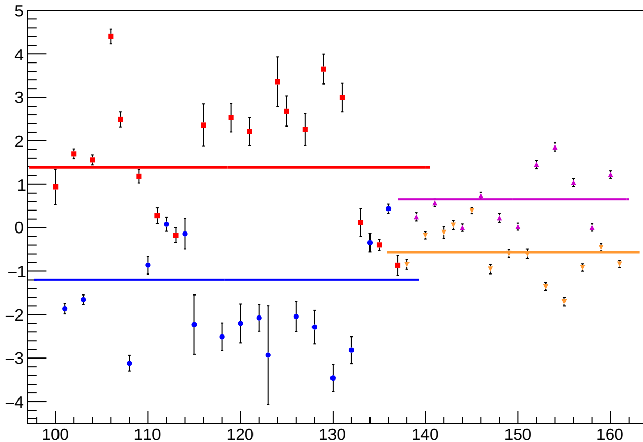
reg_asym_sam4_diff_bpm12X_slope vs Slug, Sign Corrected
