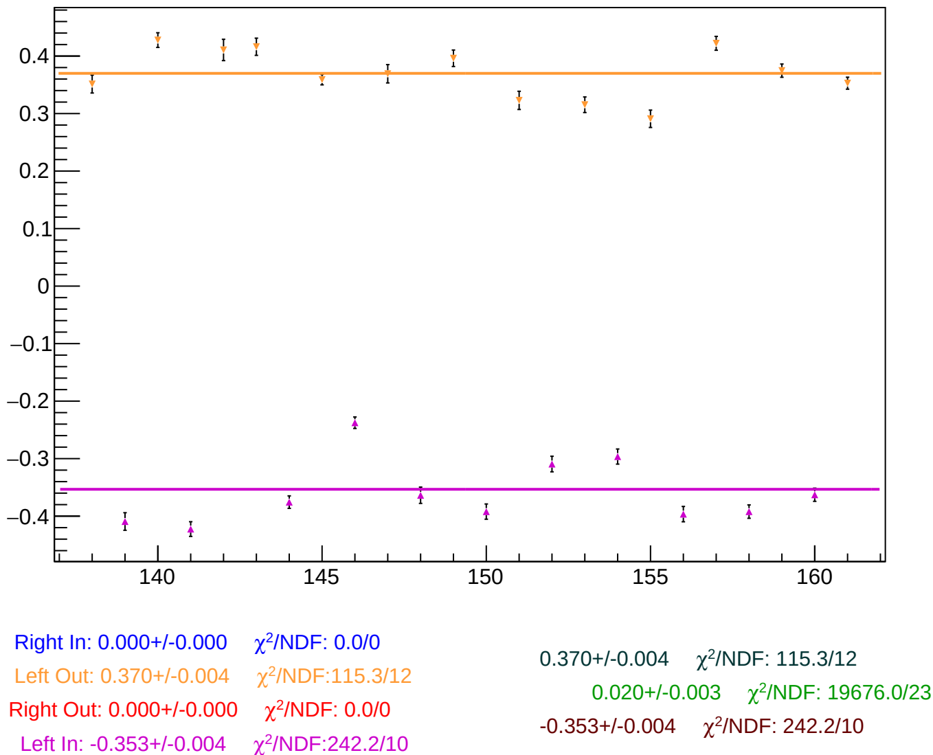
reg_asym_sam_1526_avg_diff_bpm12X_slope vs Slug, Sign Corrected
