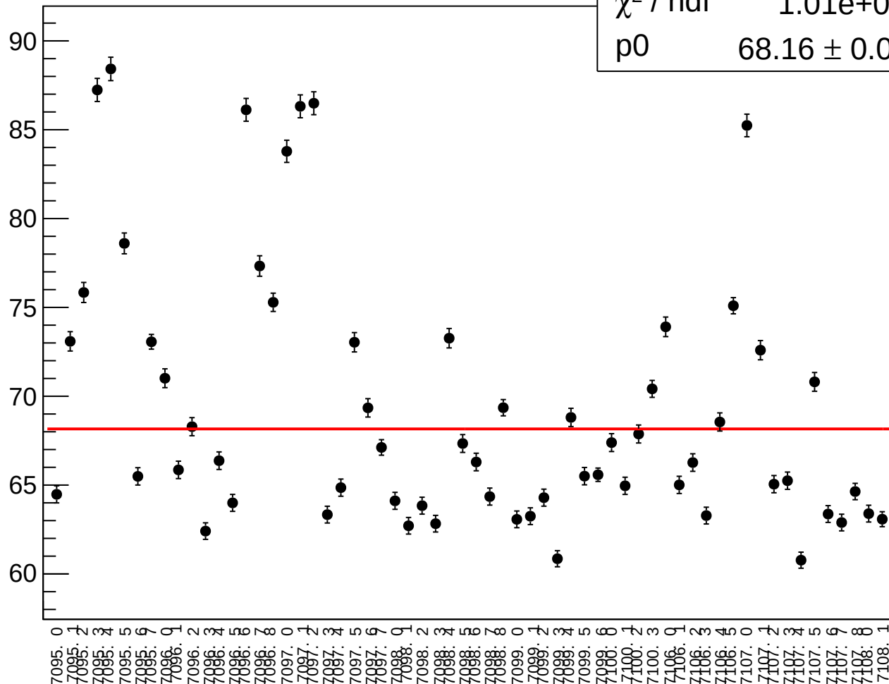
reg_asym_sam_37_avg_rms vs run
