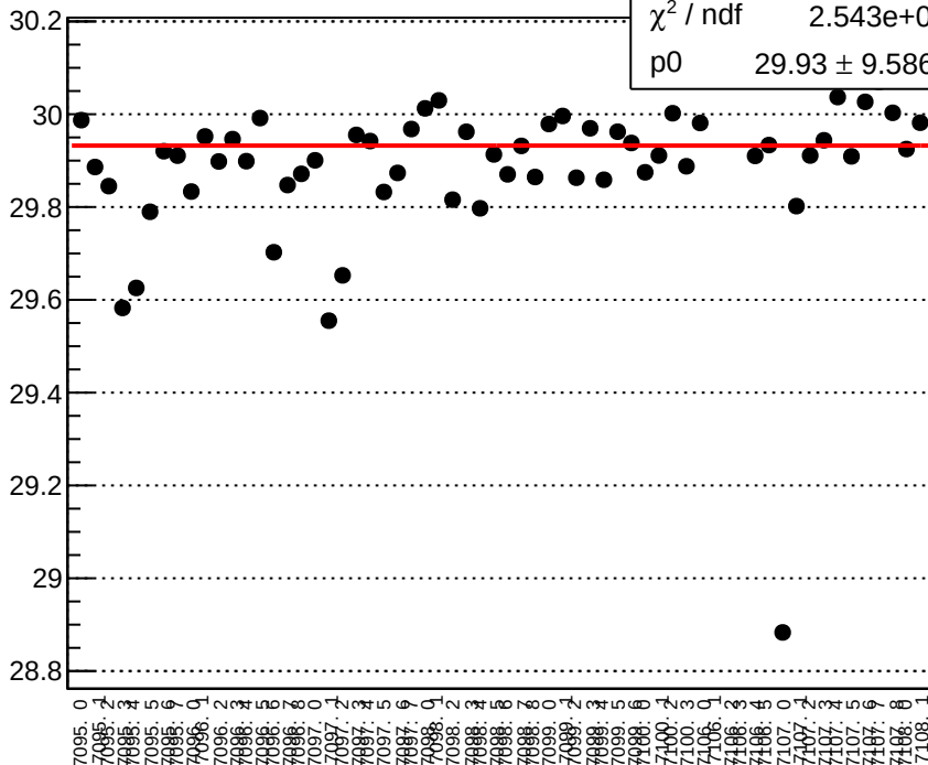
yield_sam3_mean vs run
