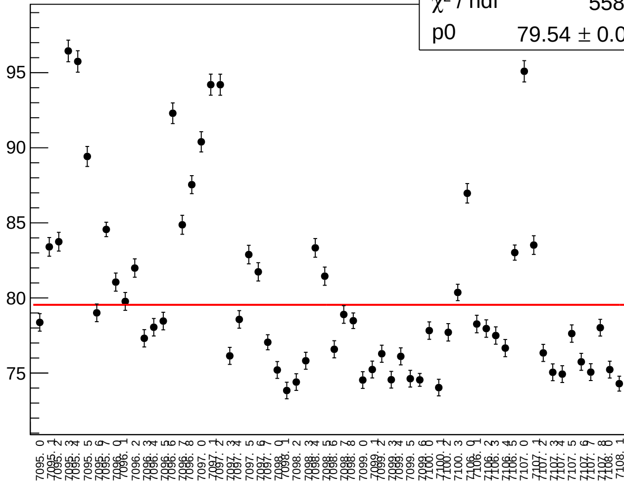
reg_asym_sam_24_68_dd_rms vs run
