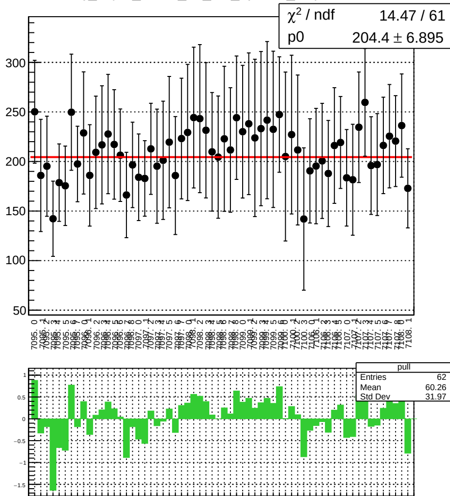
reg_asym_atr1l2_dd_diff_bpm1X_slope vs run
