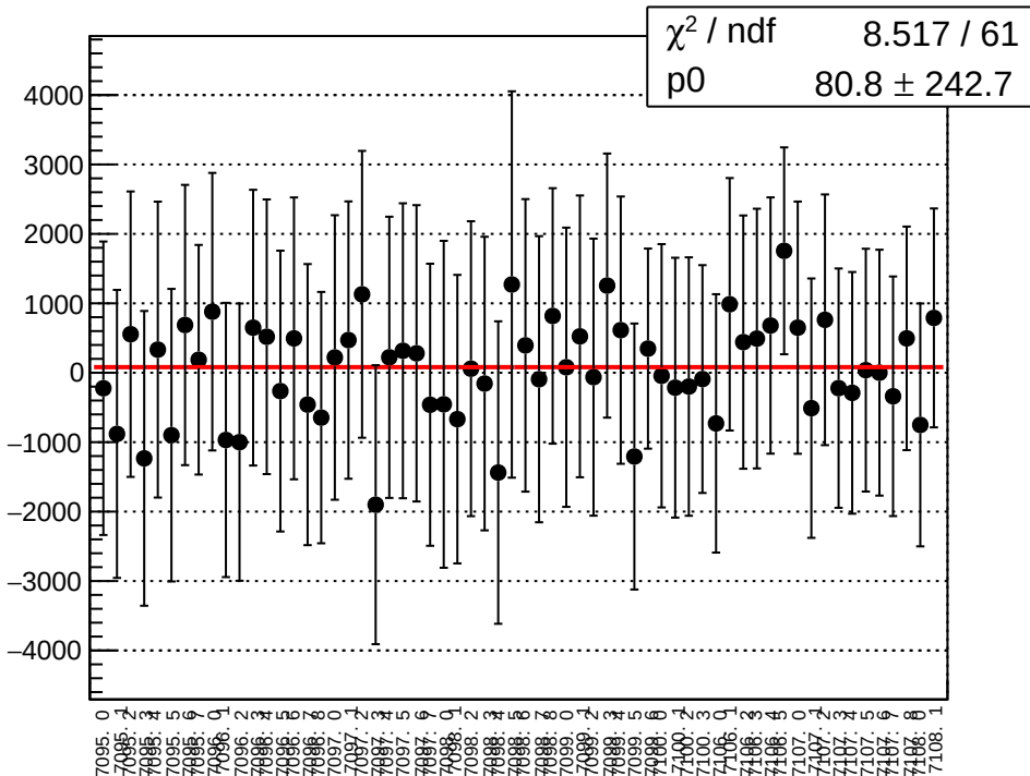
asym bcm an us bcm an ds agg avg mean vs run
