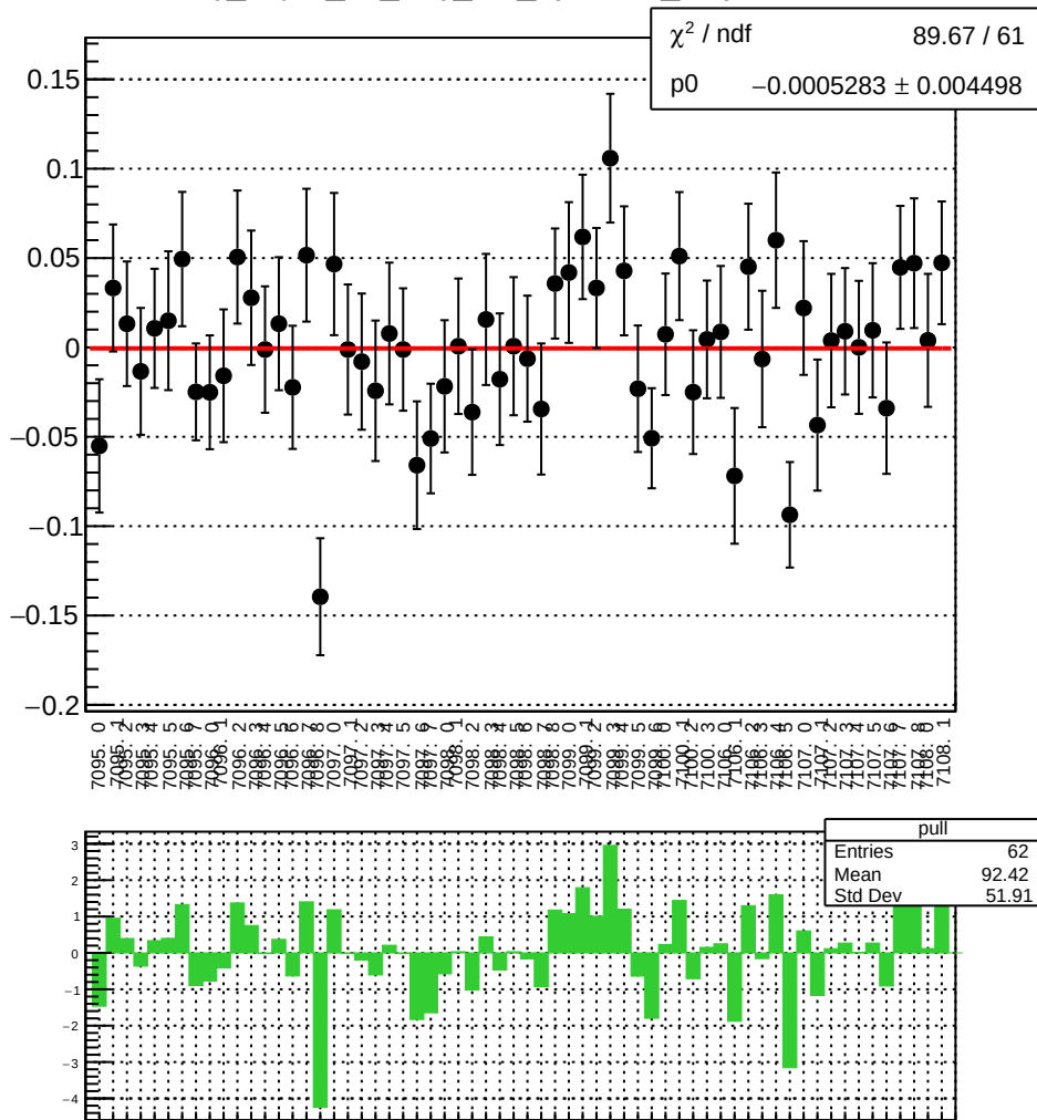
reg_asym_ds_avg_diff_bpm12X_slope vs run
