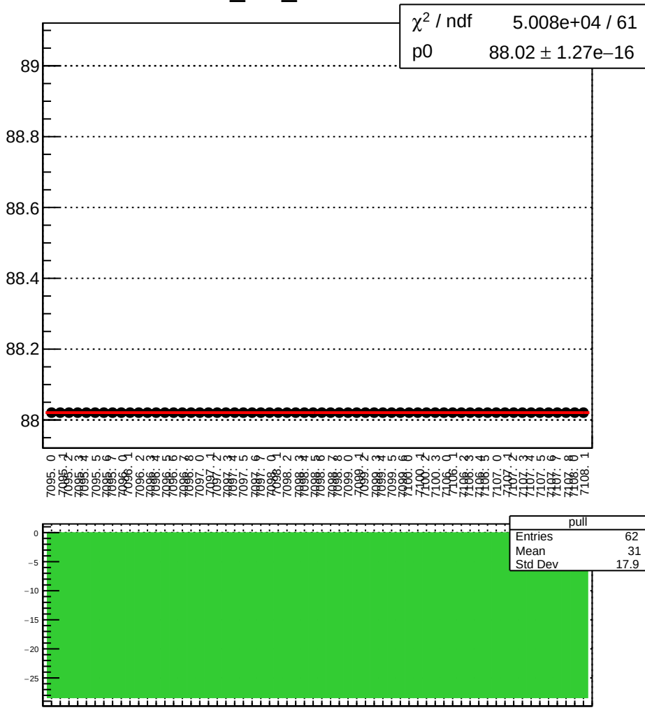
Phi_FG_mean vs run
