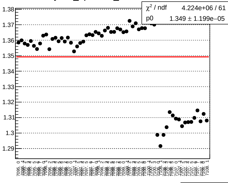
yield_bpm12Y_mean vs run
