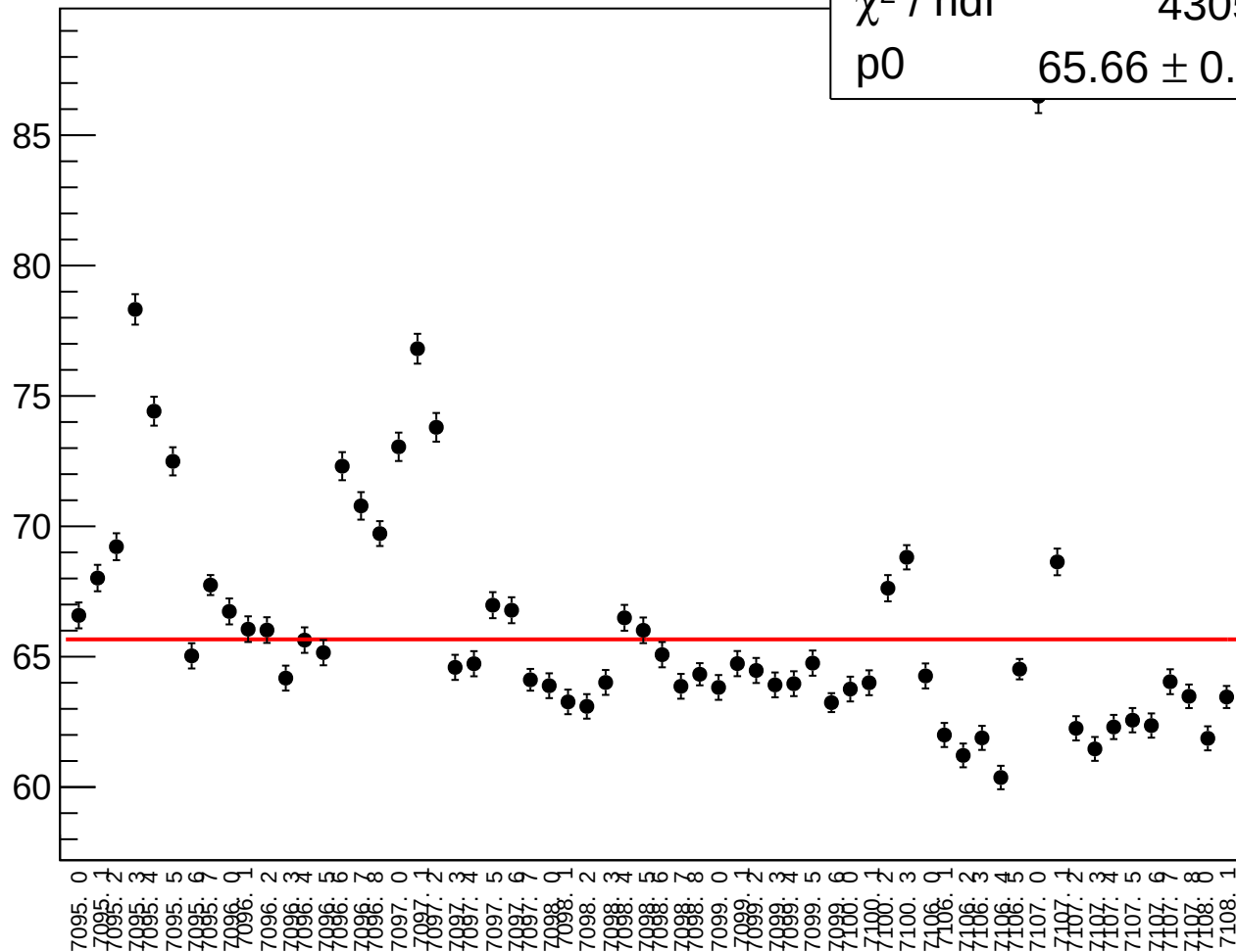
reg_asym_sam_15_avg_rms vs run
