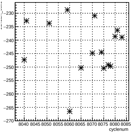
11X12X_coil1:cyclenum
