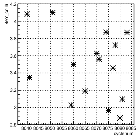
4eY_coil6:cyclenum
