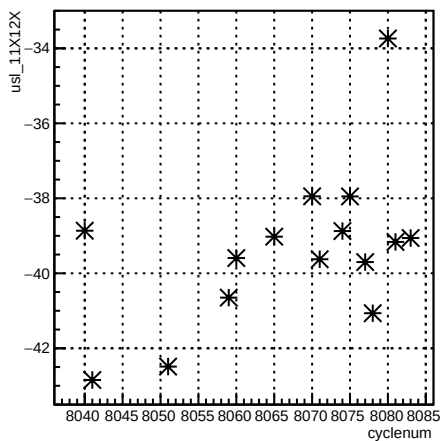
usl_11X12X:cyclenum
