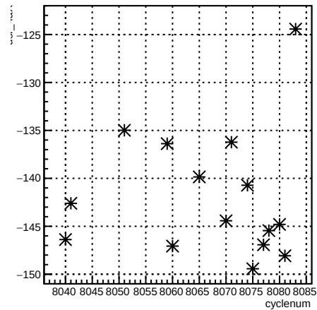
usr_4aX:cyclenum
