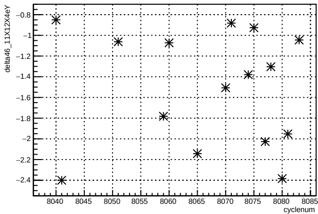
delta46_11X12X4eY:cyclenum
