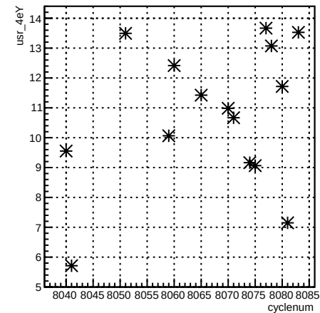
usr_4eY:cyclenum
