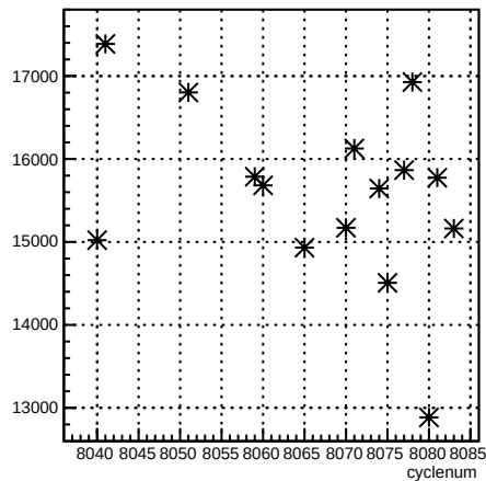
usl_coil7:cyclenum
