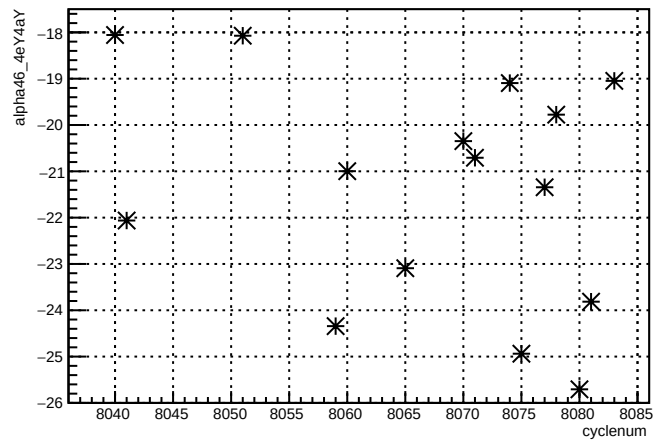
alpha46_4eY4aY:cyclenum
