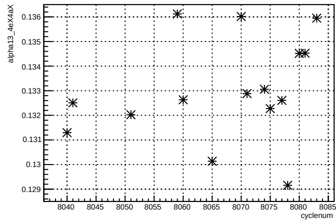
alpha13_4eX4aX:cyclenum
