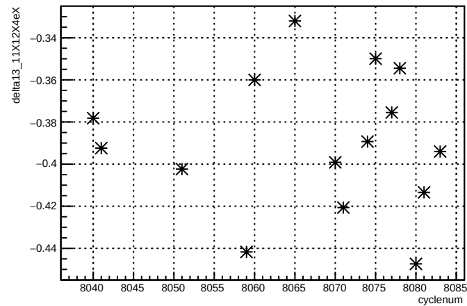
delta13_11X12X4eX:cyclenum
