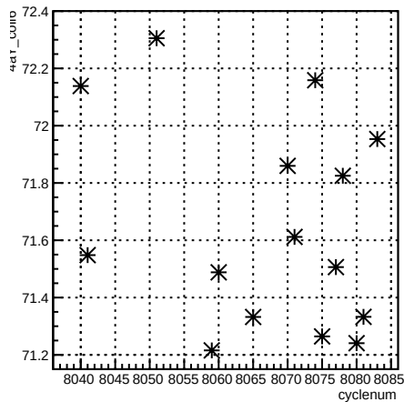
4aY_coil6:cyclenum
