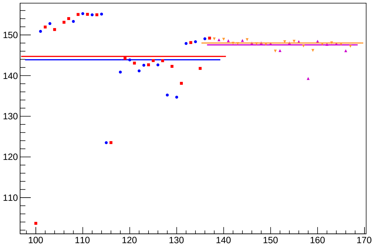
yield_bcm_an_us_mean vs Slug, Sign Corrected
