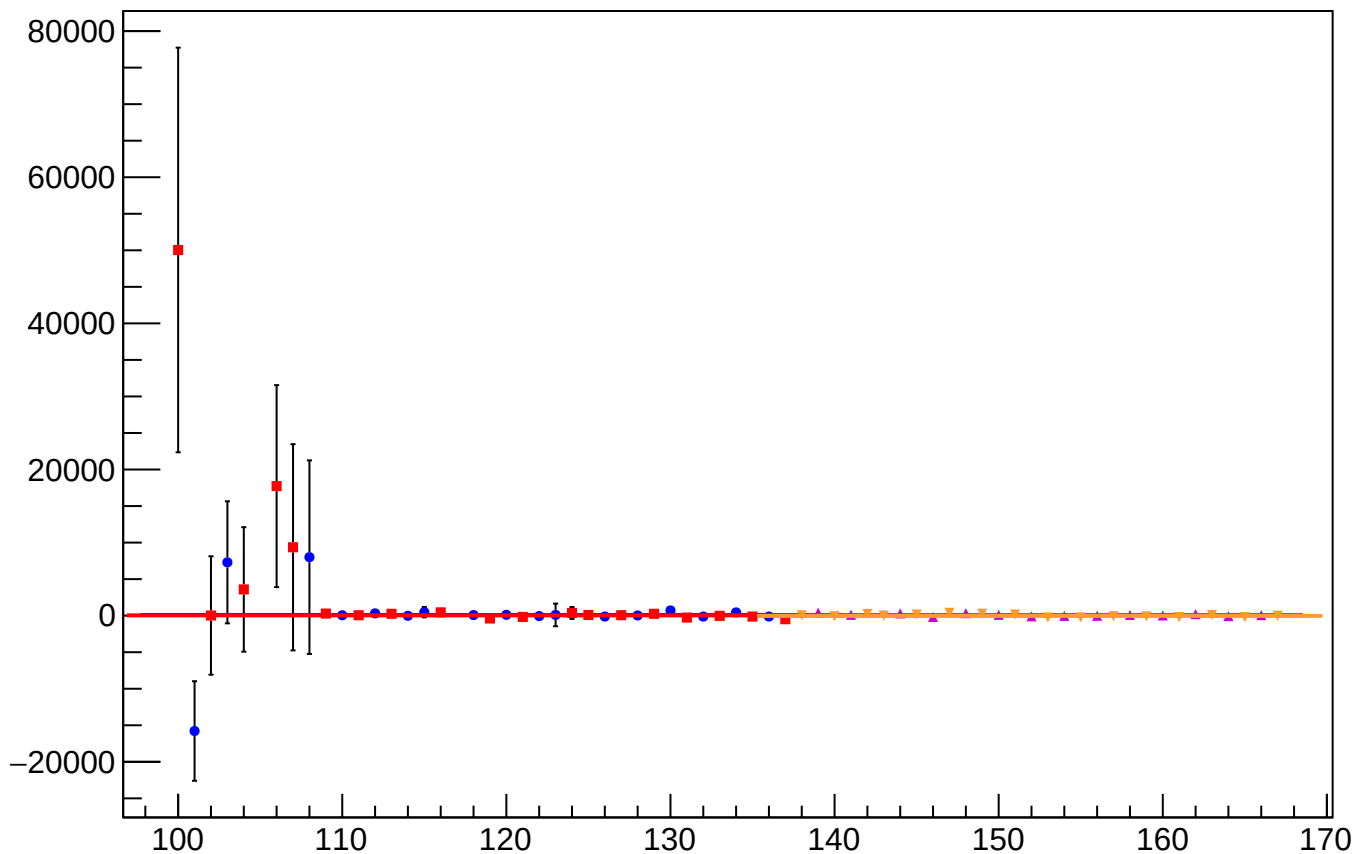
asym_cav4cQ_mean vs Slug, Sign Corrected
