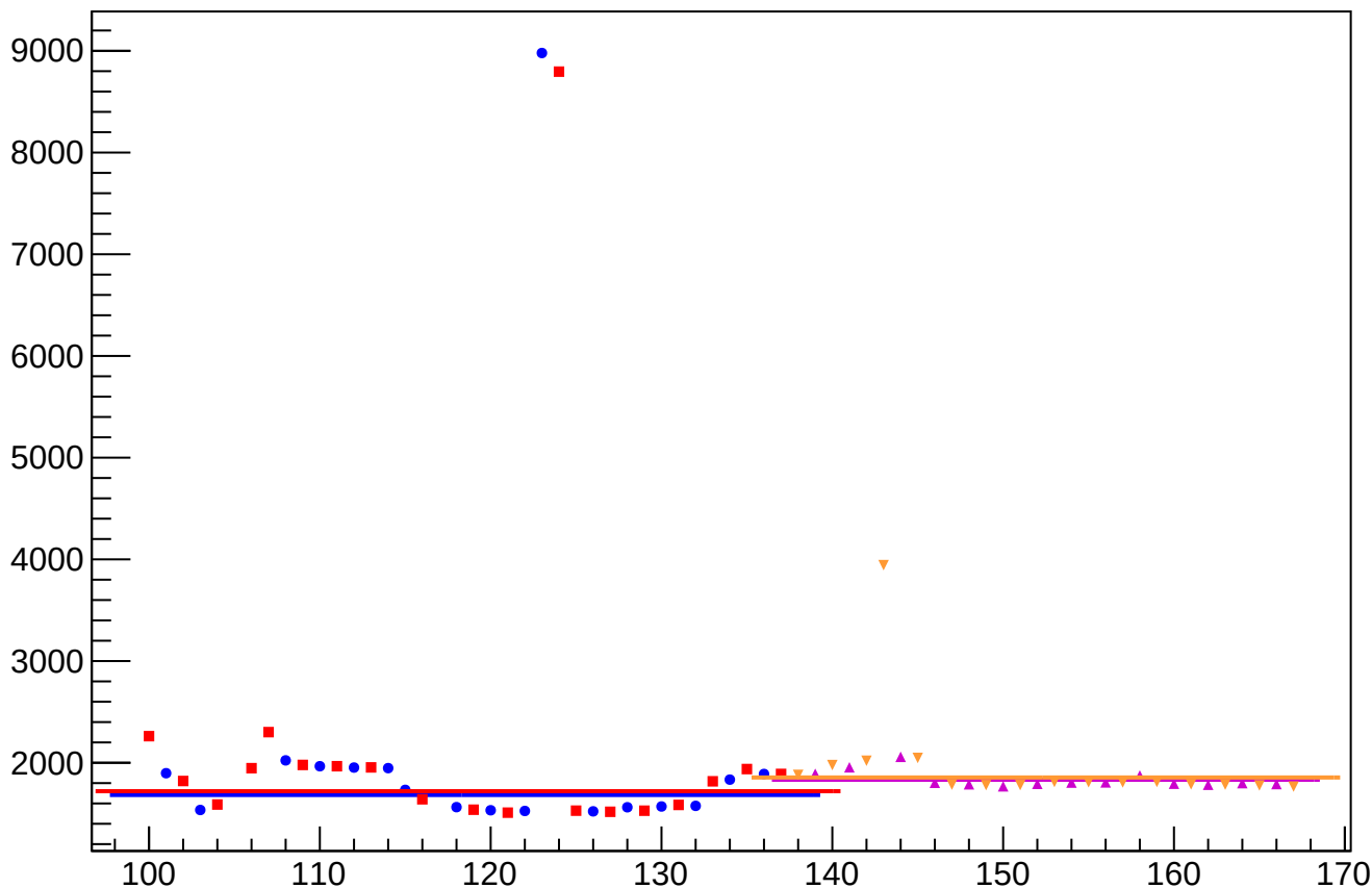
reg_asym_atl_dd_rms vs Slug, Sign Corrected
