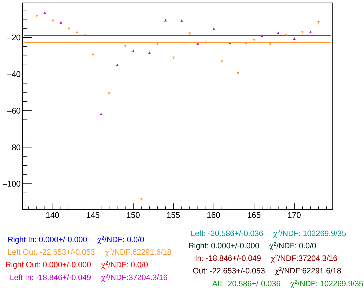
reg_asym_bcm_an_ds_diff_bpm1X_slope vs Slug, Sign Corrected
