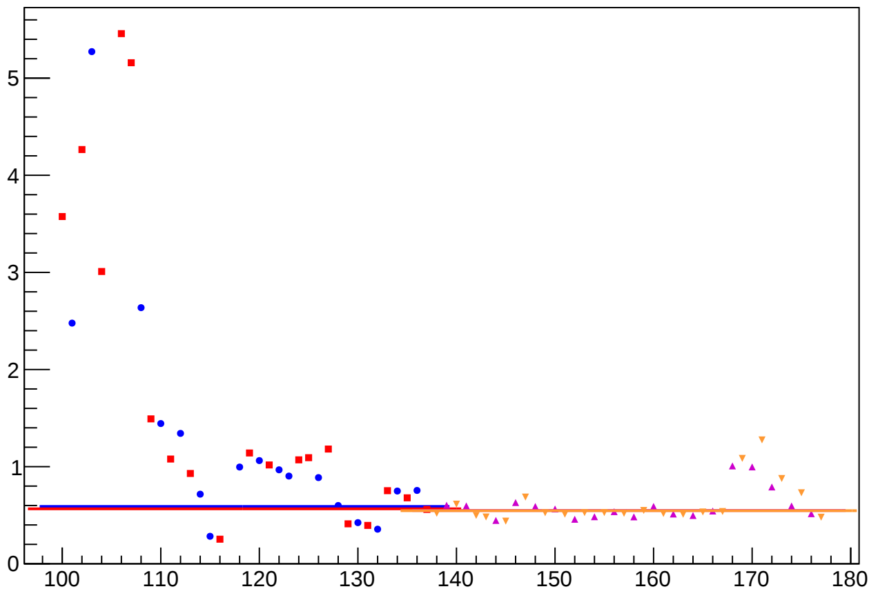
yield_cav4cQ_rms vs Slug, Sign Corrected
