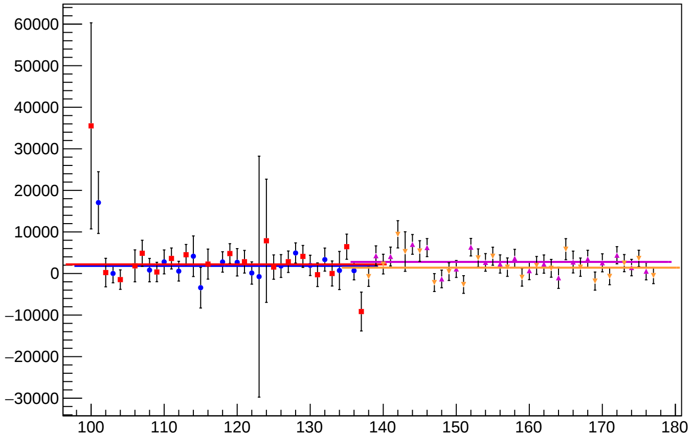
reg_asym_atr1l2_avg_mean vs Slug, Sign Corrected
