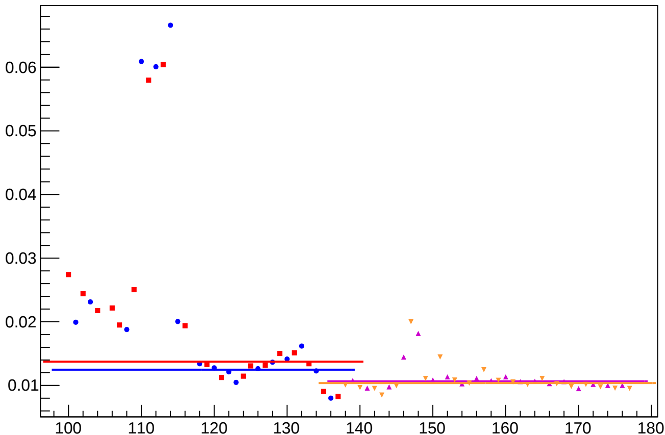
yield_sam1_rms vs Slug, Sign Corrected
