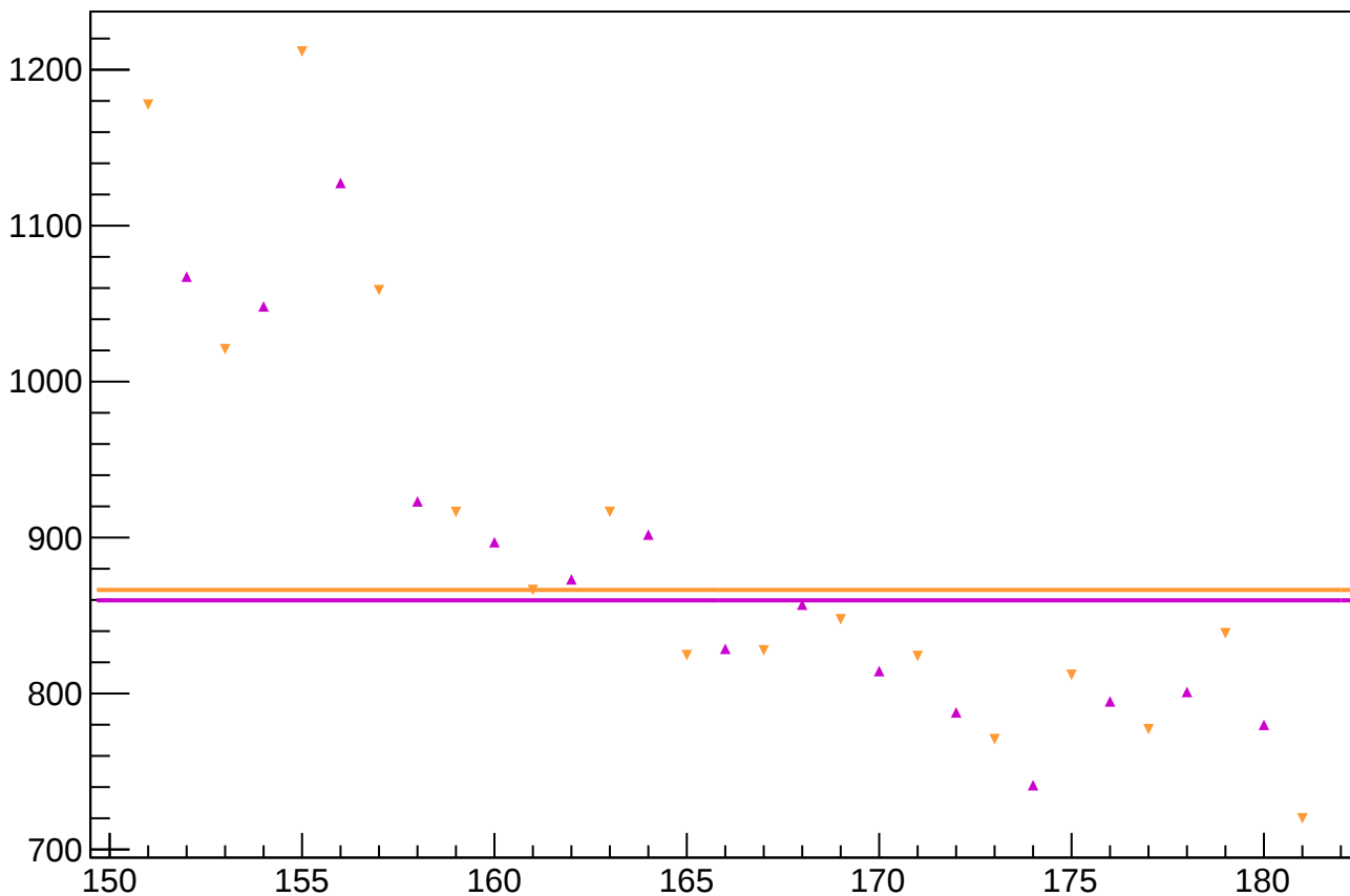
asym_sam_24_68_dd_correction_rms vs Slug
