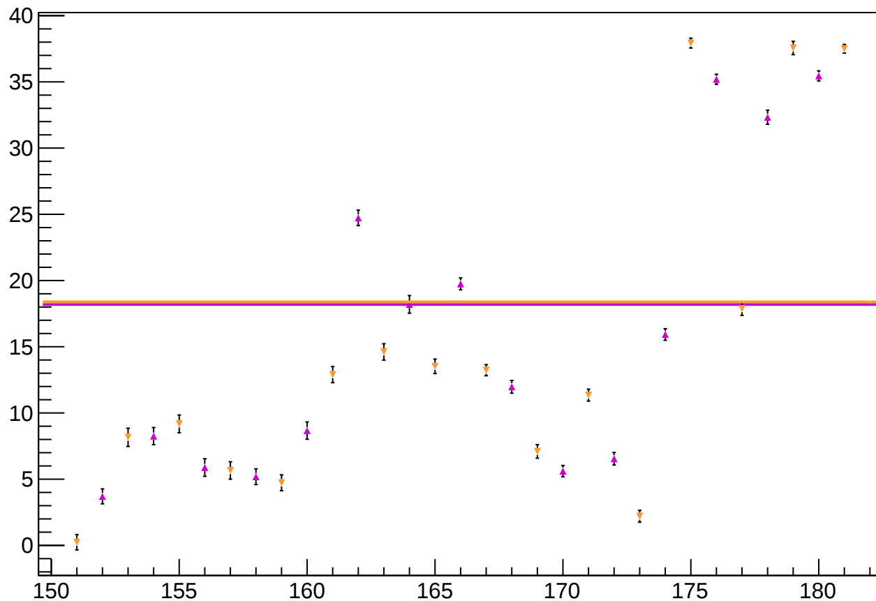
reg_asym_sam_26_48_dd_diff_bpm1X_slope vs Slug
