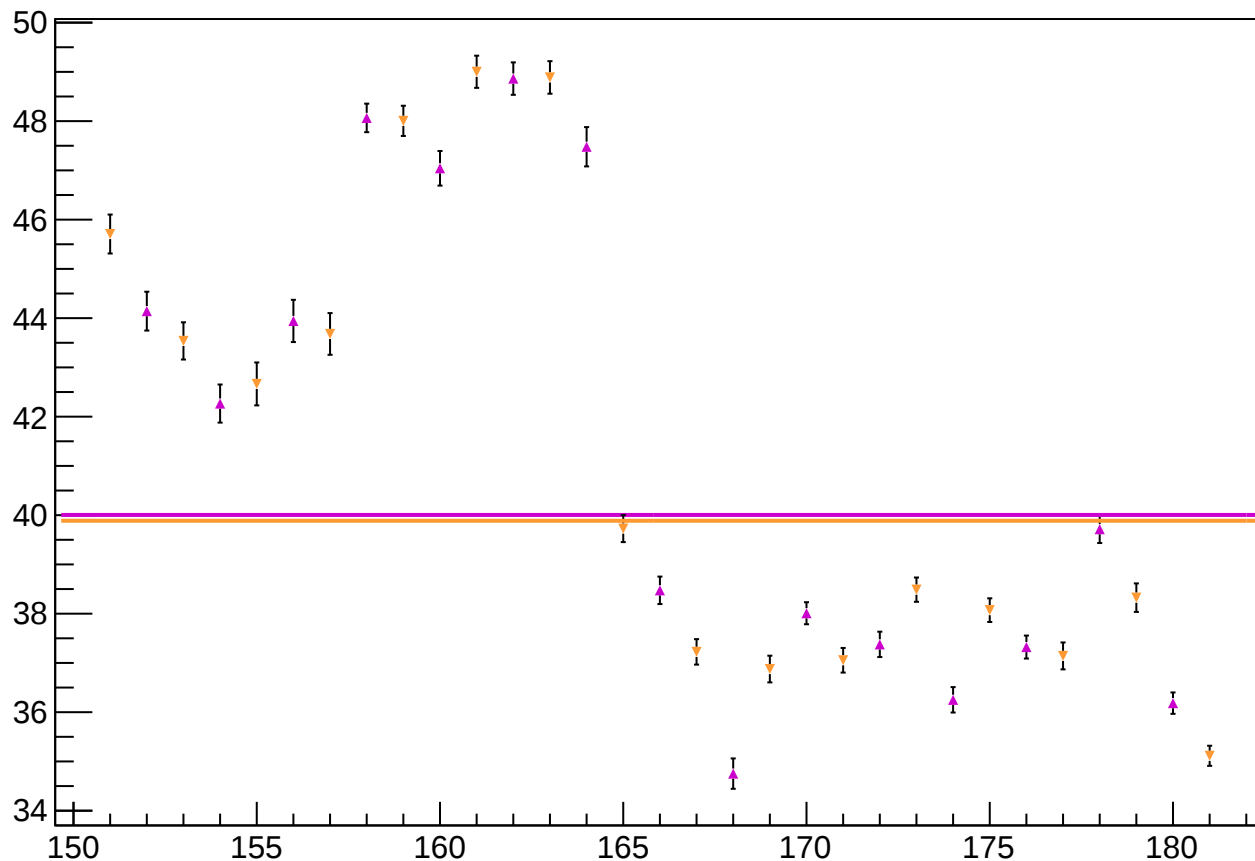
reg_asym_sam_15_26_dd_diff_bpm4eY_slope vs Slug
