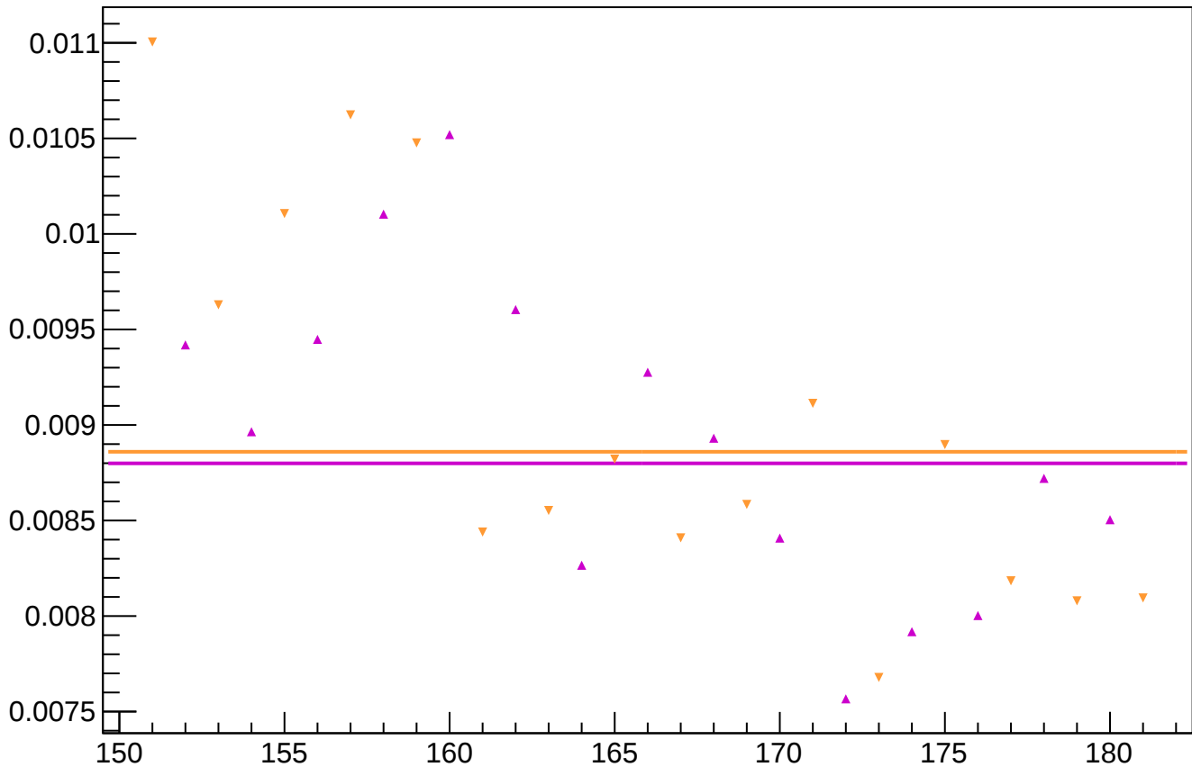
yield_cav4dX_rms vs Slug
