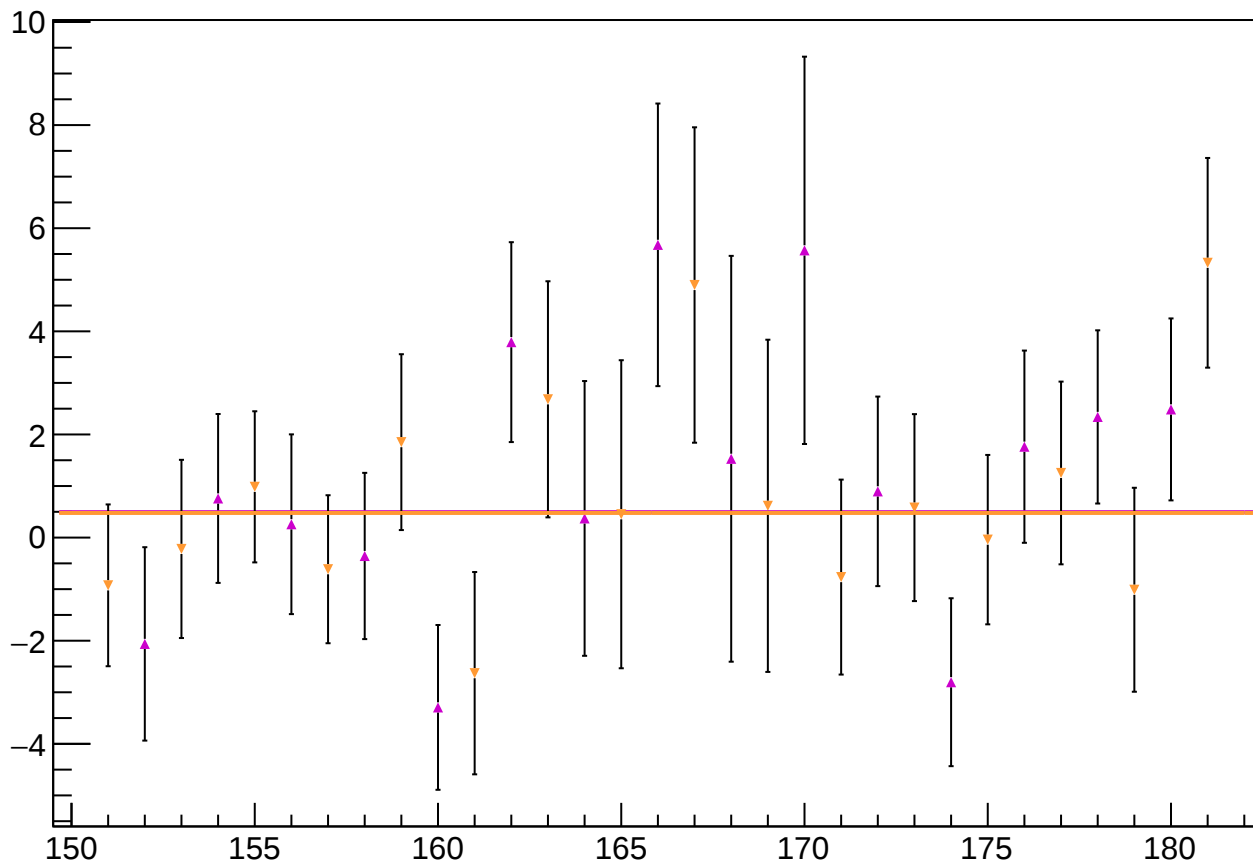
asym_ds_avg_correction_mean vs Slug
