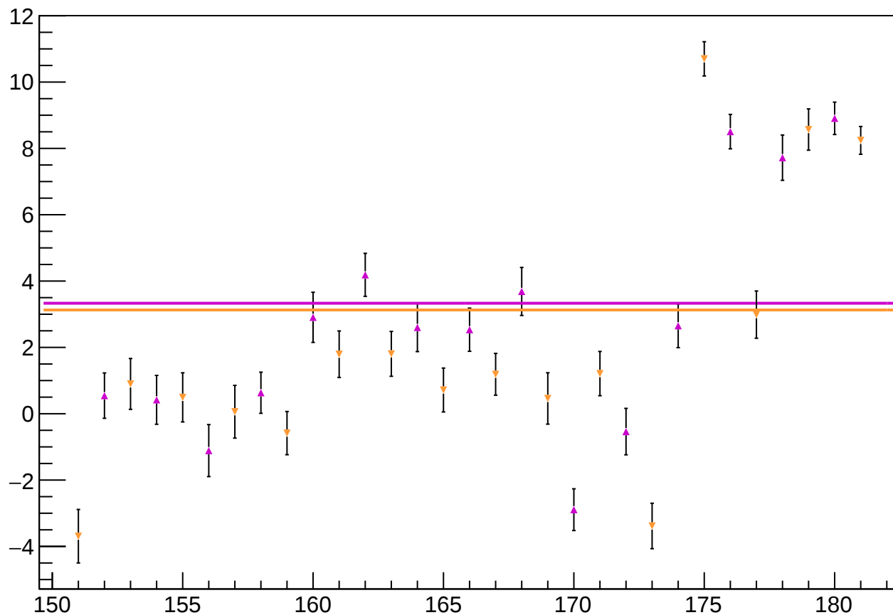
reg_asym_sam_15_dd_diff_bpm1X_slope vs Slug
