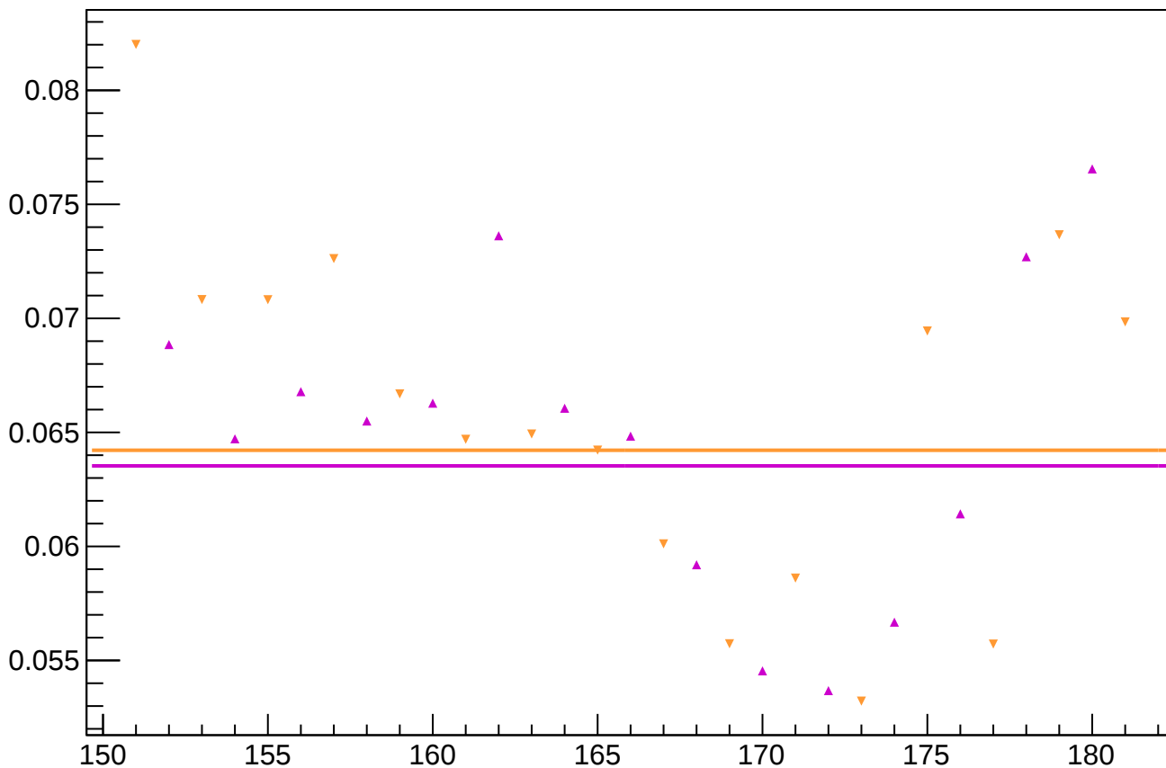
yield_sam4_rms vs Slug
