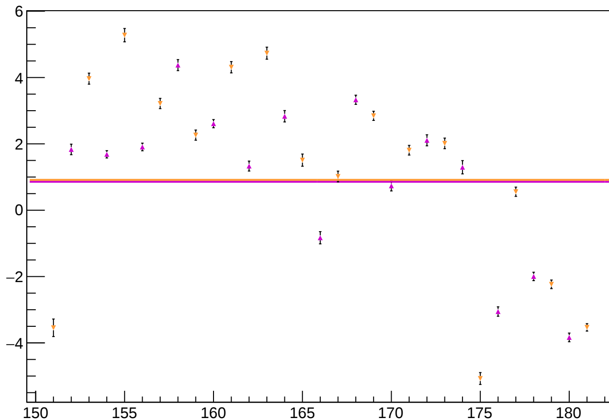
reg_asym_bcm_dg_us_diff_bpm4aY_slope vs Slug
