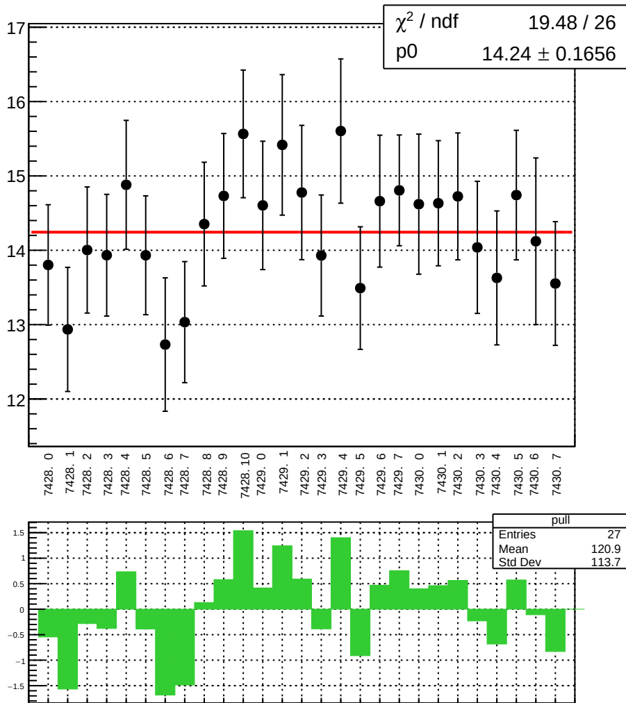
reg_asym_sam_37_26_dd_diff_bpm4eY_slope vs run
