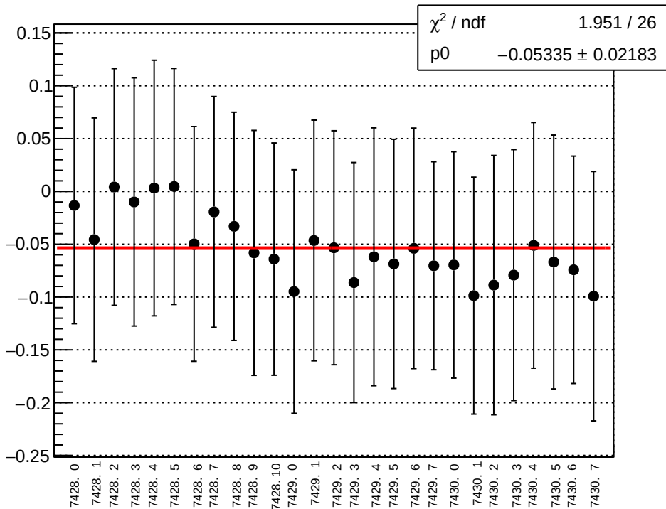
reg_asym_sam_15_48_dd_diff_bpm12X_slope vs run
