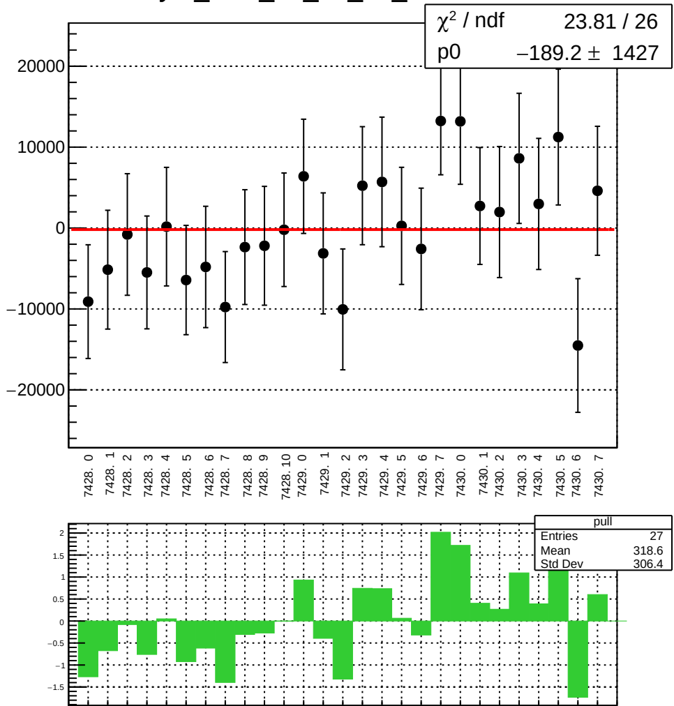
asym_sam_24_68_dd_mean vs run
