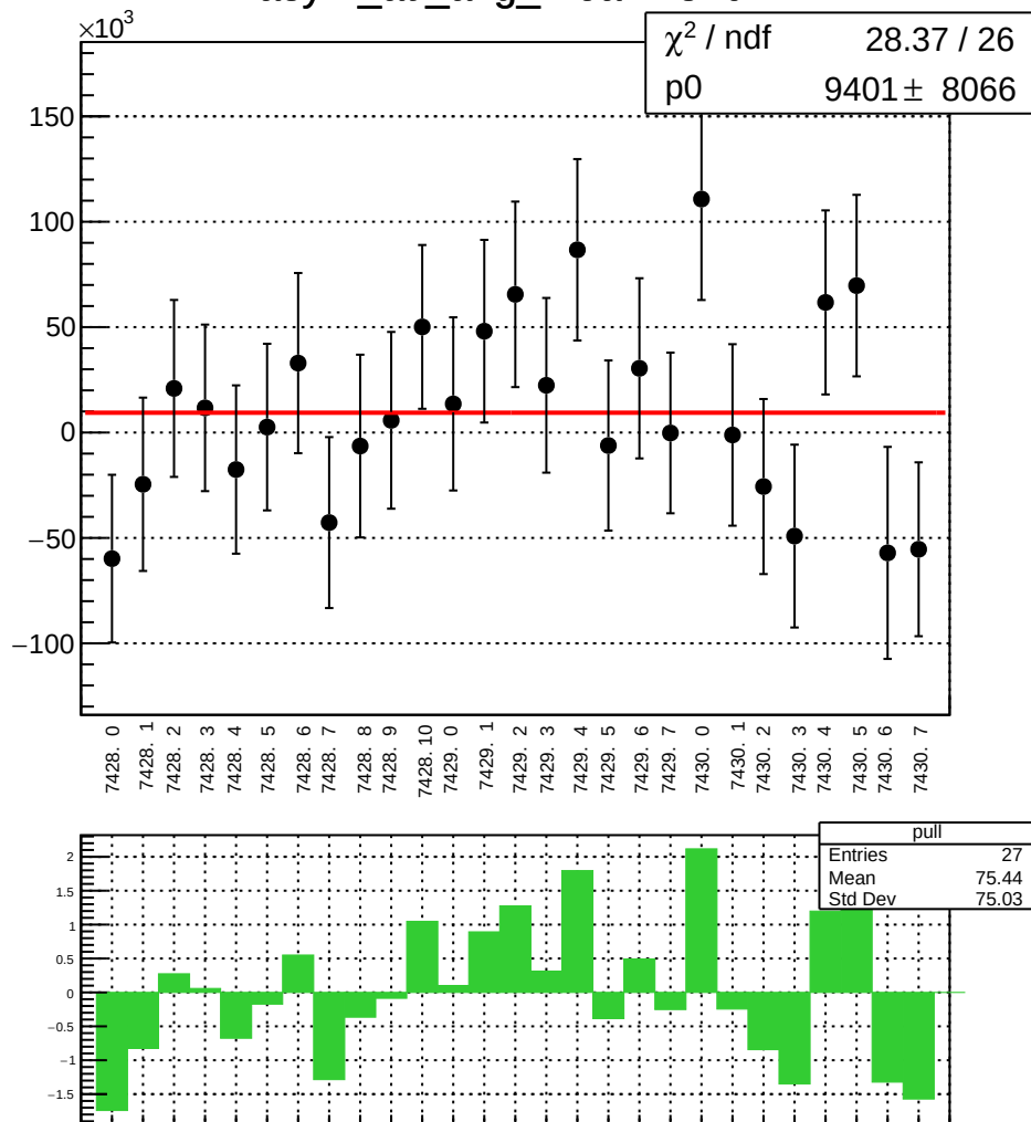
asym_atl_avg_mean vs run
