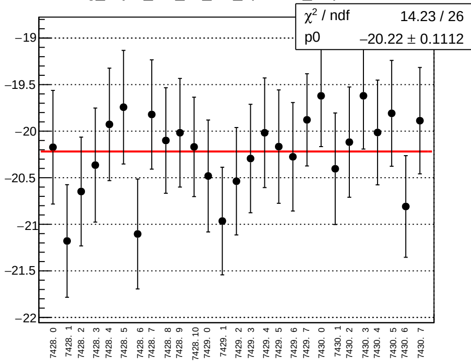
reg_asym_at2_dd_diff_bpm12X_slope vs run
