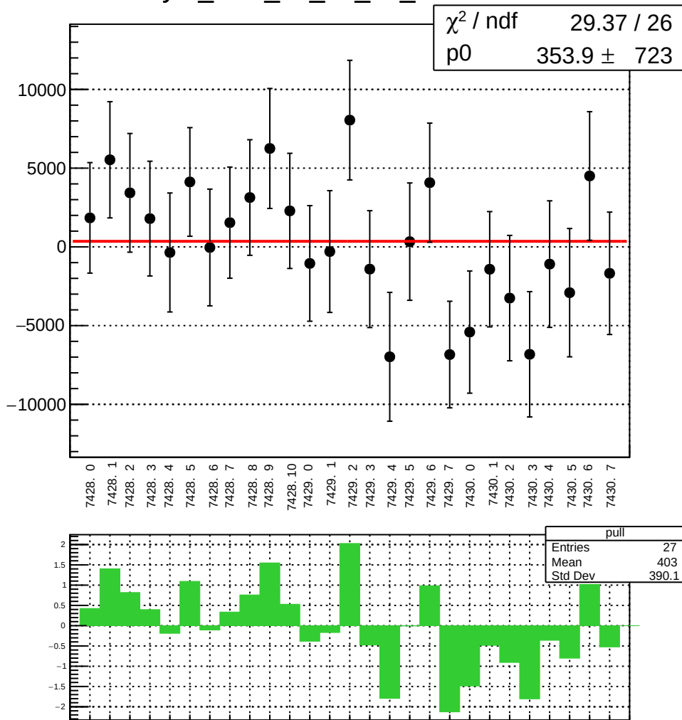
asym_sam_15_48_dd_mean vs run
