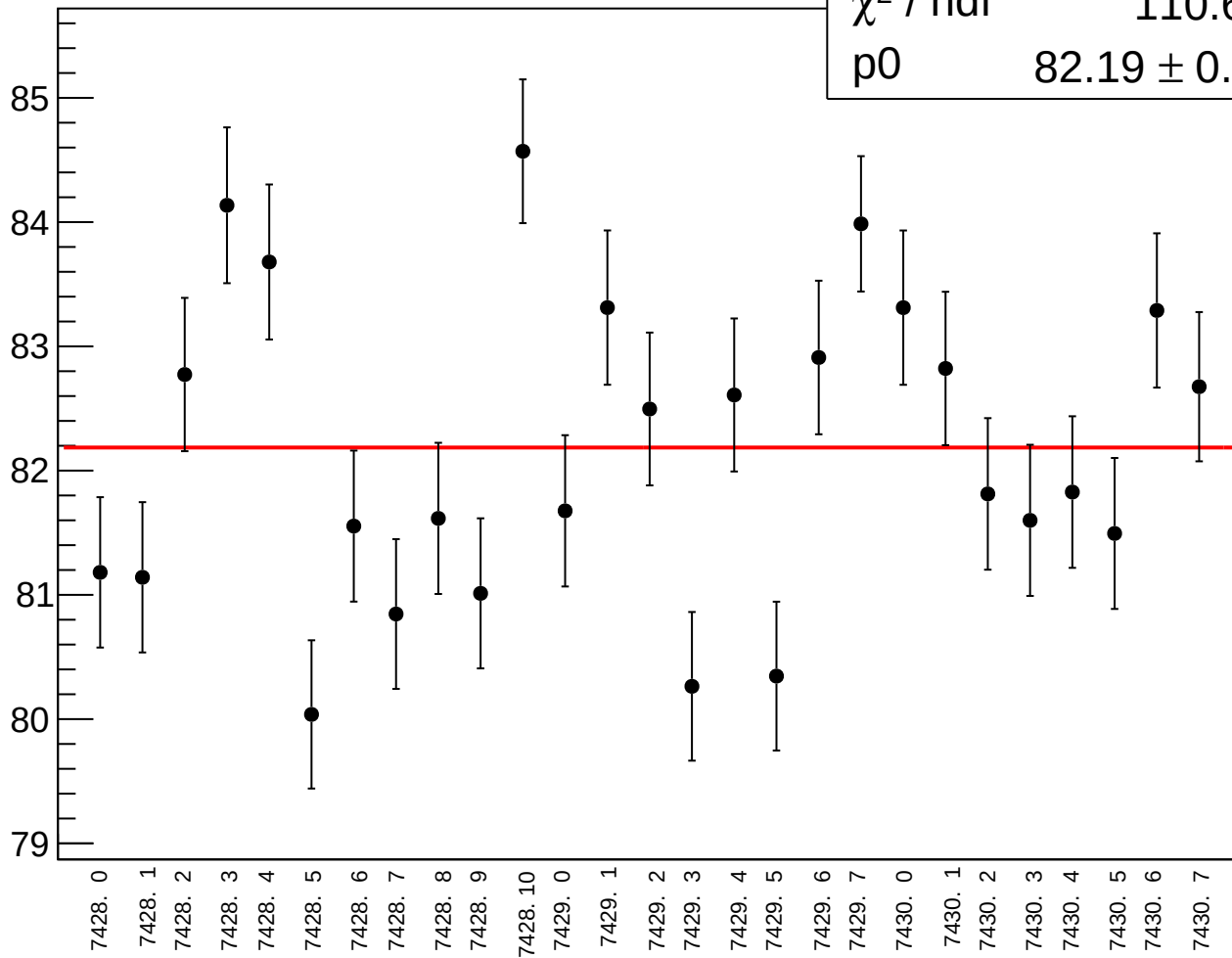
reg_asym_sam_3748_avg_rms vs run
