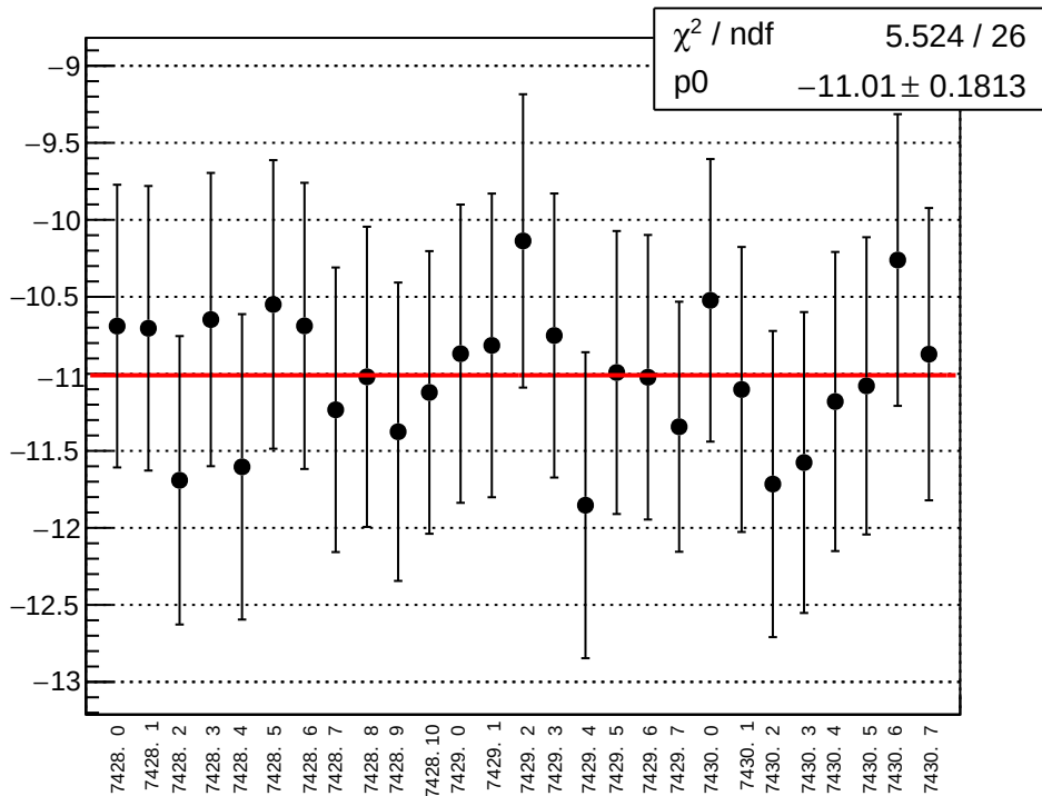
reg_asym_sam_37_26_dd_diff_bpm4eX_slope vs run
