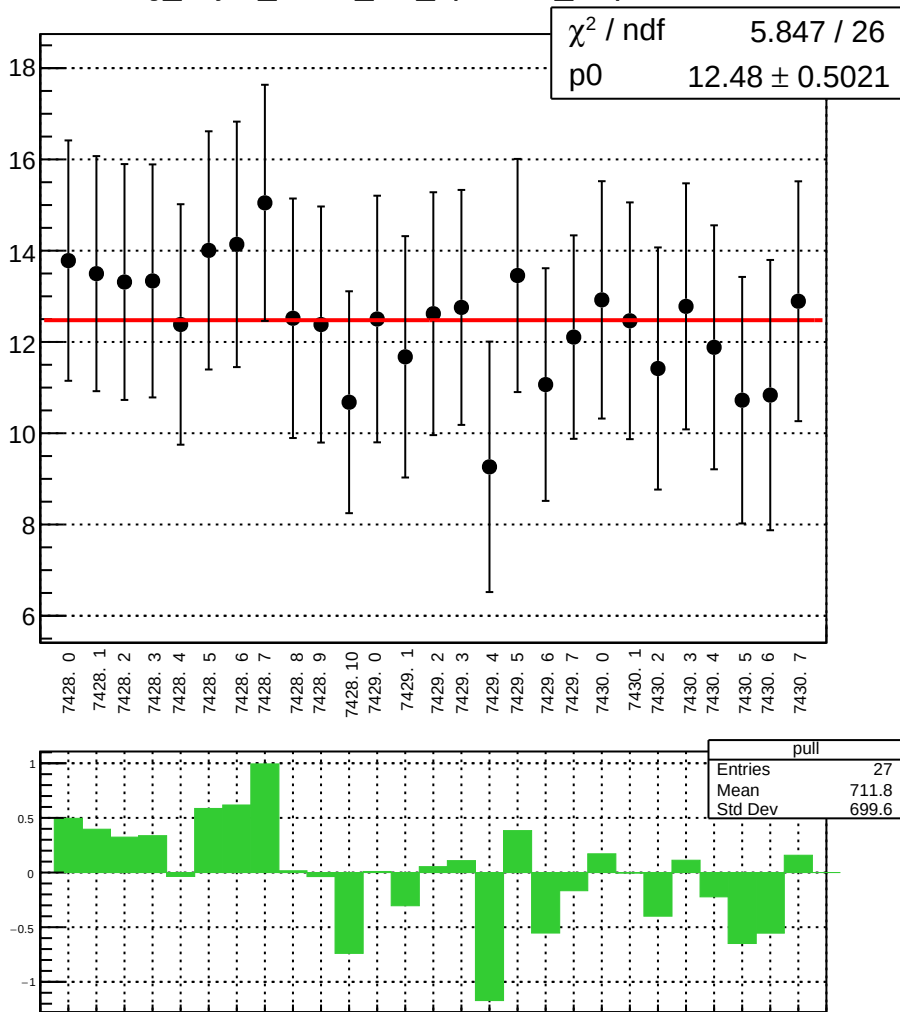
reg_asym_sam1_diff_bpm4eY_slope vs run
