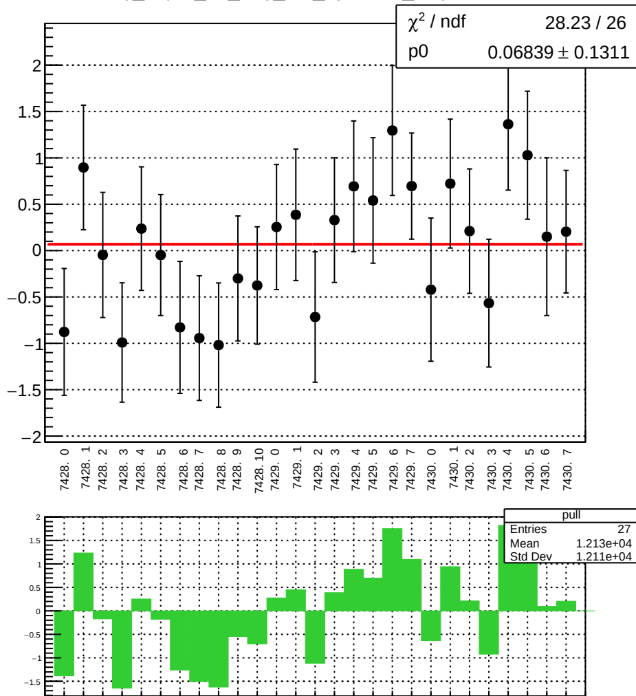
reg_asym_ds_avg_diff_bpm4eY_slope vs run
