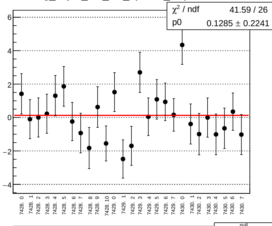
reg_asym_dsr_diff_bpm1X_slope vs run
