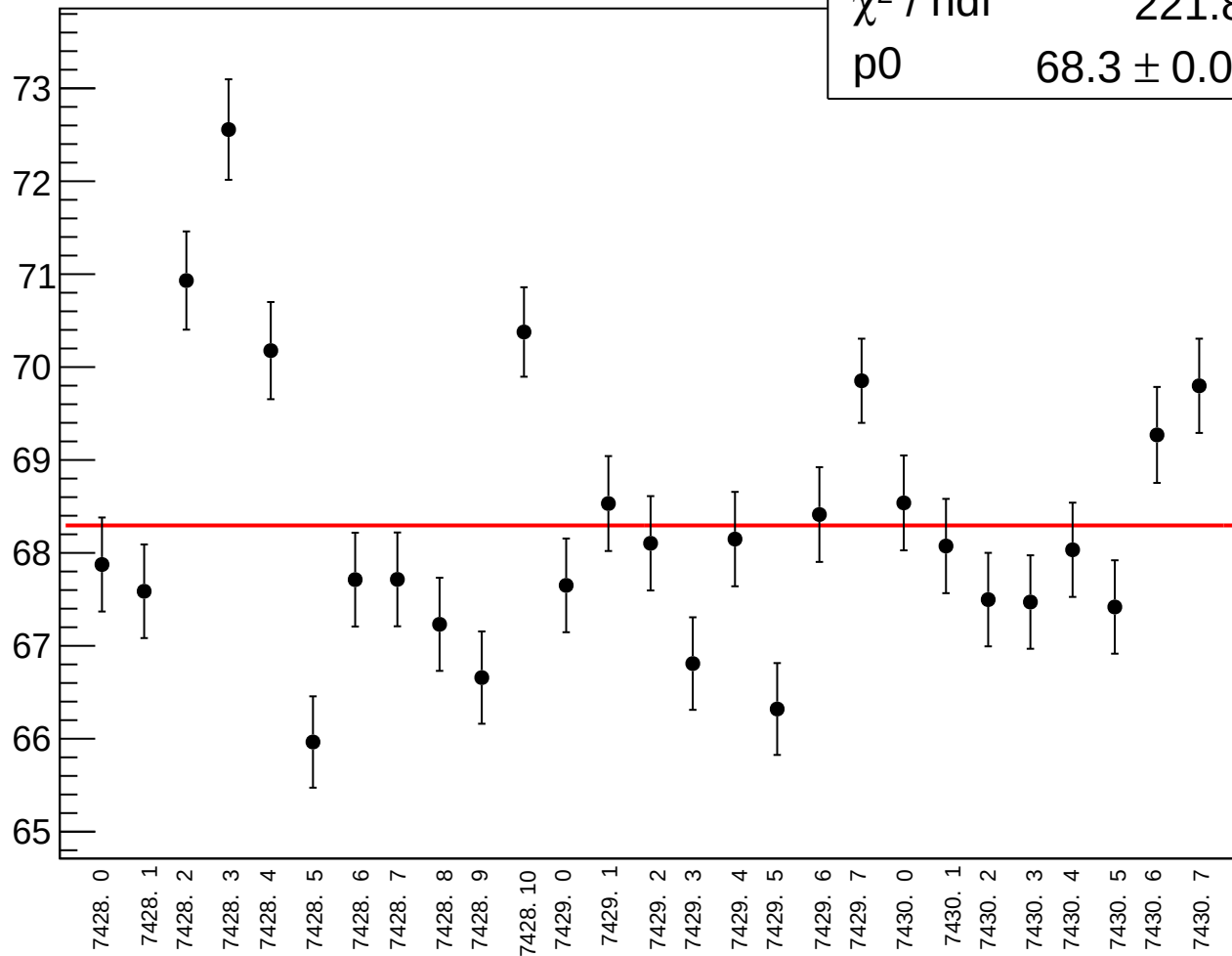
reg_asym_sam_2468_avg_rms vs run
