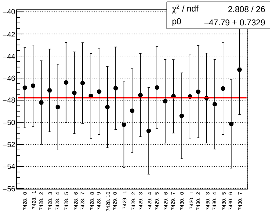
reg asym sam 12345678 avg diff bpm4eX slope vs run
