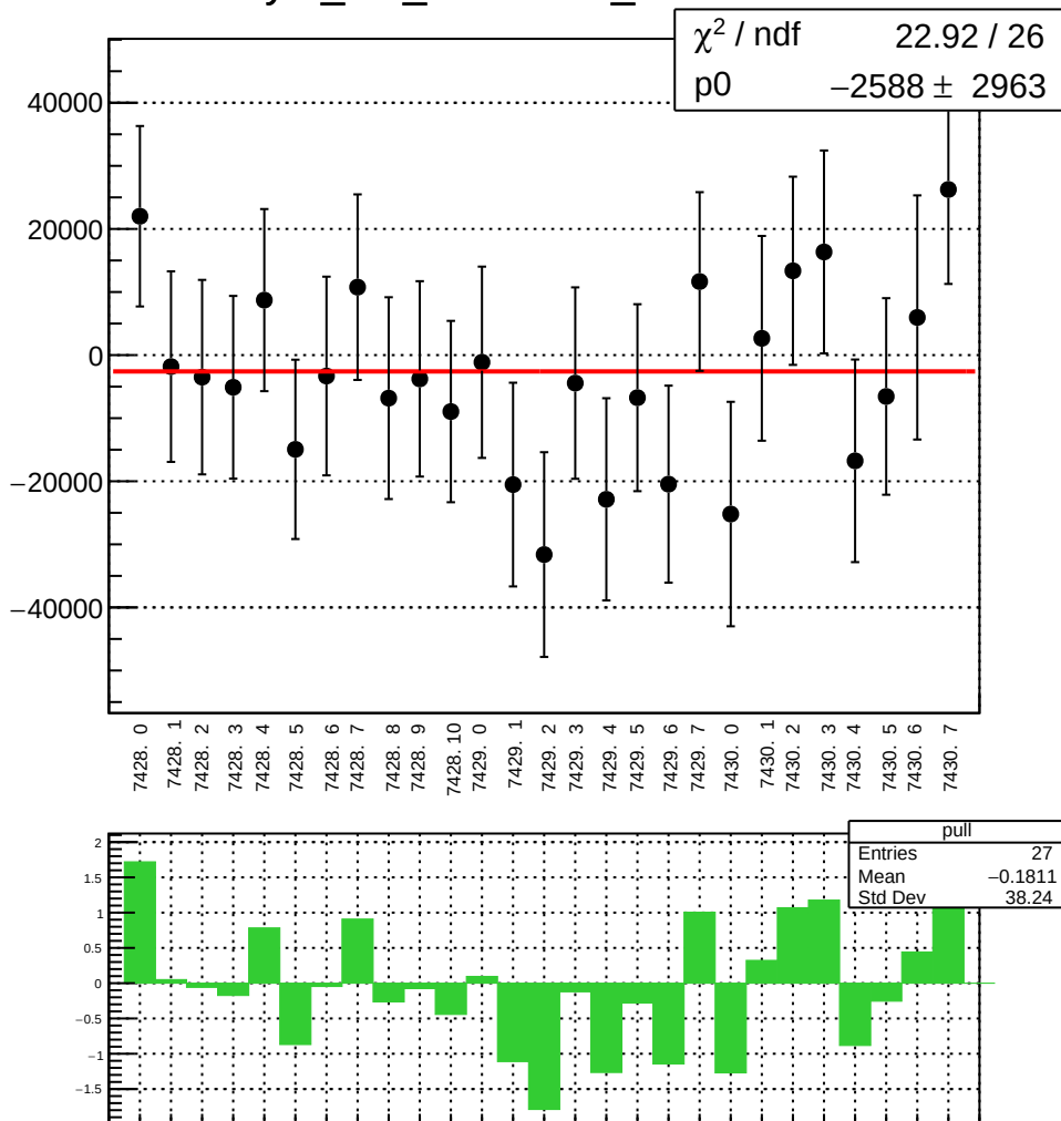
asym_usr_correction_mean vs run
