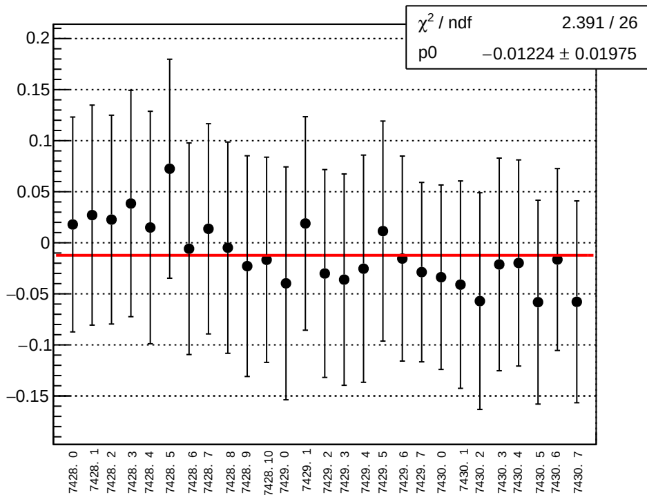
reg_asym_sam_37_48_dd_diff_bpm12X_slope vs run
