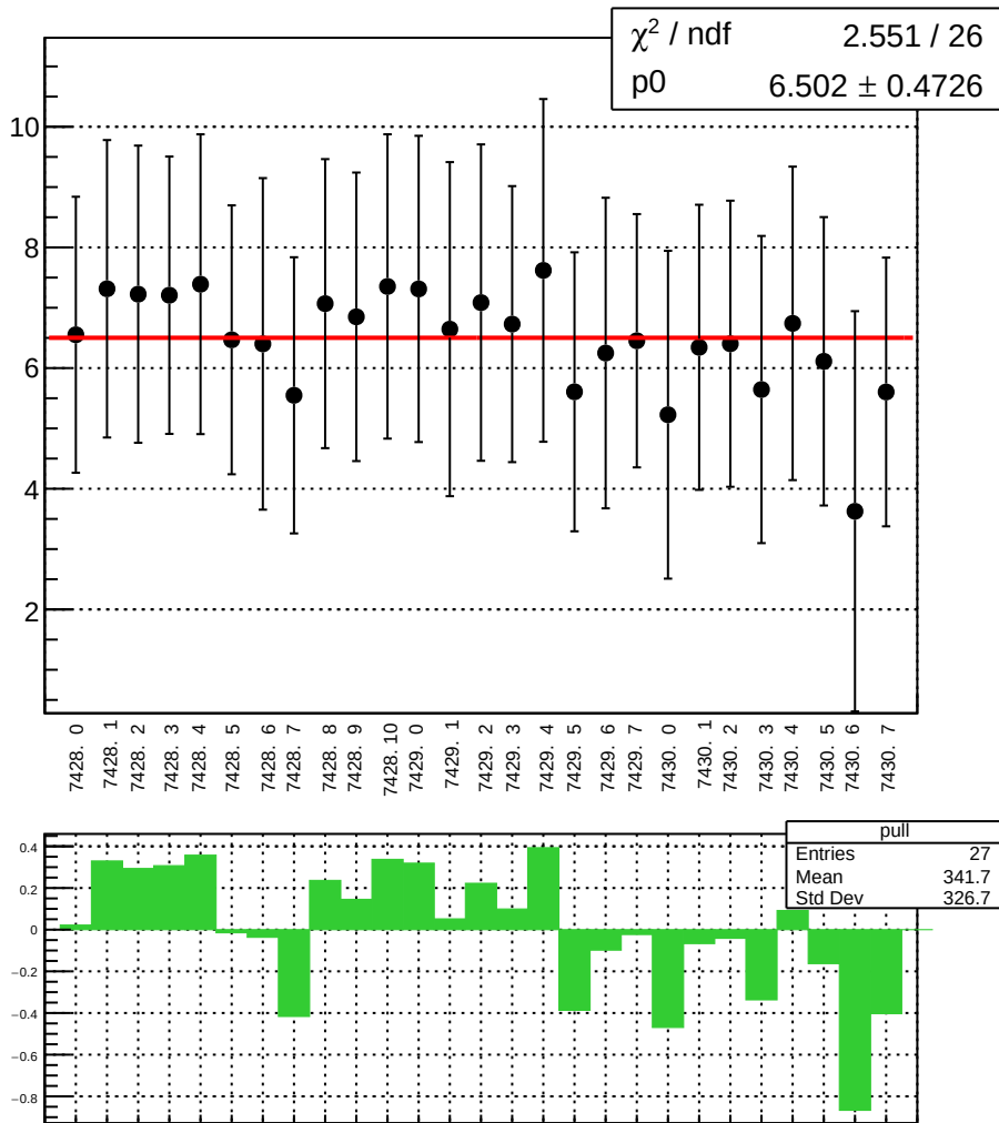
reg_asym_sam_37_48_dd_diff_bpm4aY_slope vs run
