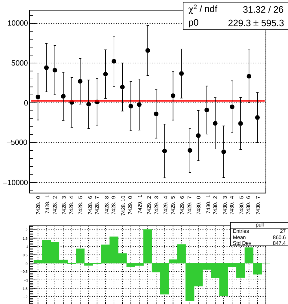
asym_sam_1357_avg_correction_mean vs run
