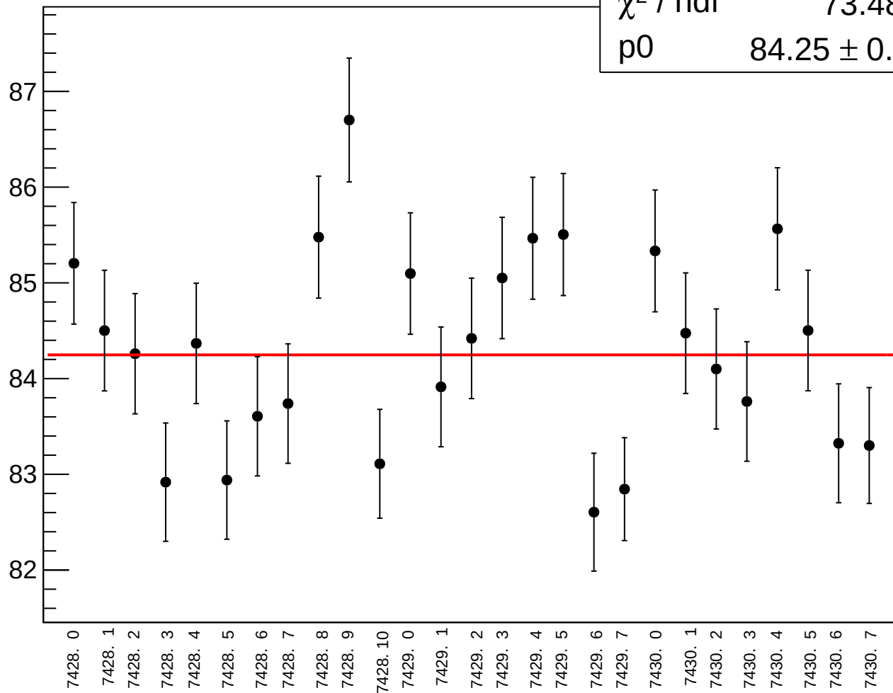
asym_ds_avg_rms vs run
