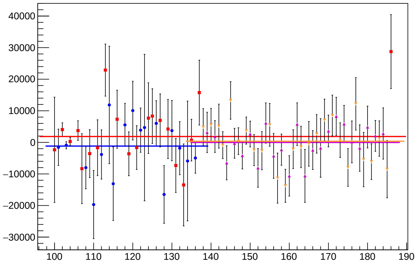
asym_atl1r2_avg_correction_mean vs Slug
