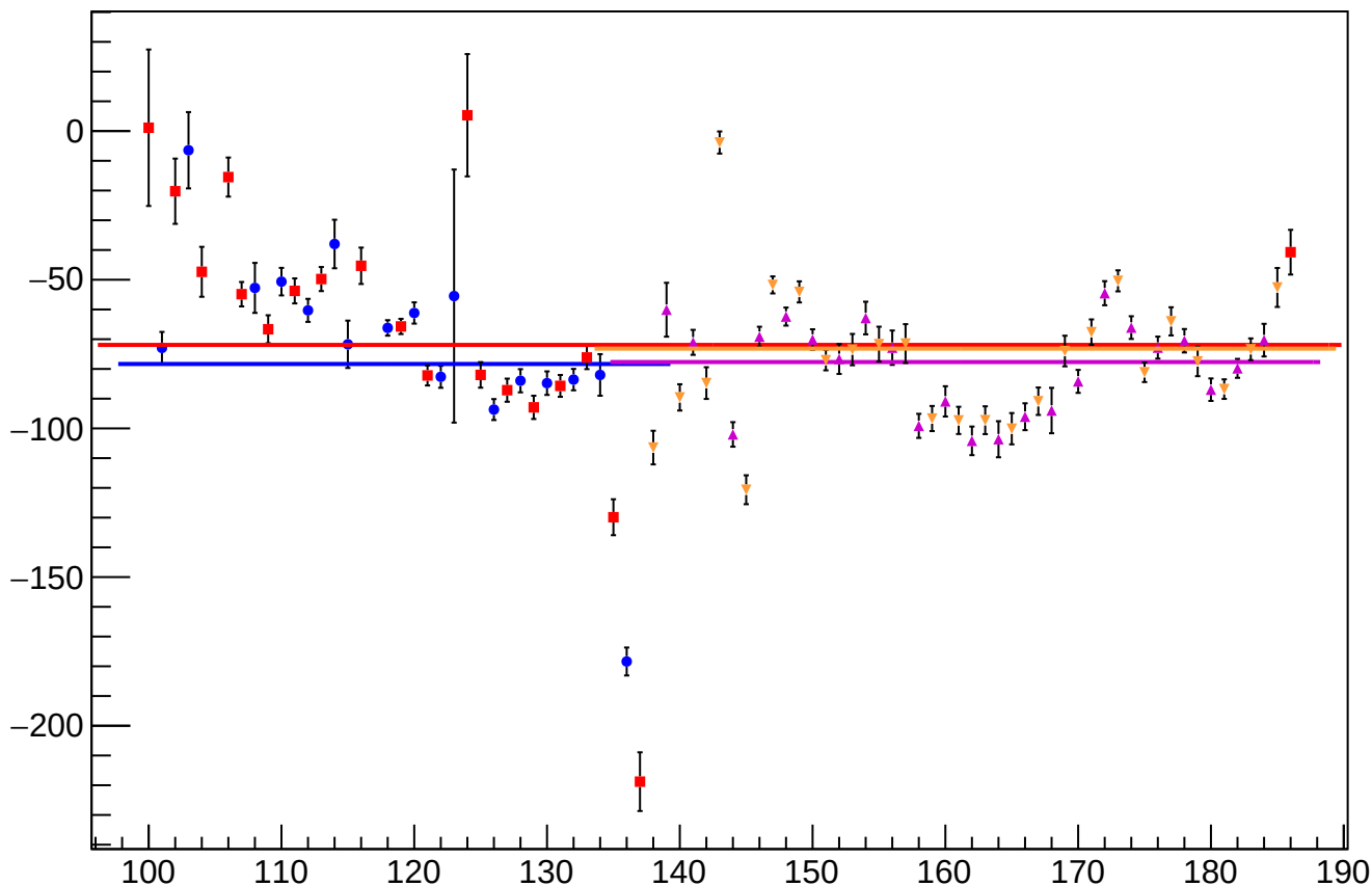
reg_asym_atl_dd_diff_bpm4eY_slope vs Slug
