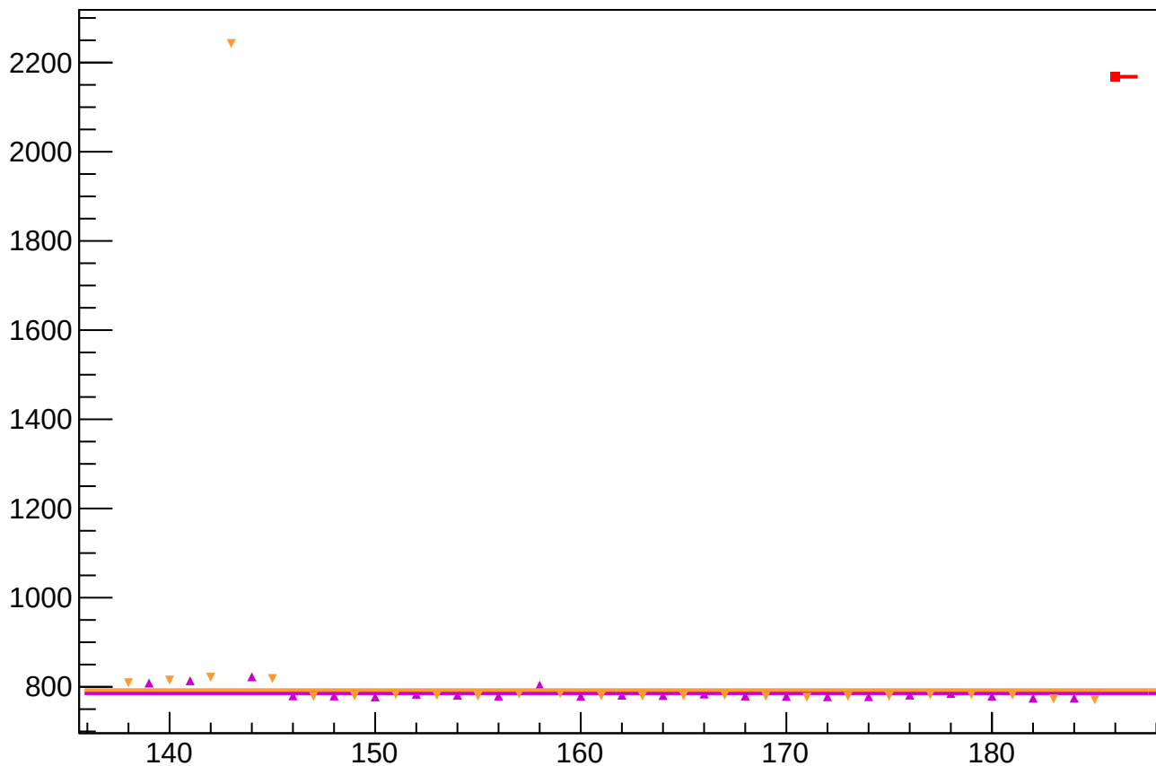
cor_asym_us_dd_rms vs Slug
