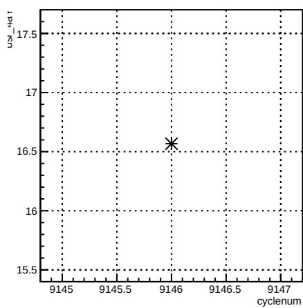
usr_4aY:cyclenum
