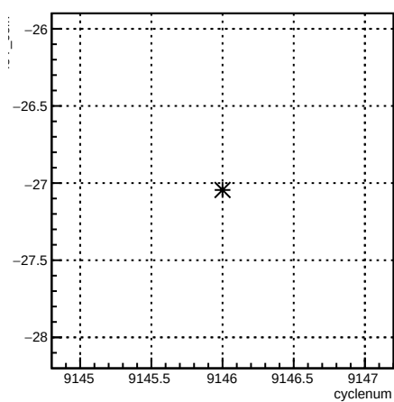
4eY_coil7:cyclenum
