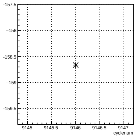
usr_4aX:cyclenum
