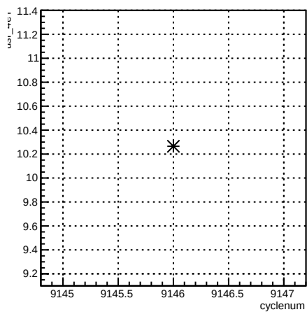
usr_4eY:cyclenum
