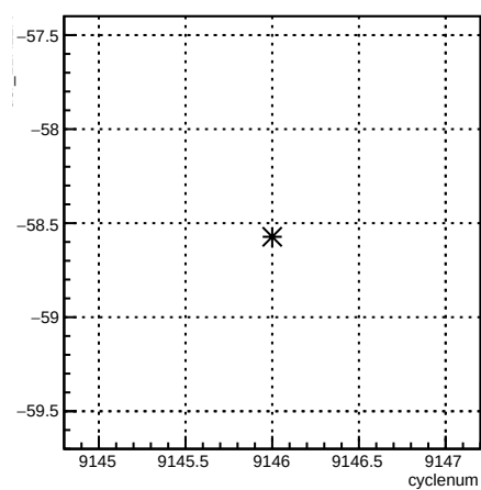
usr_11X12X:cyclenum
