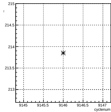
usr_4eX:cyclenum
