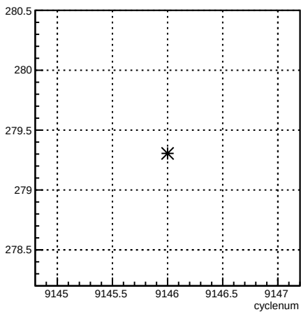
4eY_coil4:cyclenum
