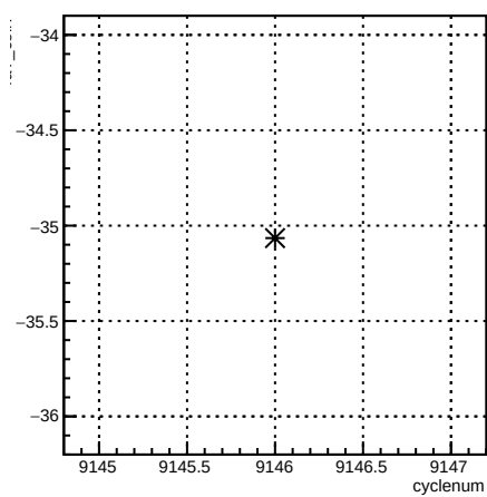
4aY_coil7:cyclenum
