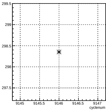
4aY_coil4:cyclenum
