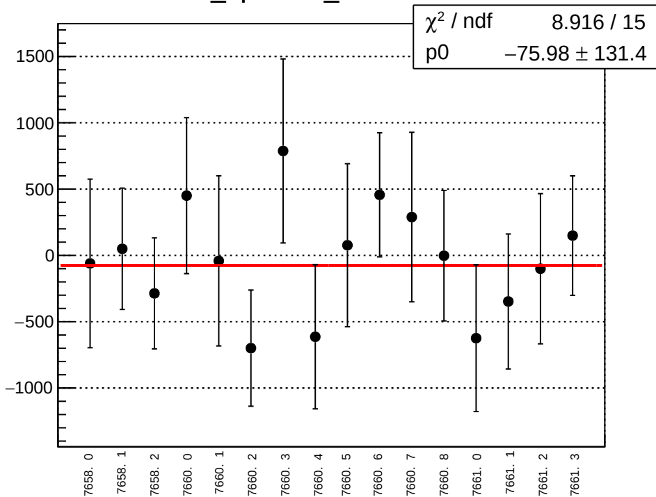
diff_bpm11Y_mean vs uen
