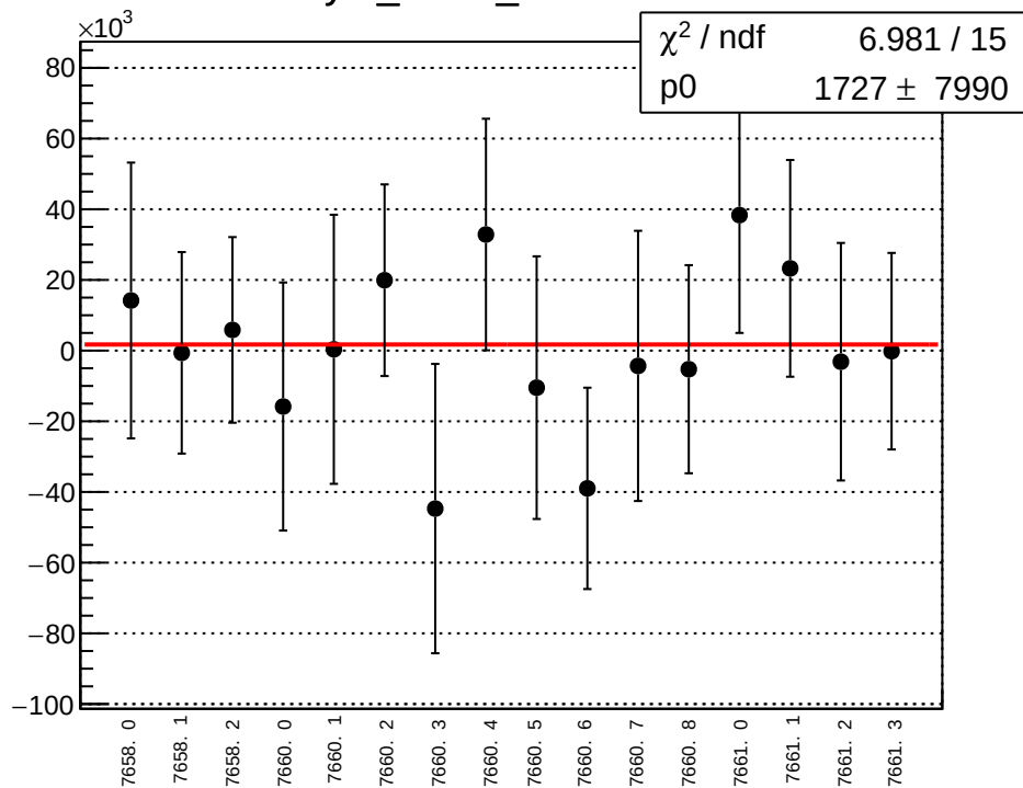
asym_sam5_mean vs run
