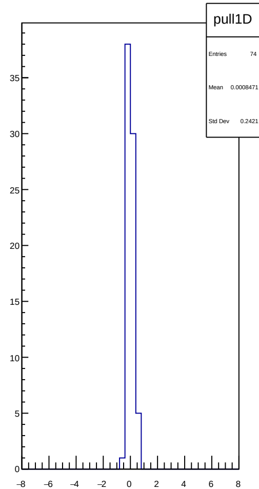
\chi^2 / \text{ndf} 4.339 / 73 p0 9.611 \pm 1.295
