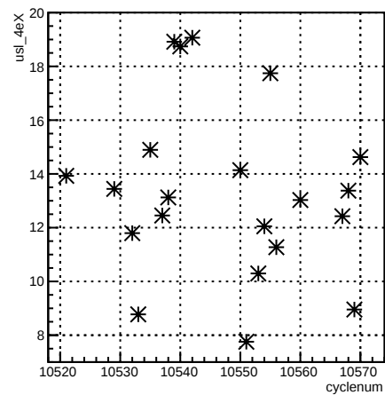
usl_4eX:cyclenum
