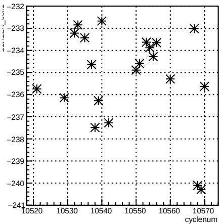
11X12X_coil1:cyclenum
