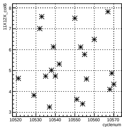
11X12X_coil6:cyclenum
