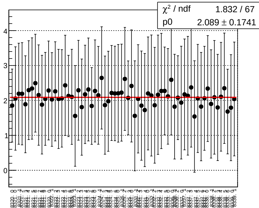
reg_asym_sam_3726_avg_diff_bpm12X_slope vs run
