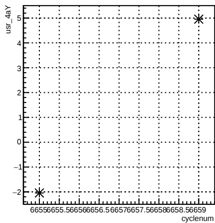
usr_4aY:cyclenum {run == 6621}
