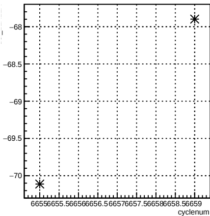
usl_11X12X:cyclenum {run == 6621}
