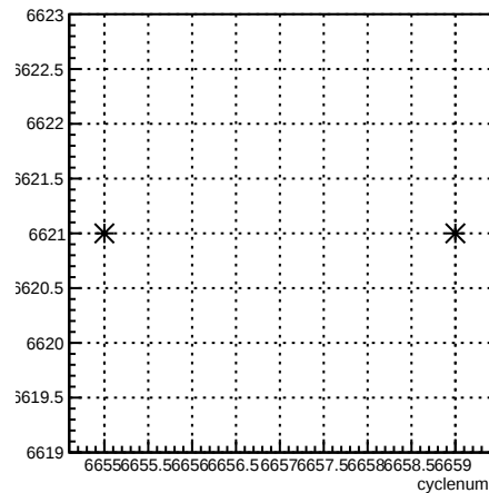
run:cyclenum {run == 6621}
