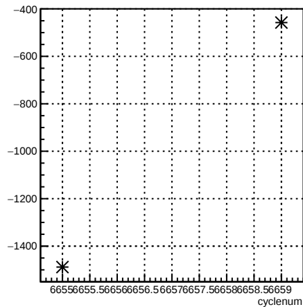
usl_coil6:cyclenum {run == 6621}
