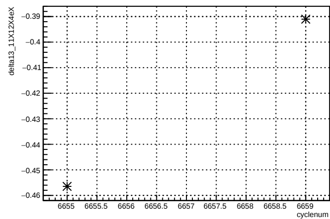
delta13_11X12X4eX:cyclenum {run == 6621}
