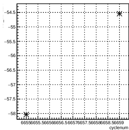
usr_11X12X:cyclenum {run == 6621}
