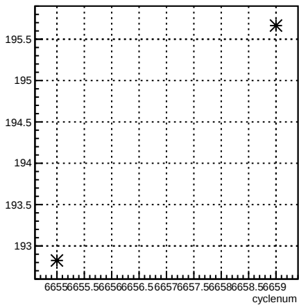
4eY_coil4:cyclenum {run == 6621}
