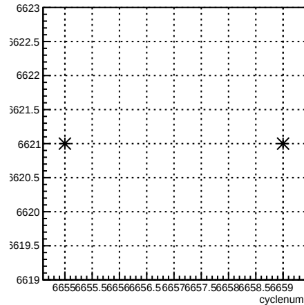
run:cyclenum {run == 6621}
