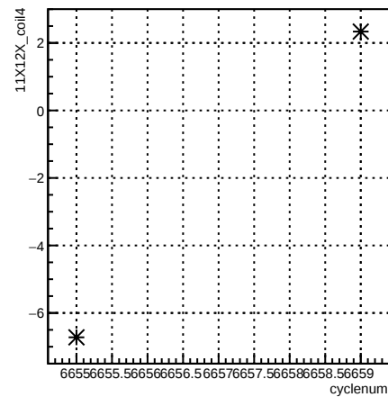
11X12X_coil4:cyclenum {run == 6621}
