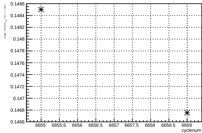
alpha13_4eX4aX:cyclenum {run == 6621}
