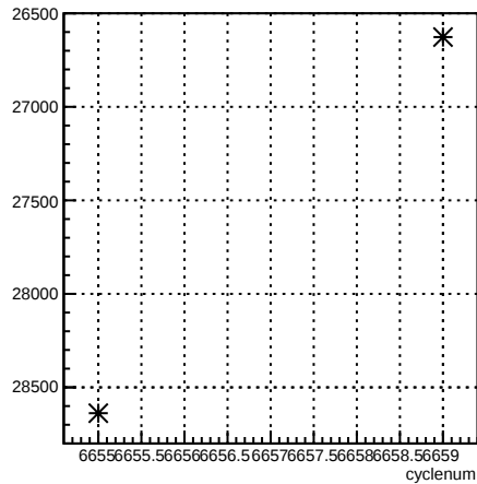
usr_coil1:cyclenum {run == 6621}
