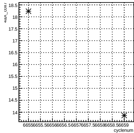
4eX_coil7:cyclenum {run == 6621}
