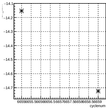
4aY_coil7:cyclenum {run == 6621}
