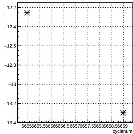
4eY_coil7:cyclenum {run == 6621}
