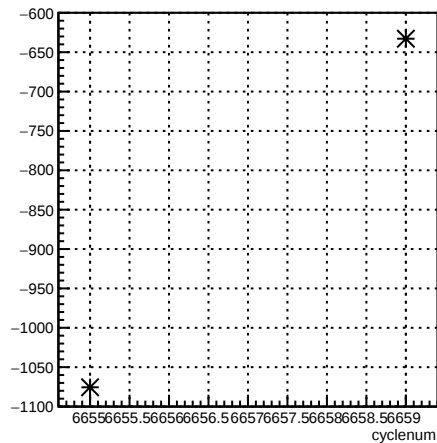
usr_coil6:cyclenum {run == 6621}
