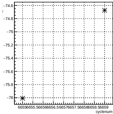
4eX_coil3:cyclenum {run == 6621}
