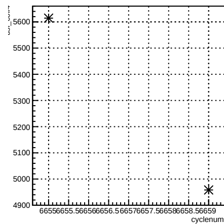
usl_coil4:cyclenum {run == 6621}
