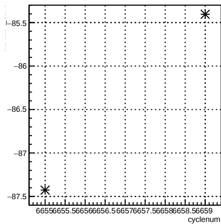
11X12X_coil3:cyclenum {run == 6621}
