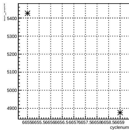
usr_coil4:cyclenum {run == 6621}
