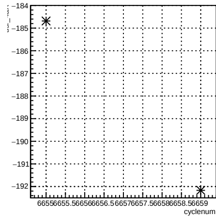
usr_4aX:cyclenum {run == 6621}
