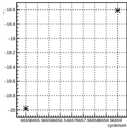
4eY_coil6:cyclenum {run == 6621}
