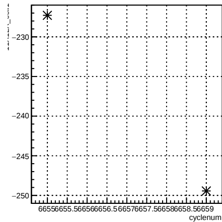
11X12X_coil1:cyclenum {run == 6621}
