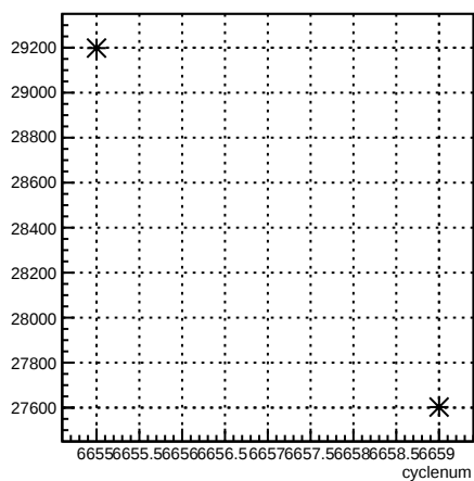
usl_coil7:cyclenum {run == 6621}
