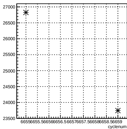
usr_coil7:cyclenum {run == 6621}
