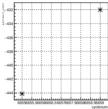
11X12X_coil7:cyclenum {run == 6621}
