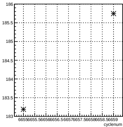
4aY_coil4:cyclenum {run == 6621}
