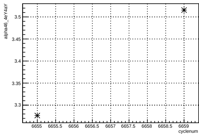
alpha46_4eY4aY:cyclenum {run == 6621}
