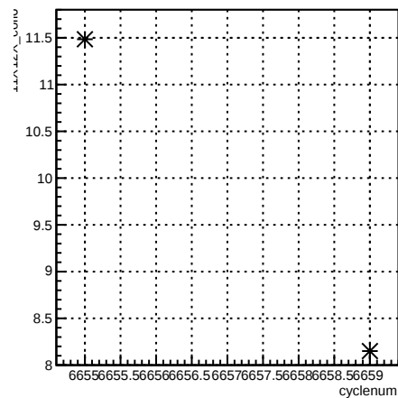
11X12X_coil6:cyclenum {run == 6621}
