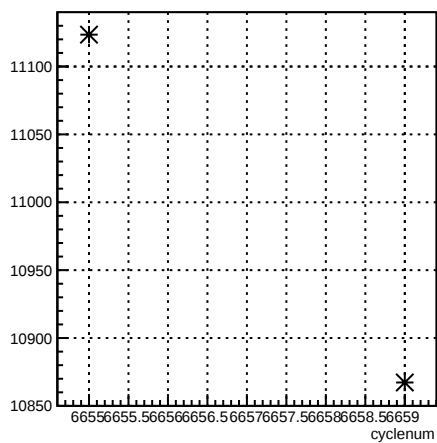
usl_coil3:cyclenum {run == 6621}
