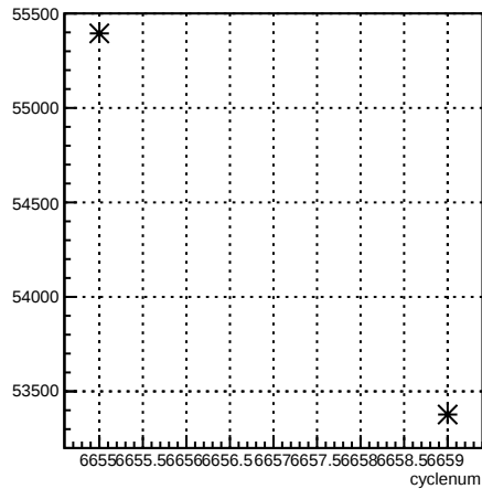
usl_coil1:cyclenum {run == 6621}
