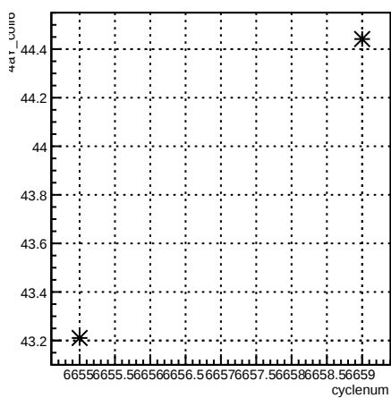
4aY_coil6:cyclenum {run == 6621}
