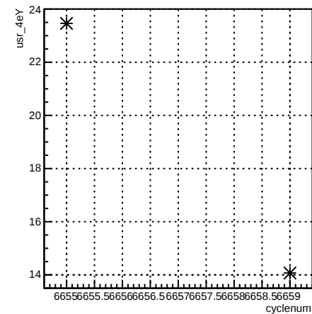
usr_4eY:cyclenum {run == 6621}
