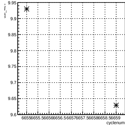
usl_4eY:cyclenum {run == 6621}
