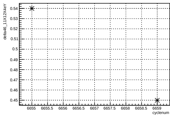
delta46_11X12X4eY:cyclenum {run == 6621}
