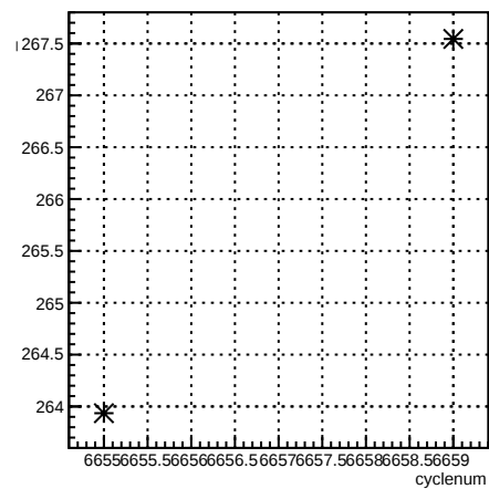
usr_4eX:cyclenum {run == 6621}
