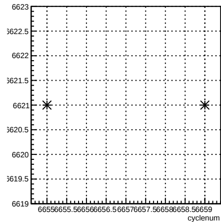
run:cyclenum {run == 6621}
