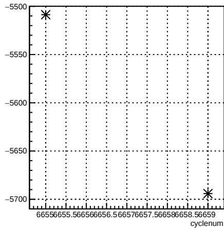
usr_coil3:cyclenum {run == 6621}
