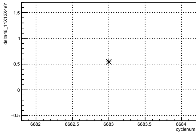
delta46_11X12X4eY:cyclenum {run == 6629}
