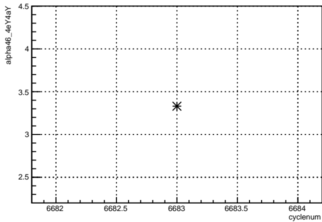
alpha46_4eY4aY:cyclenum {run == 6629}
