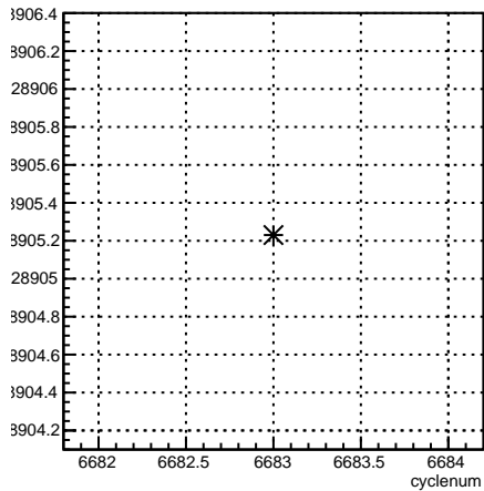
usl_coil7:cyclenum {run == 6629}
