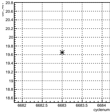
usr_4eY:cyclenum {run == 6629}
