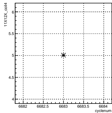
11X12X_coil4:cyclenum {run == 6629}
