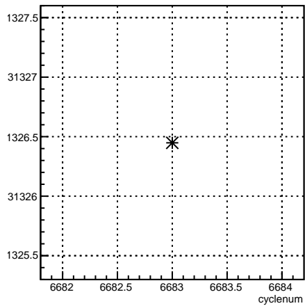
usl_coil6:cyclenum {run == 6629}
