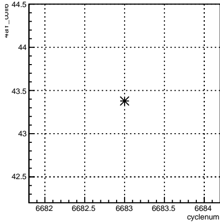
4eY_coil6:cyclenum {run == 6629}
