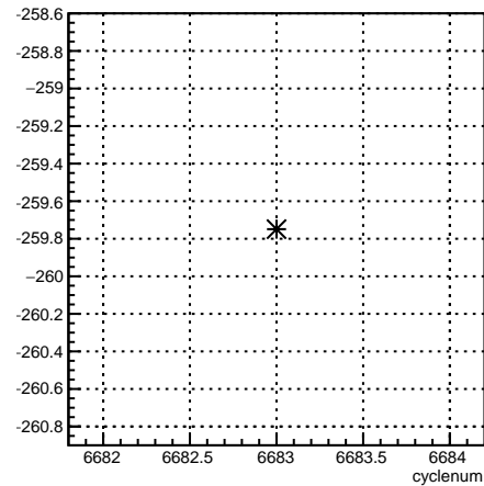
11X12X_coil1:cyclenum {run == 6629}
