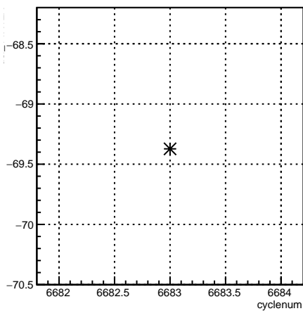
usl_11X12X:cyclenum {run == 6629}
