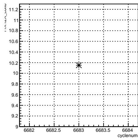
11X12X_coil6:cyclenum {run == 6629}
