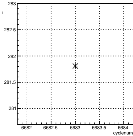
usr_4eX:cyclenum {run == 6629}
