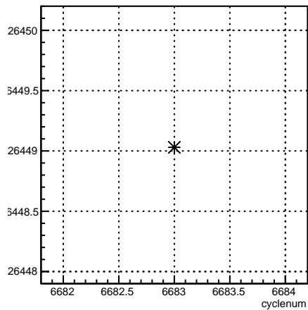
usr_coil7:cyclenum {run == 6629}
