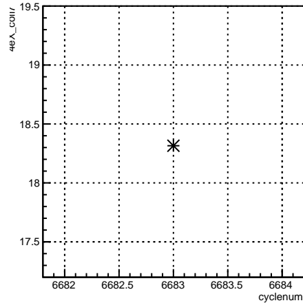
4eX_coil7:cyclenum {run == 6629}
