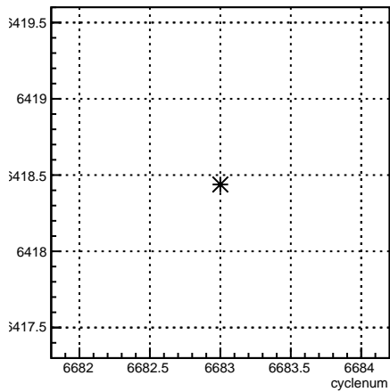
usl_coil7:cyclenum {run == 6629}
