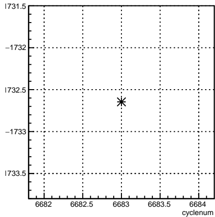
usl_coil6:cyclenum {run == 6629}
