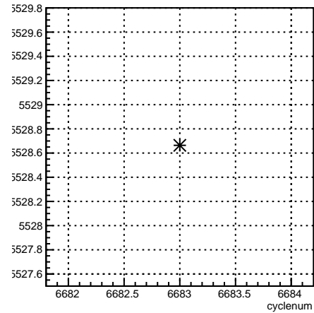
usr_coil4:cyclenum {run == 6629}
