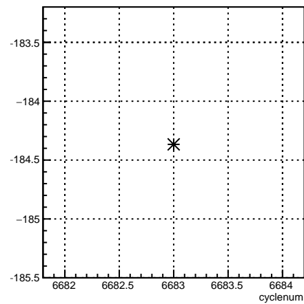
usl_4eY:cyclenum {run == 6629}
