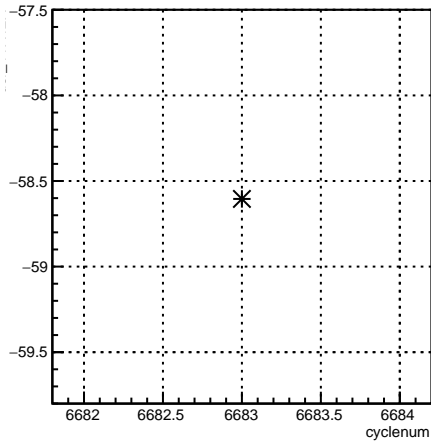
usr_11X12X:cyclenum {run == 6629}
