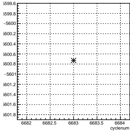
usr_coil3:cyclenum {run == 6629}
