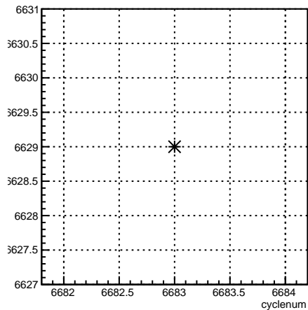
run:cyclenum {run == 6629}
