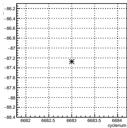
11X12X_coil3:cyclenum {run == 6629}
