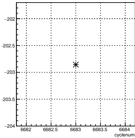
usr_4eY:cyclenum {run == 6629}
