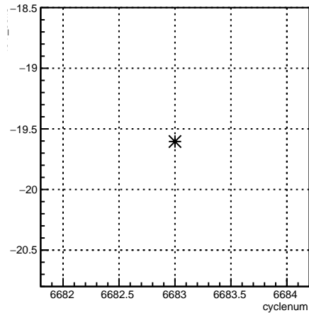
4eY_coil6:cyclenum {run == 6629}
