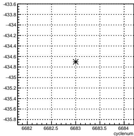
11X12X_coil7:cyclenum {run == 6629}
