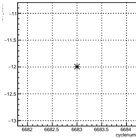
4eY_coil7:cyclenum {run == 6629}
