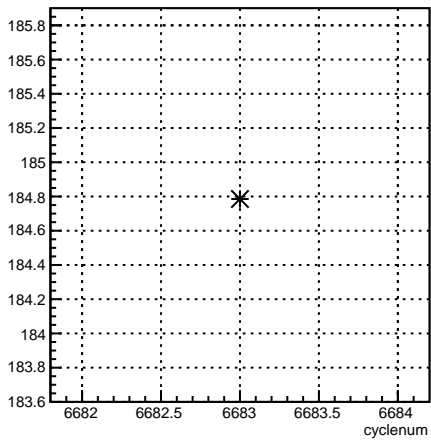
4eY_coil4:cyclenum {run == 6629}
