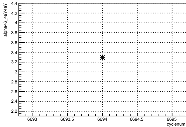
alpha46_4eY4aY:cyclenum {run == 6631}
