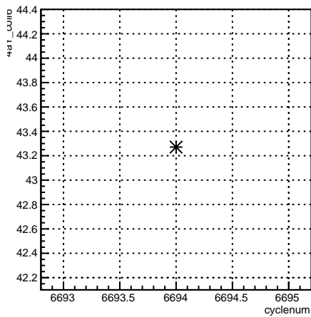
4aY_coil6:cyclenum {run == 6631}
