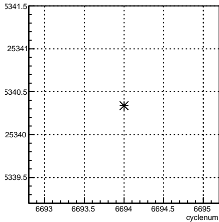
usl_coil7:cyclenum {run == 6631}
