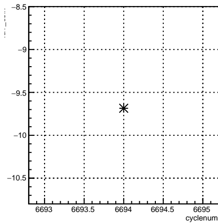
4aY_coil7:cyclenum {run == 6631}
