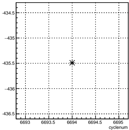
11X12X_coil7:cyclenum {run == 6631}
