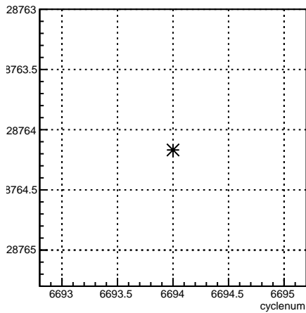
usr_coil1:cyclenum {run == 6631}
