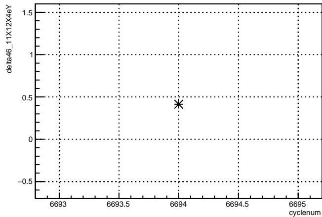
delta46_11X12X4eY:cyclenum {run == 6631}
