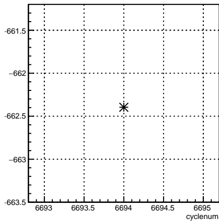
usr_coil6:cyclenum {run == 6631}
