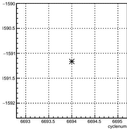
usl_coil6:cyclenum {run == 6631}
