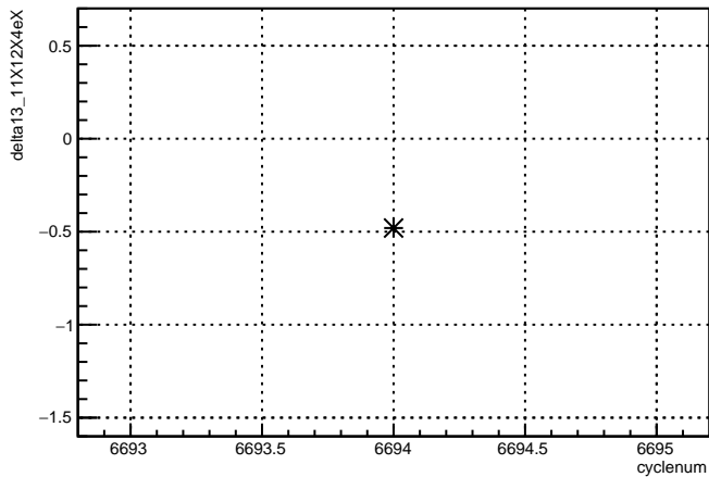
delta13_11X12X4eX:cyclenum {run == 6631}
