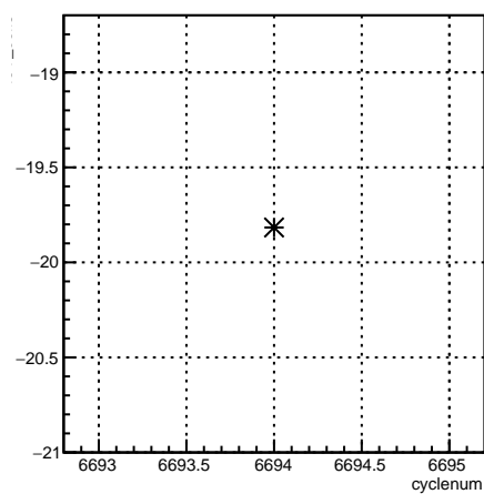
4eY_coil6:cyclenum {run == 6631}
