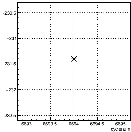
11X12X_coil6:cyclenum {run == 6631}
