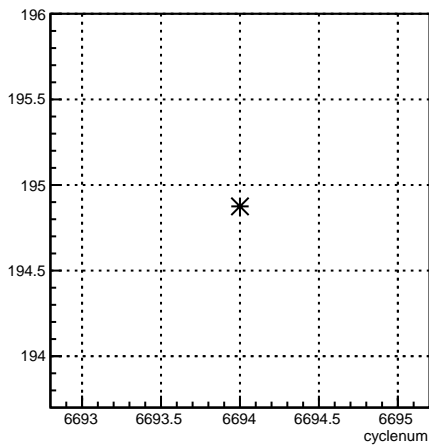
4eY_coil4:cyclenum {run == 6631}
