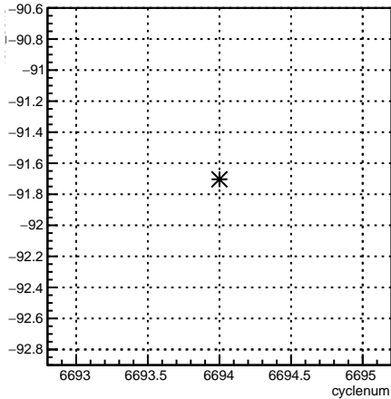
4eX_coil3:cyclenum {run == 6631}
