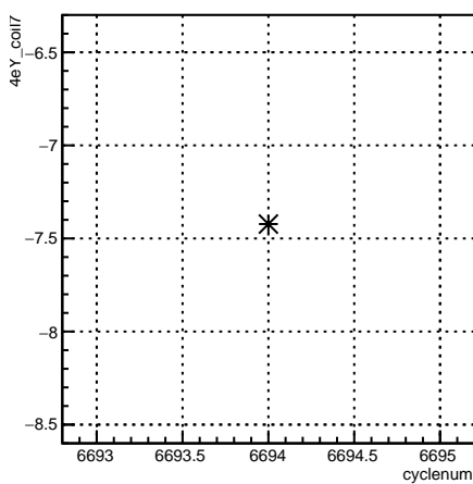
4eY_coil7:cyclenum {run == 6631}
