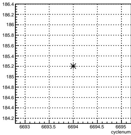
4aY_coil4:cyclenum {run == 6631}
