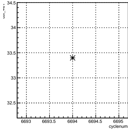
usl_4eY:cyclenum {run == 6631}
