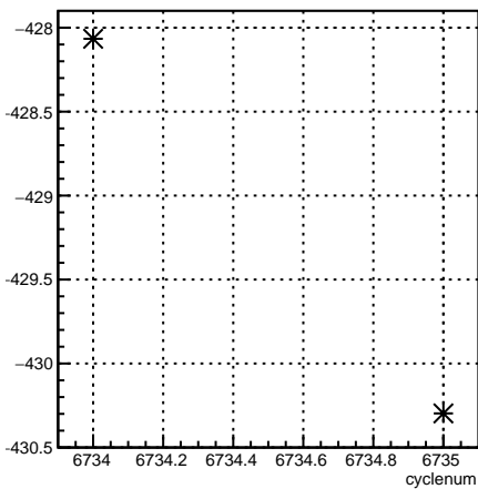
11X12X_coil7:cyclenum {run == 6645}
