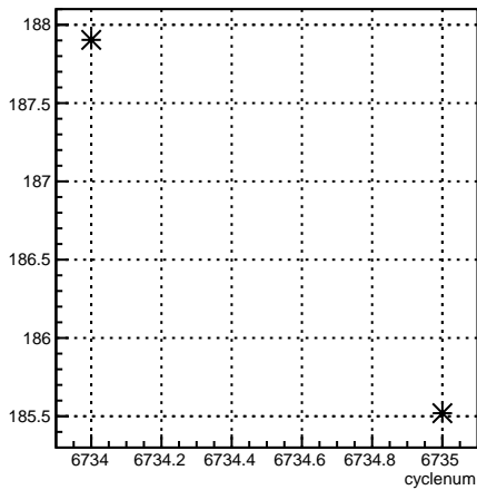
4eY_coil4:cyclenum {run == 6645}
