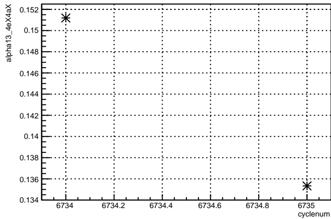
alpha13_4eX4aX:cyclenum {run == 6645}
