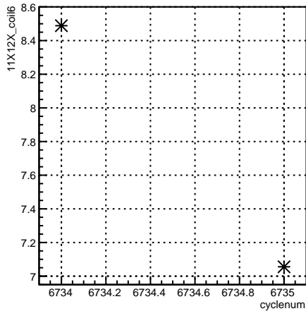
11X12X_coil6:cyclenum {run == 6645}
