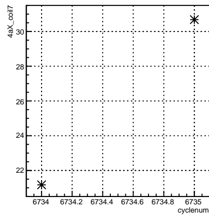
4aX_coil7:cyclenum {run == 6645}
