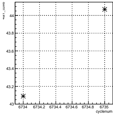
4eY_coil6:cyclenum {run == 6645}
