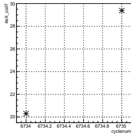
4eX_coil7:cyclenum {run == 6645}
