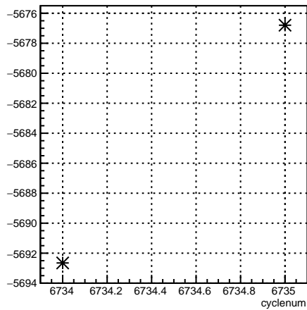
usr_coil7:cyclenum {run == 6645}
