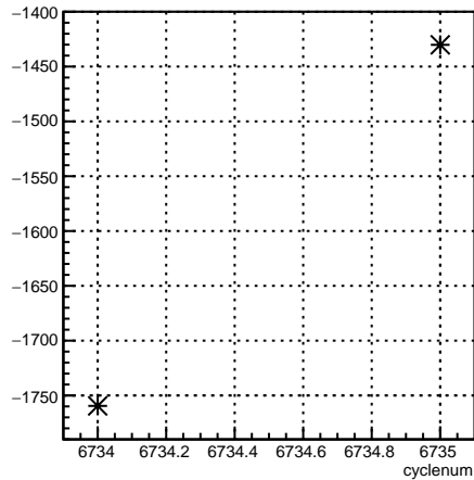
usl_coil6:cyclenum {run == 6645}
