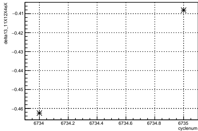
delta13_11X12X4eX:cyclenum {run == 6645}
