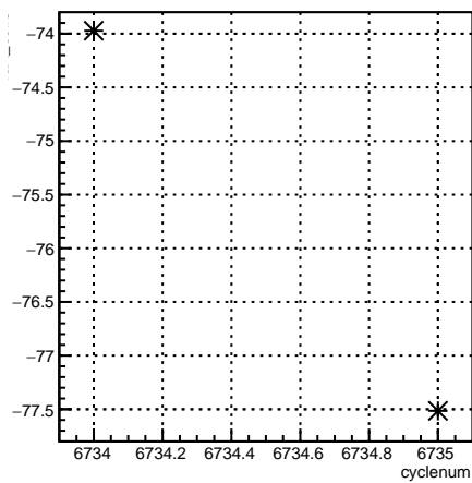
4aX_coil3:cyclenum {run == 6645}
