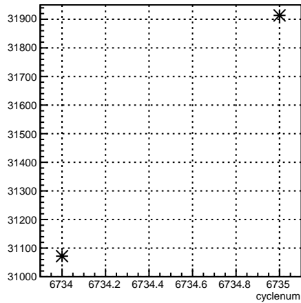
usl_coil6:cyclenum {run == 6645}
