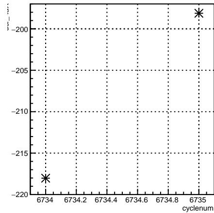
usr_4eY:cyclenum {run == 6645}
