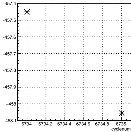
4aX_coil1:cyclenum {run == 6645}
