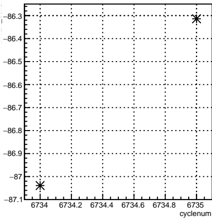
11X12X_coil3:cyclenum {run == 6645}
