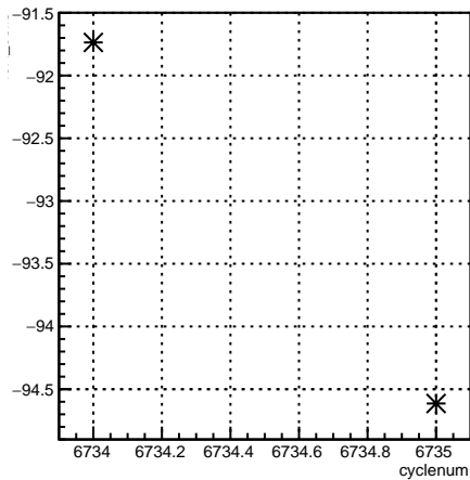
4eX_coil3:cyclenum {run == 6645}
