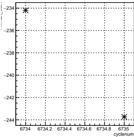
11X12X_coil1:cyclenum {run == 6645}
