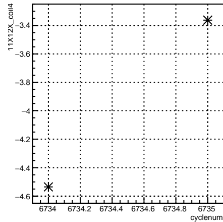
11X12X_coil4:cyclenum {run == 6645}
