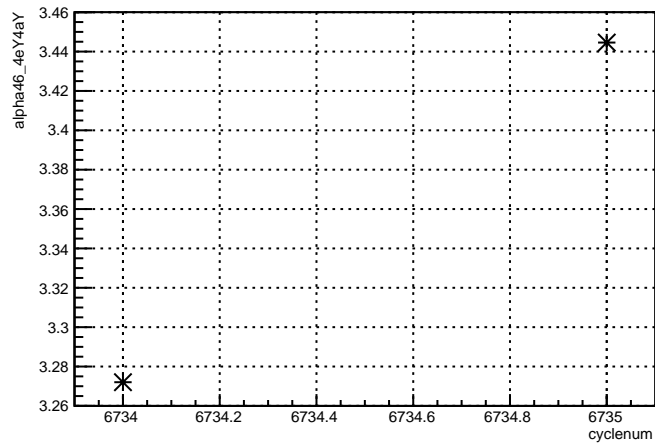
alpha46_4eY4aY:cyclenum {run == 6645}
