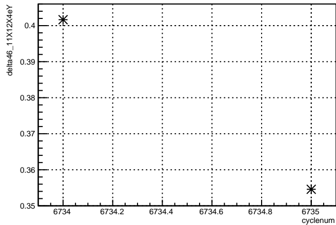
delta46_11X12X4eY:cyclenum {run == 6645}
