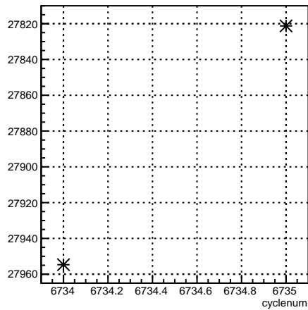
usr_coil6:cyclenum {run == 6645}
