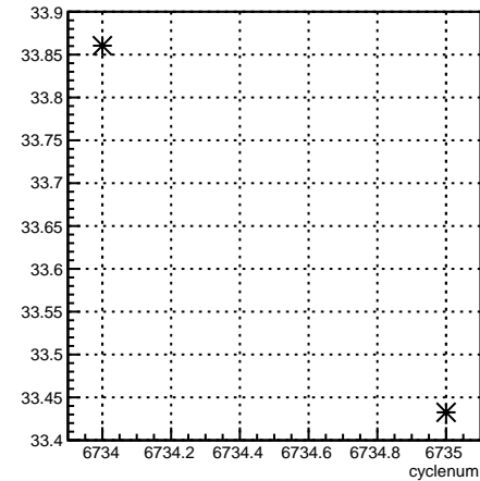
usl_4eY:cyclenum {run == 6645}
