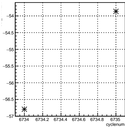
usr_11X12X:cyclenum {run == 6645}
