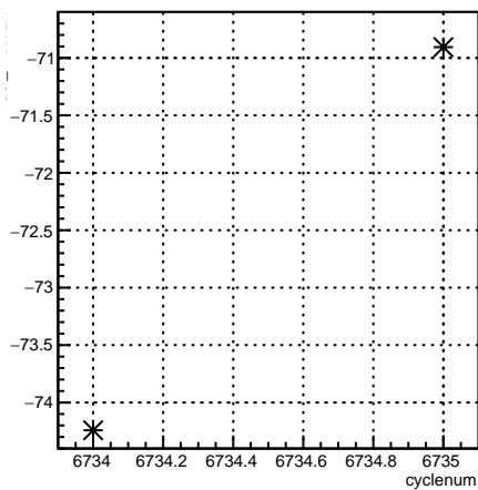
usl_11X12X:cyclenum {run == 6645}
