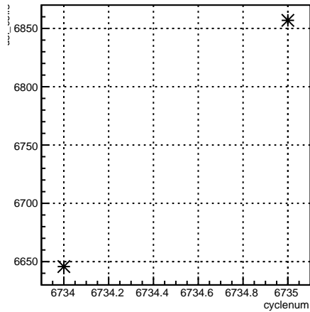
usl_coil7:cyclenum {run == 6645}
