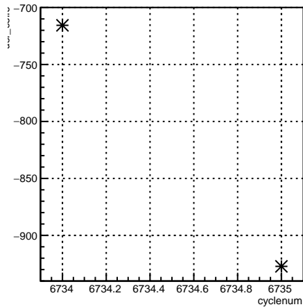
usr_coil6:cyclenum {run == 6645}
