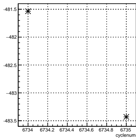
4eX_coil1:cyclenum {run == 6645}
