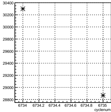
usl_coil7:cyclenum {run == 6645}
