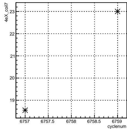
4eX_coil7:cyclenum {run == 6663}
