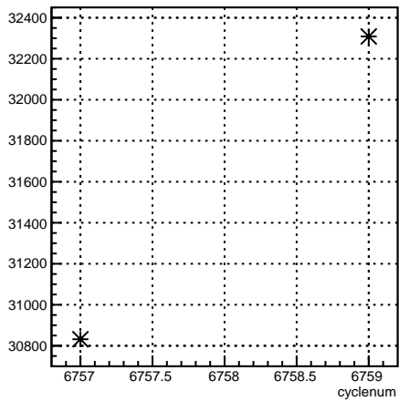
usl_coil6:cyclenum {run == 6663}
