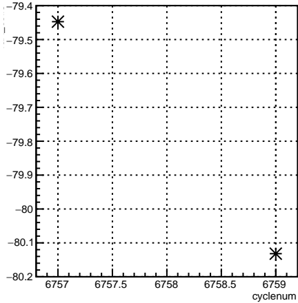
4eX_coil3:cyclenum {run == 6663}
