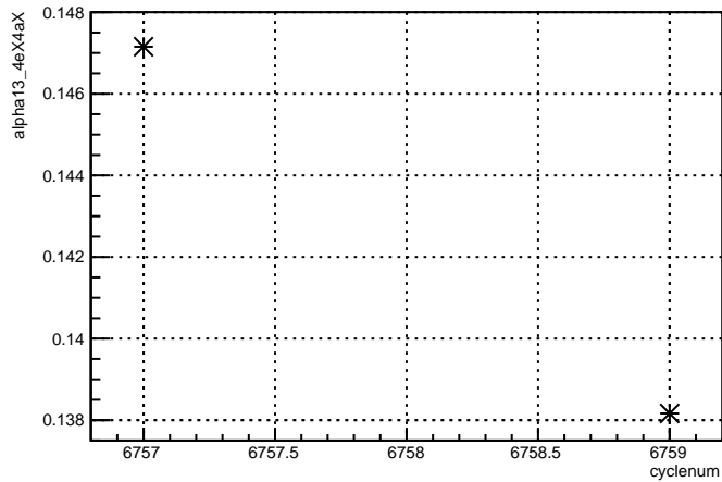
alpha13_4eX4aX:cyclenum {run == 6663}
