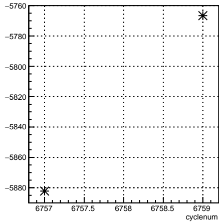
usr_coil3:cyclenum {run == 6663}
