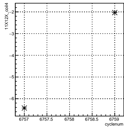
11X12X_coil4:cyclenum {run == 6663}
