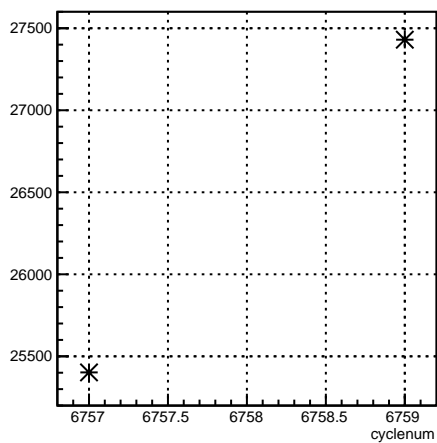
usr_coil7:cyclenum {run == 6663}
