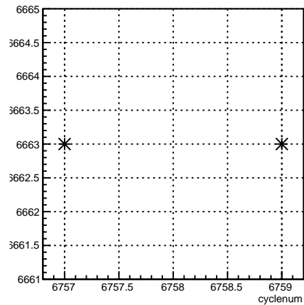
run:cyclenum {run == 6663}
