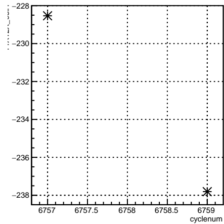
11X12X_coil1:cyclenum {run == 6663}
