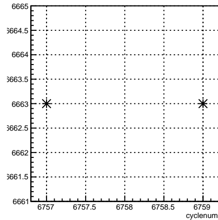
run:cyclenum {run == 6663}
