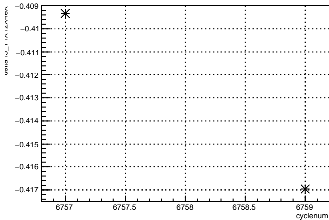
delta13_11X12X4eX:cyclenum {run == 6663}
