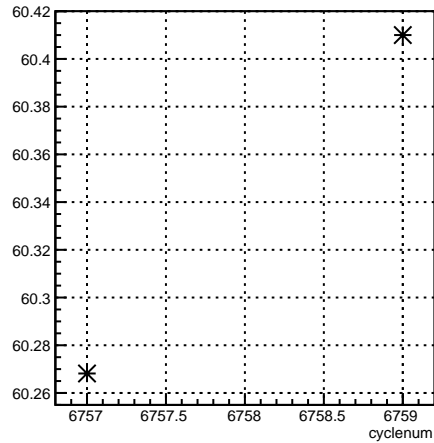
4aY_coil6:cyclenum {run == 6663}
