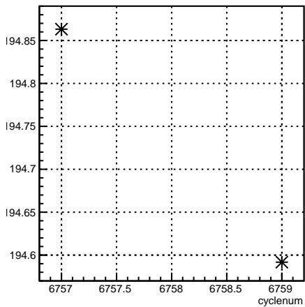
4eY_coil4:cyclenum {run == 6663}
