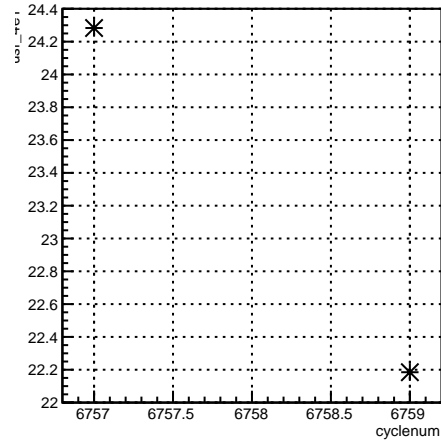
usr_4eY:cyclenum {run == 6663}
