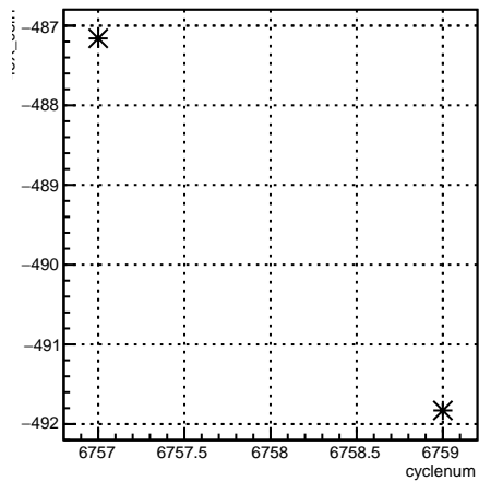
4eX_coil1:cyclenum {run == 6663}
