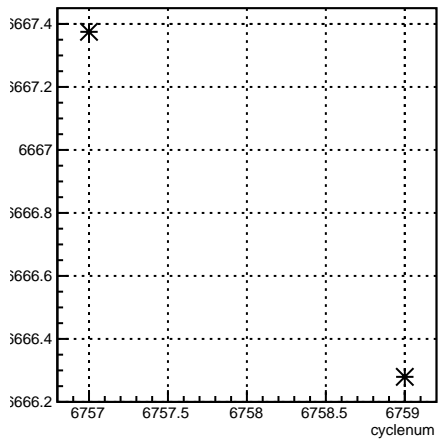
usl_coil7:cyclenum {run == 6663}
