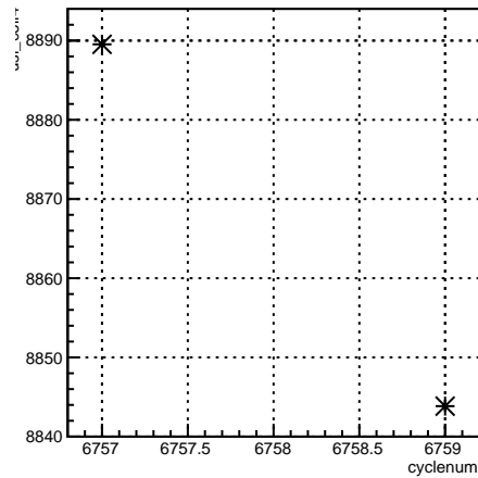
run:cyclenum {run == 6663}
