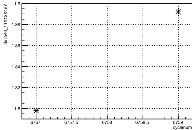
delta46_11X12X4eY:cyclenum {run == 6663}
