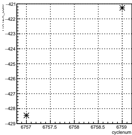
11X12X_coil7:cyclenum {run == 6663}
