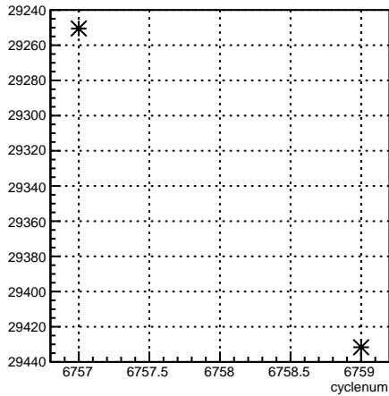
usr_coil1:cyclenum {run == 6663}
