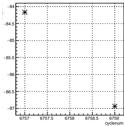
11X12X_coil3:cyclenum {run == 6663}
