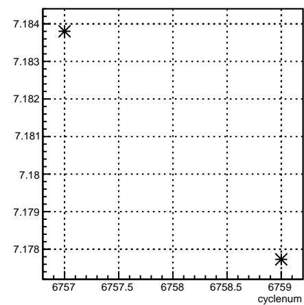
11X12X_coil6:cyclenum {run == 6663}
