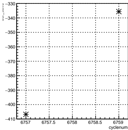
usr_coil6:cyclenum {run == 6663}
