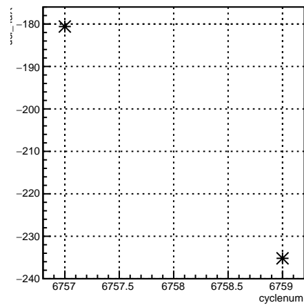
usl_4eY:cyclenum {run == 6663}
