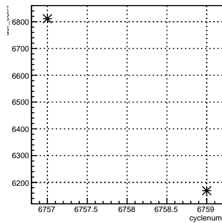
usr_coil4:cyclenum {run == 6663}
