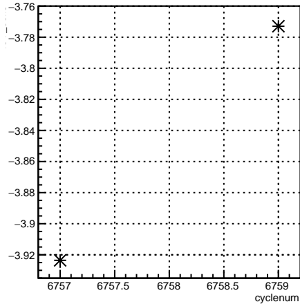
4eY_coil6:cyclenum {run == 6663}
