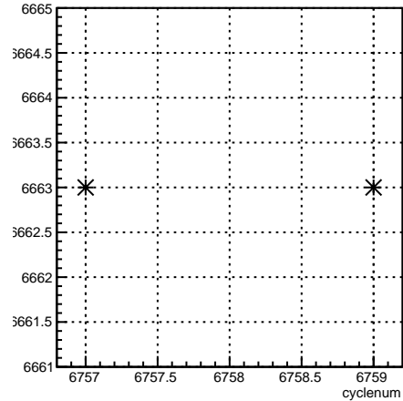
run:cyclenum {run == 6663}
