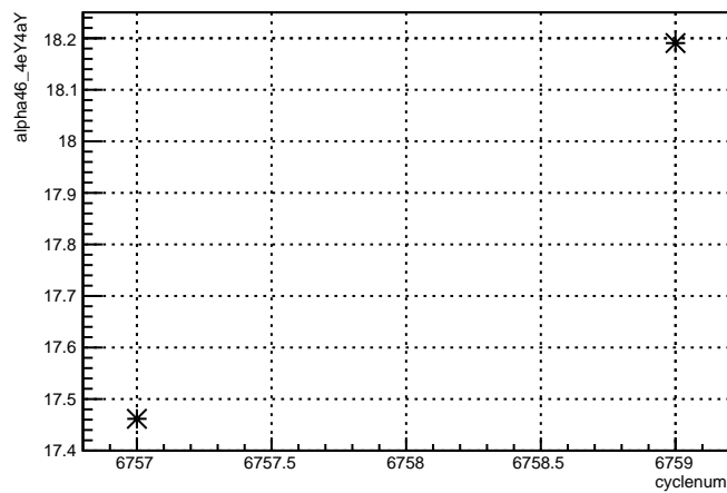
alpha46_4eY4aY:cyclenum {run == 6663}
