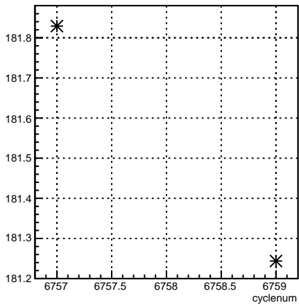
4eY_coil4:cyclenum {run == 6663}
