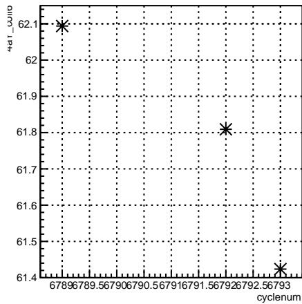
4eY_coil6:cyclenum {run == 6670}
