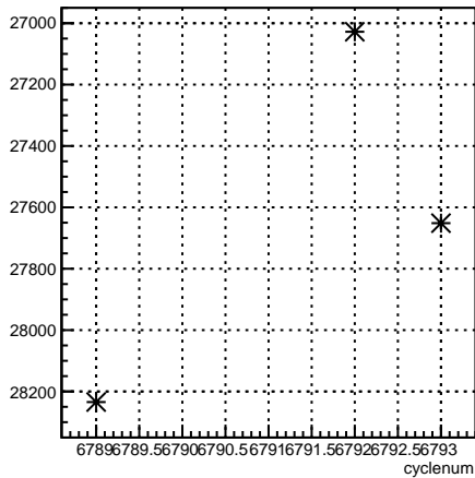
usr_coil6:cyclenum {run == 6670}
