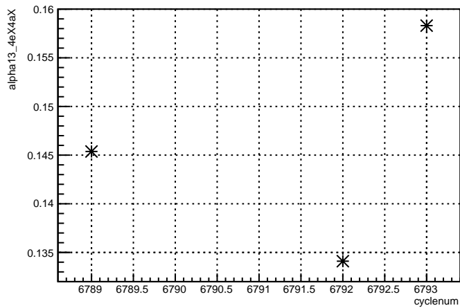
alpha13_4eX4aX:cyclenum {run == 6670}
