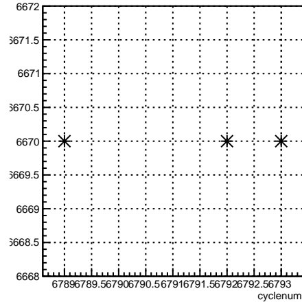
run:cyclenum {run == 6670}
