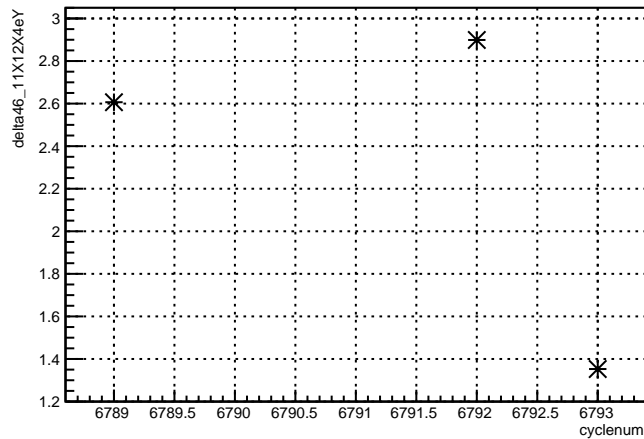
delta46_11X12X4eY:cyclenum {run == 6670}
