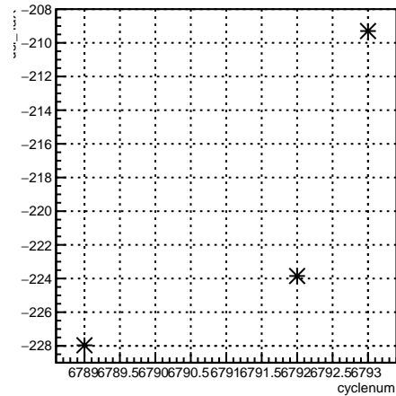
usl_4eY:cyclenum {run == 6670}
