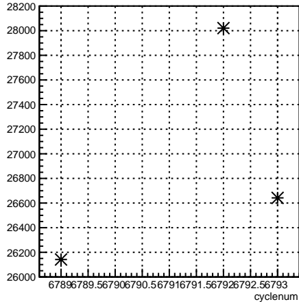
usr_coil7:cyclenum {run == 6670}
