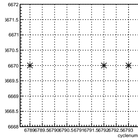
run:cyclenum {run == 6670}
