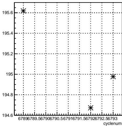
4eY_coil4:cyclenum {run == 6670}
