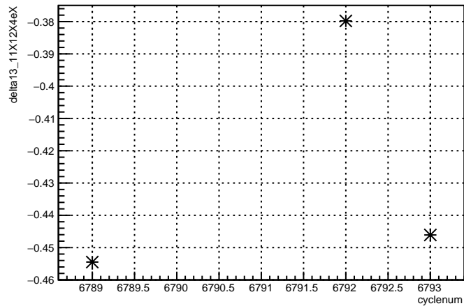
delta13_11X12X4eX:cyclenum {run == 6670}
