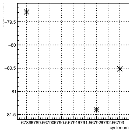
usl_11X12X:cyclenum {run == 6670}
