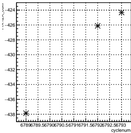
11X12X_coil7:cyclenum {run == 6670}
