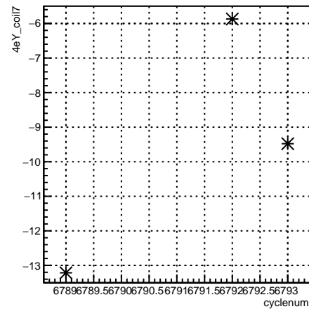
4eY_coil7:cyclenum {run == 6670}
