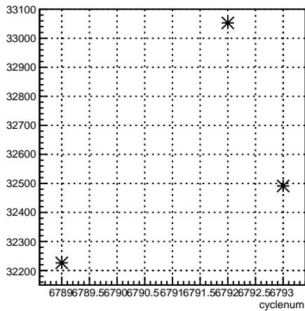
usl_coil1:cyclenum {run == 6670}
