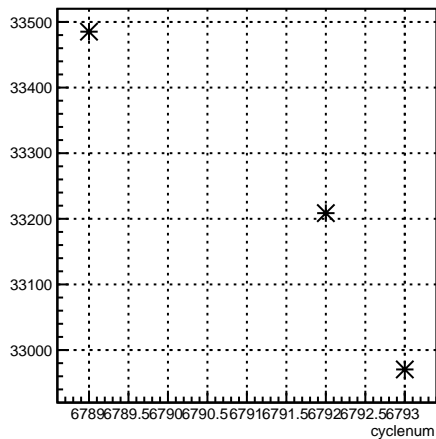
usl_coil7:cyclenum {run == 6670}
