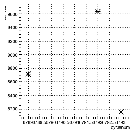
usl_coil4:cyclenum {run == 6670}
