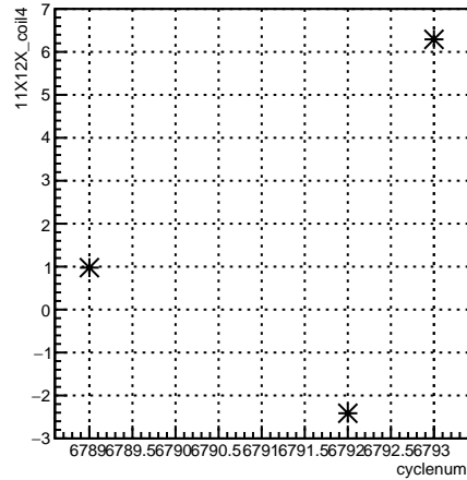
11X12X_coil4:cyclenum {run == 6670}
