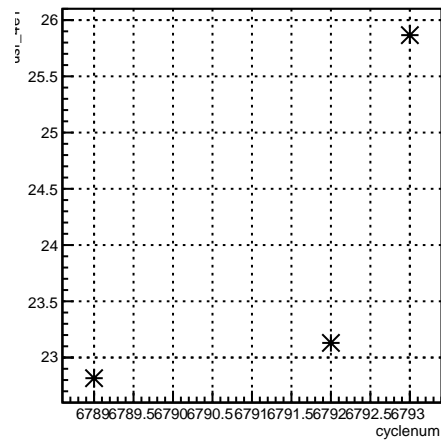
usr_4eY:cyclenum {run == 6670}
