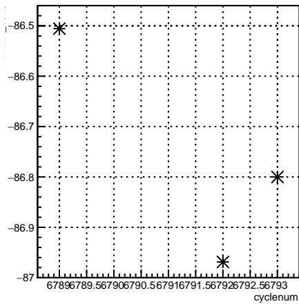
11X12X_coil3:cyclenum {run == 6670}
