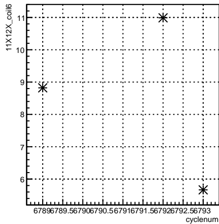
11X12X_coil6:cyclenum {run == 6670}
