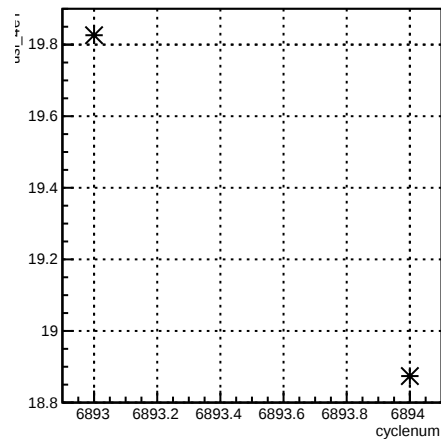
usl_4eY:cyclenum {run == 6755}
