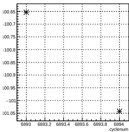
4eX_coil3:cyclenum {run == 6755}
