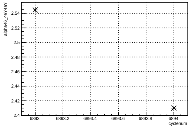
alpha46_4eY4aY:cyclenum {run == 6755}
