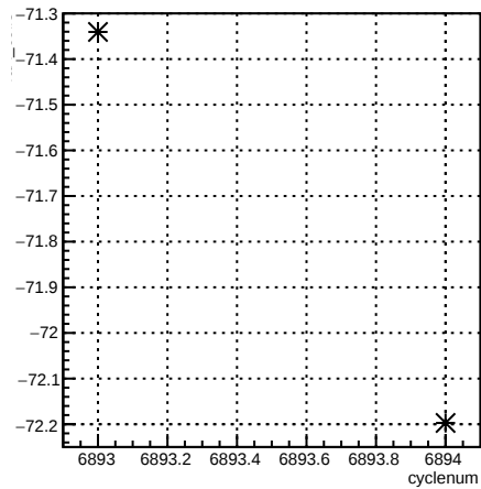
4aX_coil3:cyclenum {run == 6755}
