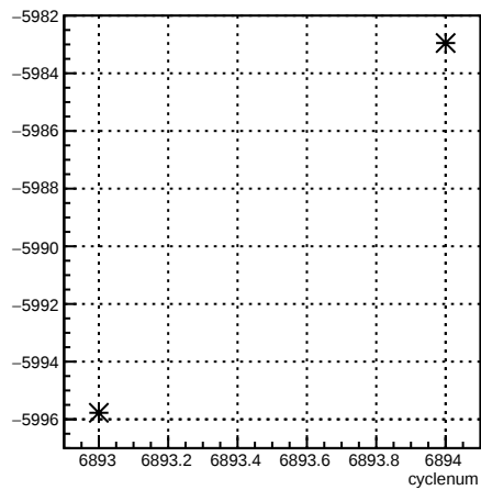
usr_coil3:cyclenum {run == 6755}
