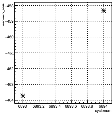
11X12X_coil7:cyclenum {run == 6755}
