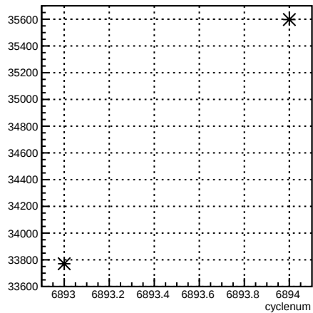
usl_coil6:cyclenum {run == 6755}
