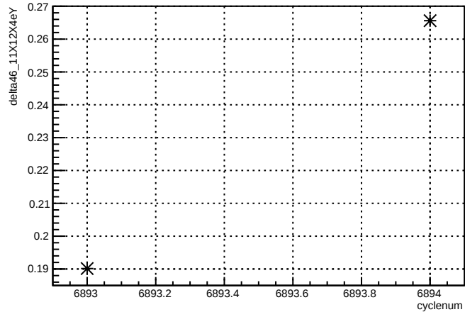
delta46_11X12X4eY:cyclenum {run == 6755}
