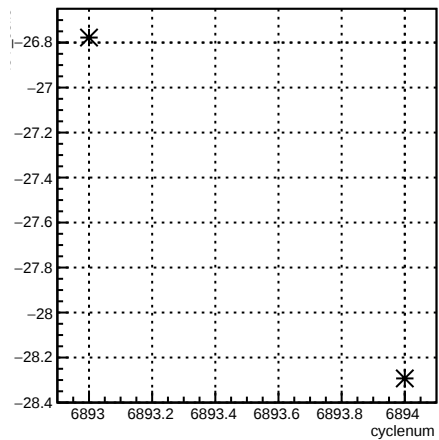
4eY_coil6:cyclenum {run == 6755}
