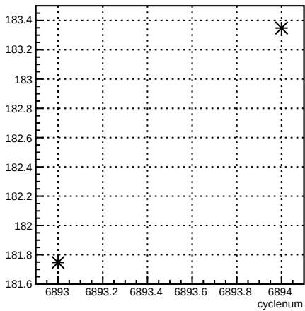
4eY_coil4:cyclenum {run == 6755}
