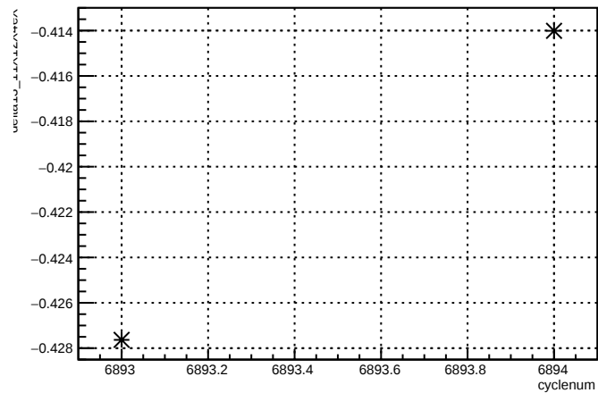
delta13_11X12X4eX:cyclenum {run == 6755}
