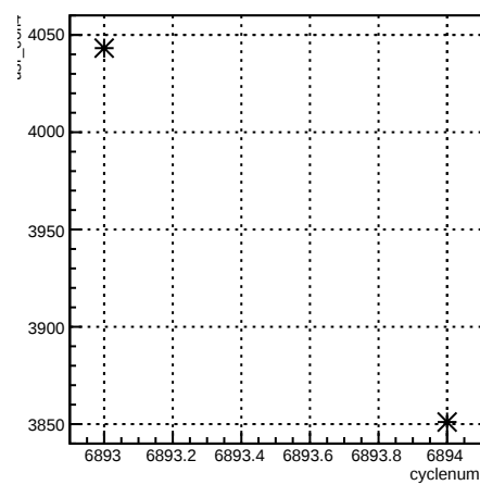
usr_coil4:cyclenum {run == 6755}
