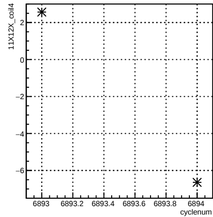
run:cyclenum {run == 6755}
