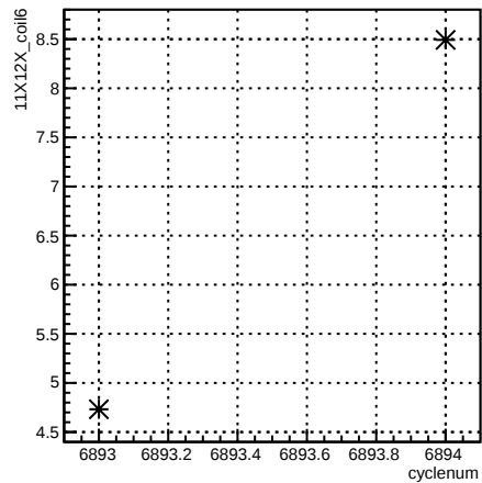
11X12X_coil6:cyclenum {run == 6755}
