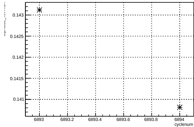
alpha13_4eX4aX:cyclenum {run == 6755}
