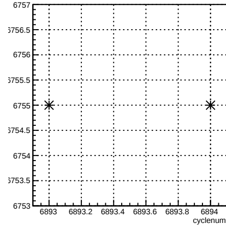
run:cyclenum {run == 6755}
