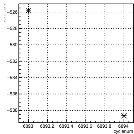
4eX_coil1:cyclenum {run == 6755}
