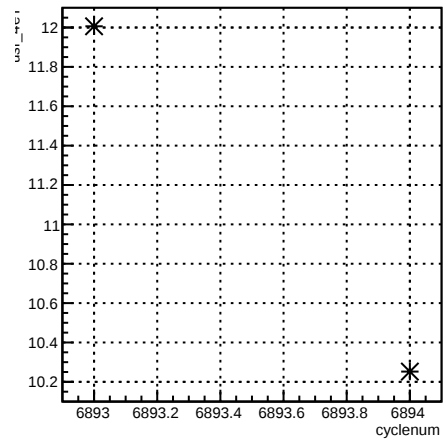
usr_4eY:cyclenum {run == 6755}
