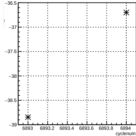
usl_11X12X:cyclenum {run == 6755}
