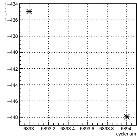
4aX_coil1:cyclenum {run == 6755}
