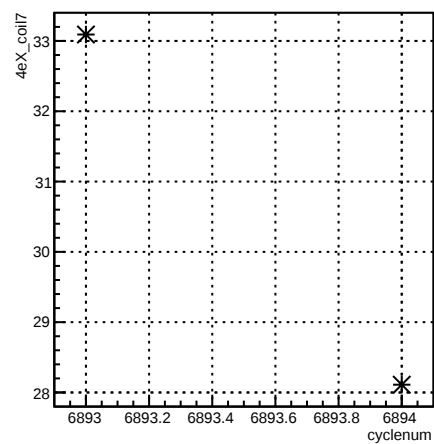
4eX_coil7:cyclenum {run == 6755}
