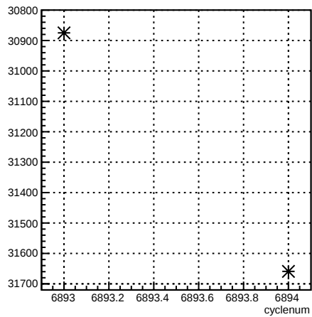
usr_coil1:cyclenum {run == 6755}
