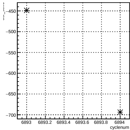
usr_coil6:cyclenum {run == 6755}
