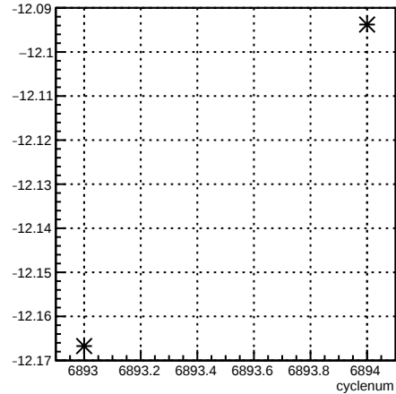
4eY_coil7:cyclenum {run == 6755}
