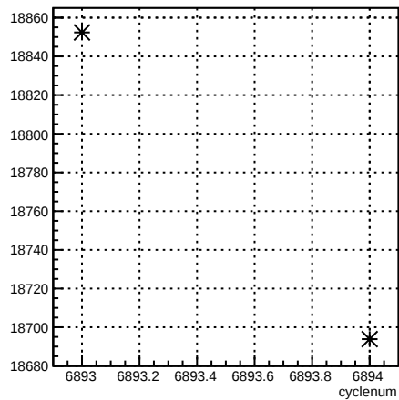
usr_coil7:cyclenum {run == 6755}
