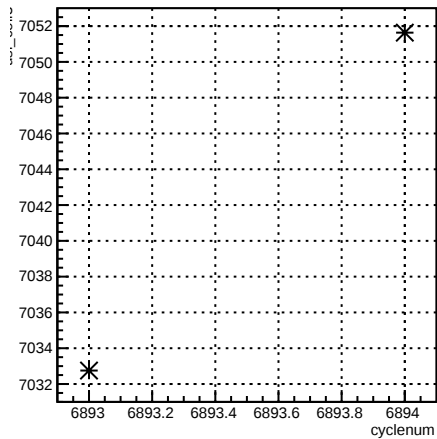
usl_coil7:cyclenum {run == 6755}
