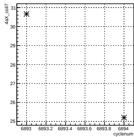
4aX_coil7:cyclenum {run == 6755}
