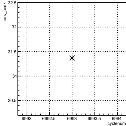
4eX_coil7:cyclenum {run == 6797}
