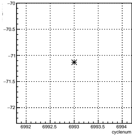
4aX_coil3:cyclenum {run == 6797}
