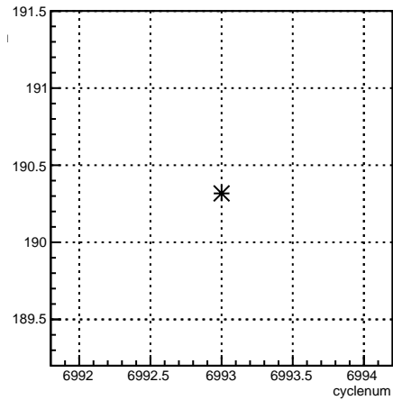
usr_4eX:cyclenum {run == 6797}
