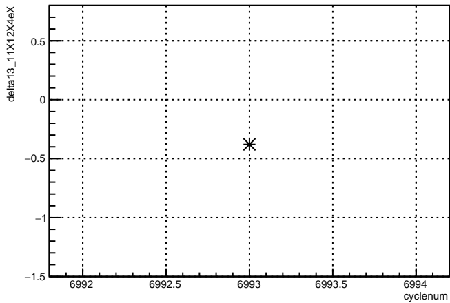
delta13_11X12X4eX:cyclenum {run == 6797}
