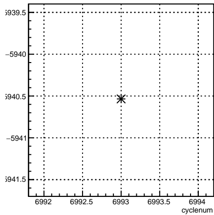
usr_coil7:cyclenum {run == 6797}
