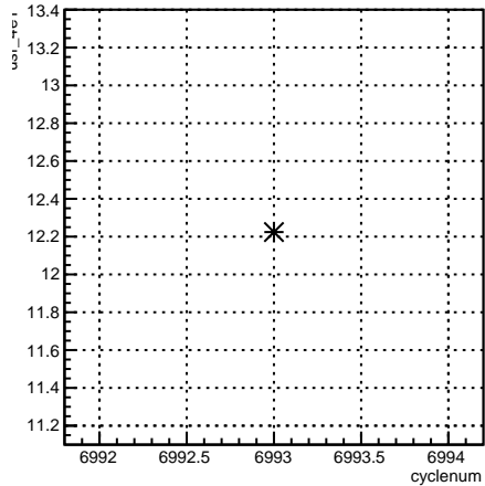
usr_4eY:cyclenum {run == 6797}
