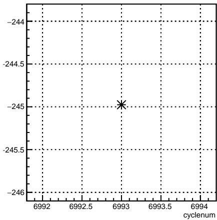
11X12X_coil1:cyclenum {run == 6797}
