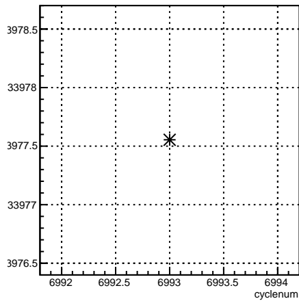
usl_coil6:cyclenum {run == 6797}
