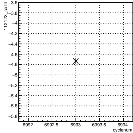
11X12X_coil4:cyclenum {run == 6797}
