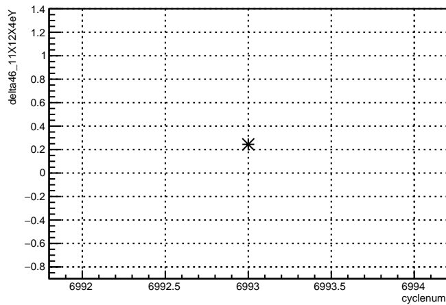
delta46_11X12X4eY:cyclenum {run == 6797}
