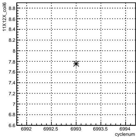
11X12X_coil6:cyclenum {run == 6797}
