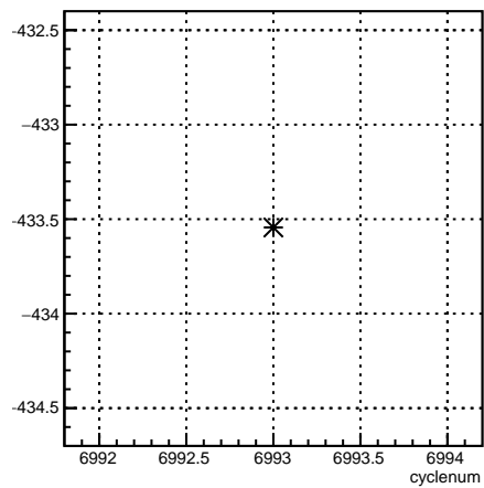
4aX_coil1:cyclenum {run == 6797}
