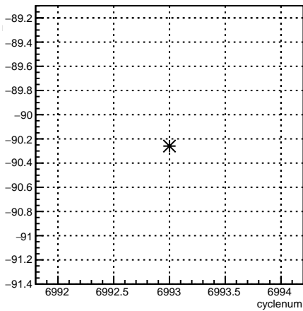
usl_4eY:cyclenum {run == 6797}
