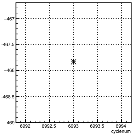
11X12X_coil7:cyclenum {run == 6797}
