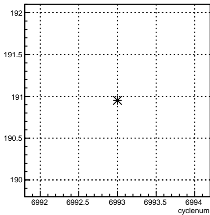
4eY_coil4:cyclenum {run == 6797}
