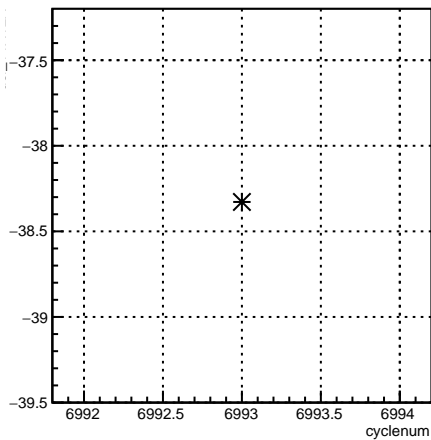
usl_11X12X:cyclenum {run == 6797}
