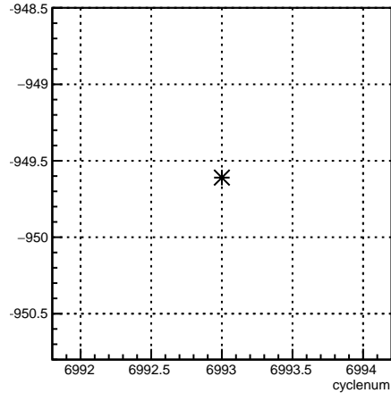
usr_coil6:cyclenum {run == 6797}
