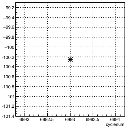
4eX_coil3:cyclenum {run == 6797}
