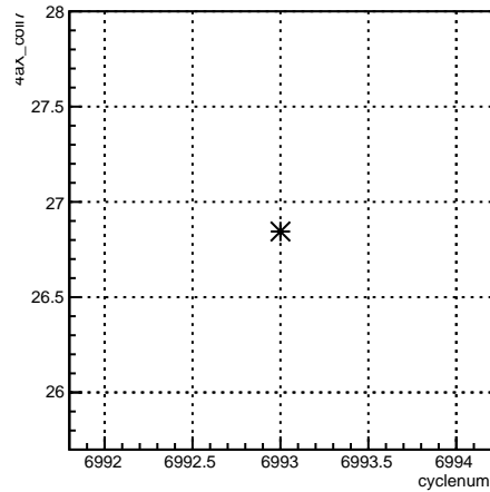
4aX_coil7:cyclenum {run == 6797}
