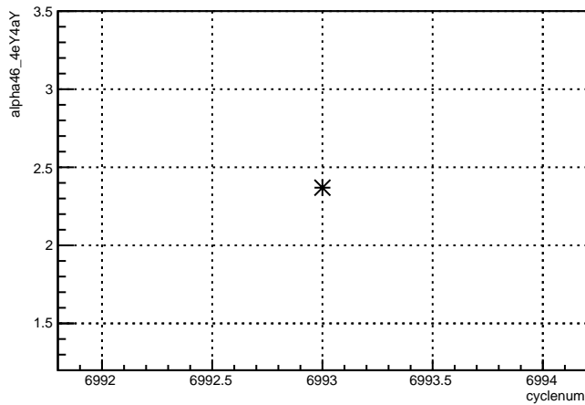
alpha46_4eY4aY:cyclenum {run == 6797}
