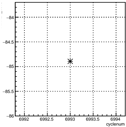
11X12X_coil3:cyclenum {run == 6797}
