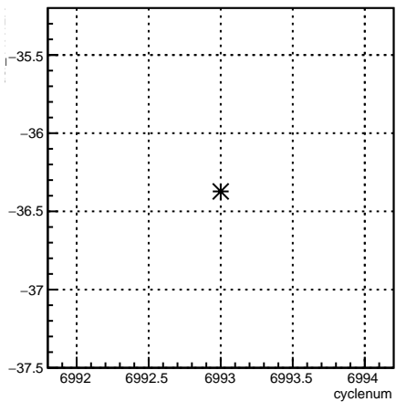
usr_11X12X:cyclenum {run == 6797}
