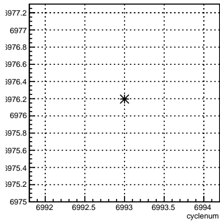
usl_coil7:cyclenum {run == 6797}
