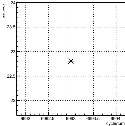
usl_4eY:cyclenum {run == 6797}
