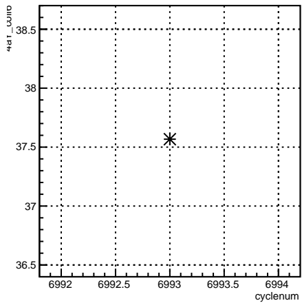
4eY_coil6:cyclenum {run == 6797}
