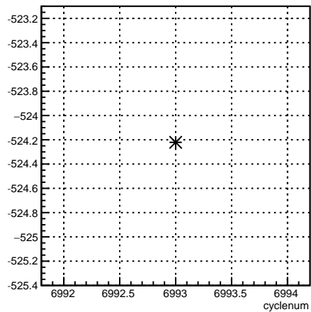
4eX_coil1:cyclenum {run == 6797}
