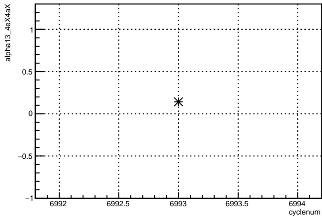
alpha13_4eX4aX:cyclenum {run == 6797}
