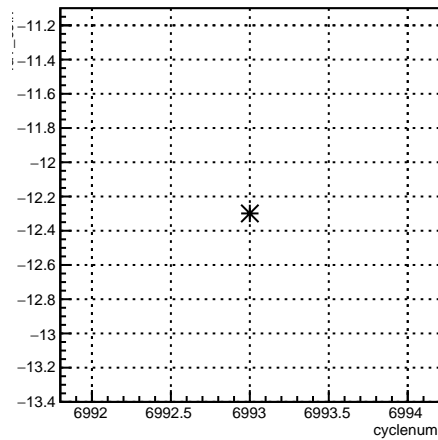
4eY_coil7:cyclenum {run == 6797}
