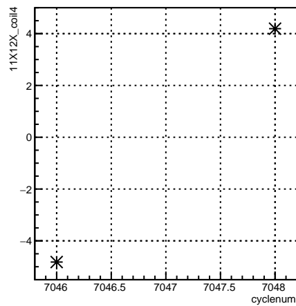
11X12X_coil4:cyclenum {run == 6808}
