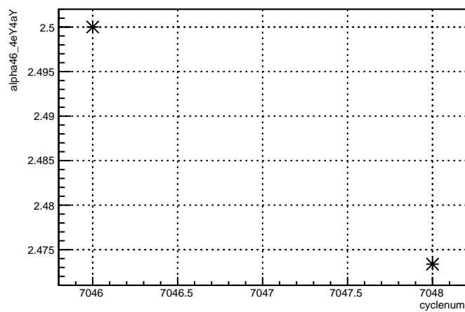
alpha46_4eY4aY:cyclenum {run == 6808}
