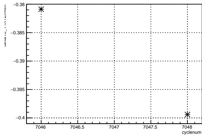
delta13_11X12X4eX:cyclenum {run == 6808}
