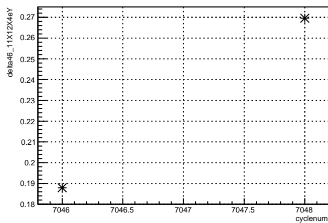
delta46_11X12X4eY:cyclenum {run == 6808}
