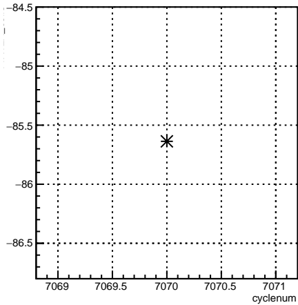
11X12X_coil3:cyclenum {run == 6813}
