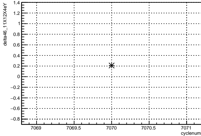
delta46_11X12X4eY:cyclenum {run == 6813}
