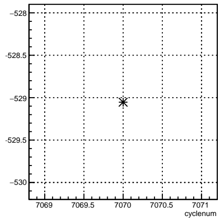
4eX_coil1:cyclenum {run == 6813}
