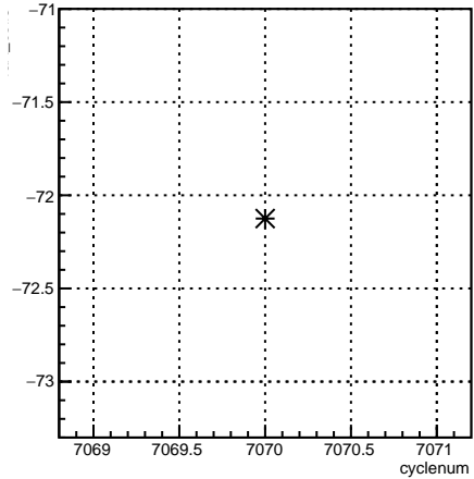
4eX_coil3:cyclenum {run == 6813}
