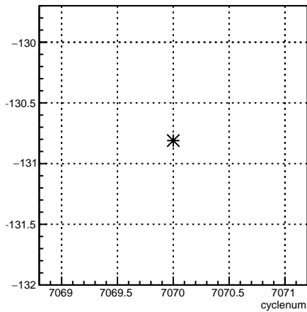
usr_4eY:cyclenum {run == 6813}
