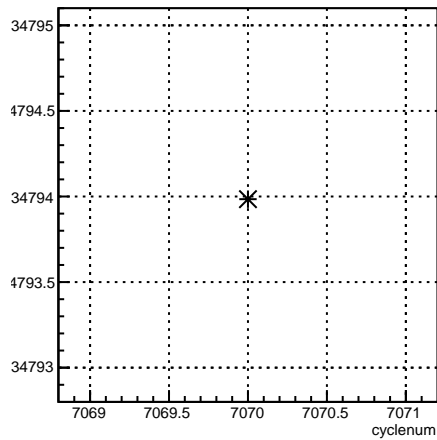
usl_coil6:cyclenum {run == 6813}
