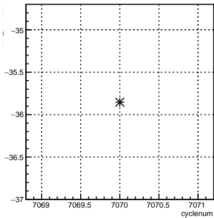
usr_11X12X:cyclenum {run == 6813}
