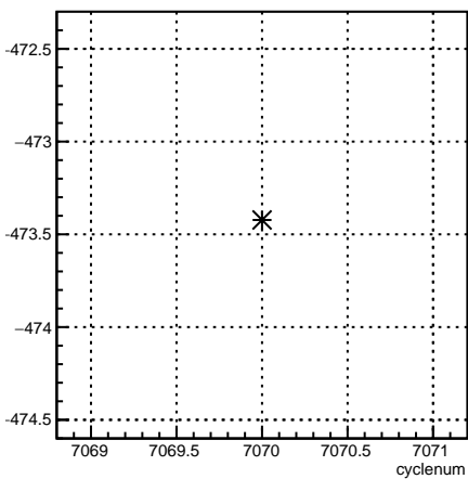
11X12X_coil7:cyclenum {run == 6813}
