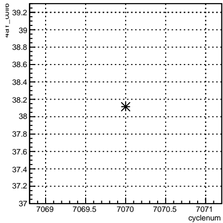
4eY_coil6:cyclenum {run == 6813}
