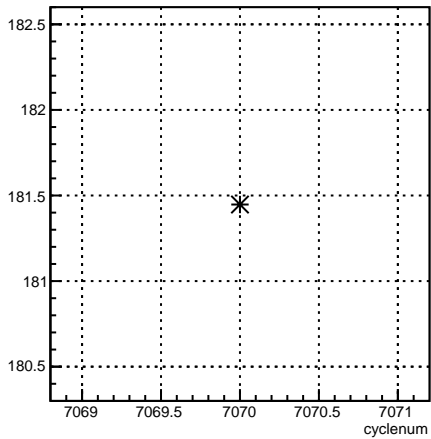
4eY_coil4:cyclenum {run == 6813}
