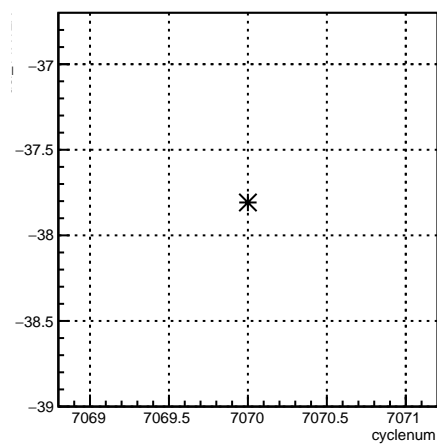
usl_11X12X:cyclenum {run == 6813}
