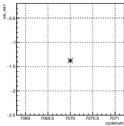
usl_4aY:cyclenum {run == 6813}
