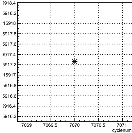
usl_coil7:cyclenum {run == 6813}
