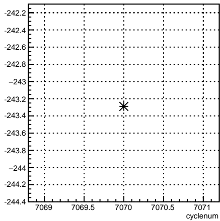
11X12X_coil1:cyclenum {run == 6813}
