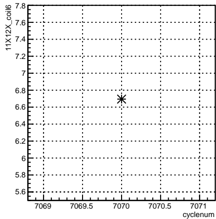
11X12X_coil6:cyclenum {run == 6813}
