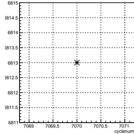
run:cyclenum {run == 6813}
