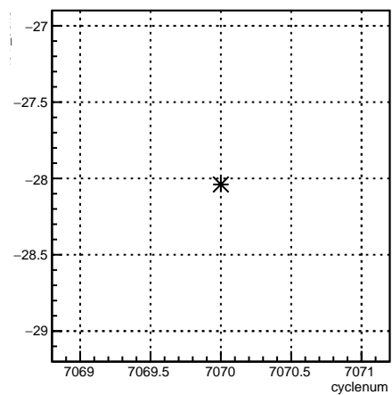
4eY_coil6:cyclenum {run == 6813}
