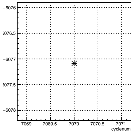
usr_coil7:cyclenum {run == 6813}
