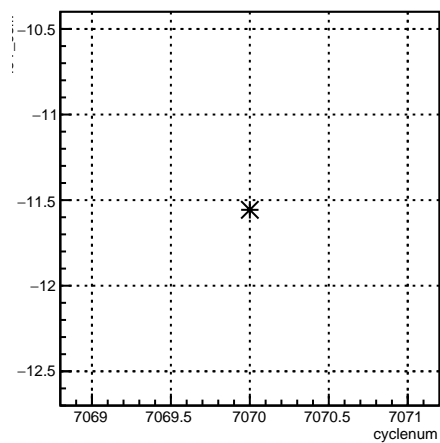
4eY_coil7:cyclenum {run == 6813}
