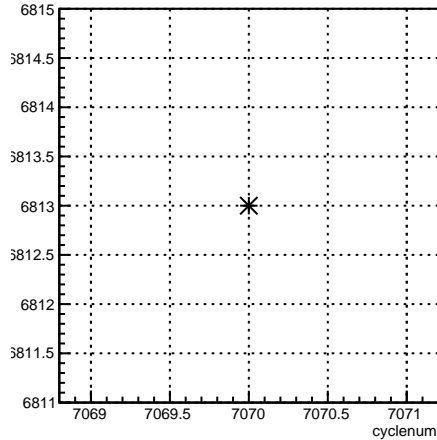
run:cyclenum {run == 6813}
