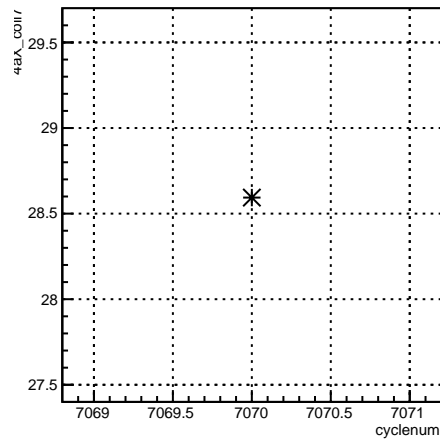
4eX_coil7:cyclenum {run == 6813}
