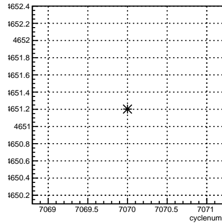
usl_coil4:cyclenum {run == 6813}
