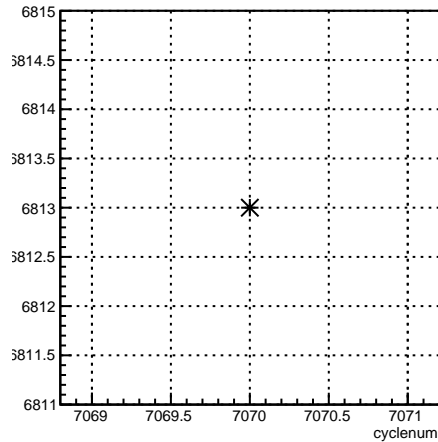
run:cyclenum {run == 6813}
