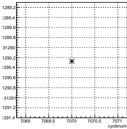
usr_coil6:cyclenum {run == 6813}
