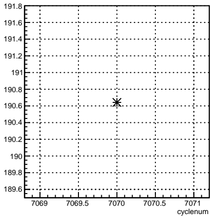
4eY_coil4:cyclenum {run == 6813}
