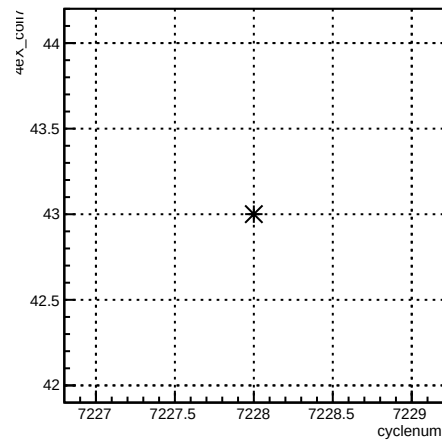
4eX_coil7:cyclenum {run == 6886}
