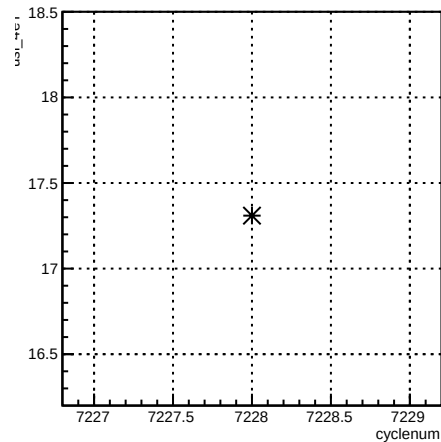
usl_4eY:cyclenum {run == 6886}
