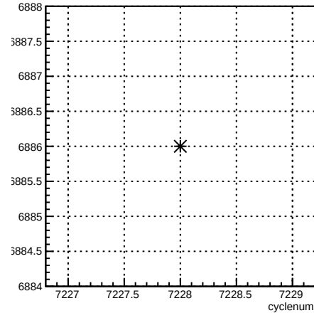
run:cyclenum {run == 6886}
