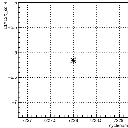
11X12X_coil4:cyclenum {run == 6886}
