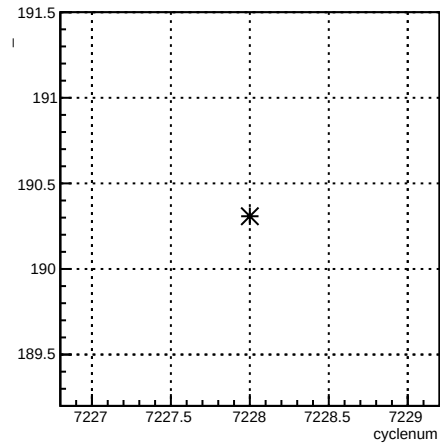
usr_4eX:cyclenum {run == 6886}
