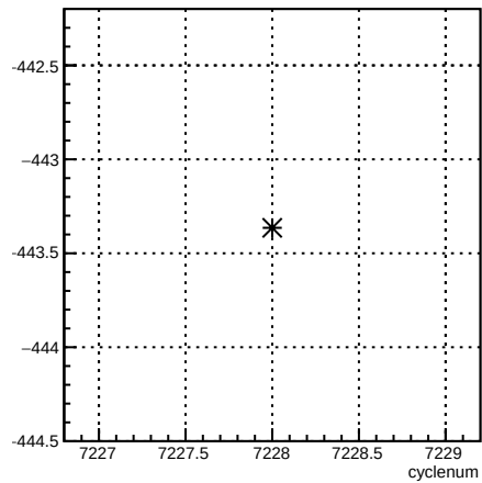
4eX_coil1:cyclenum {run == 6886}
