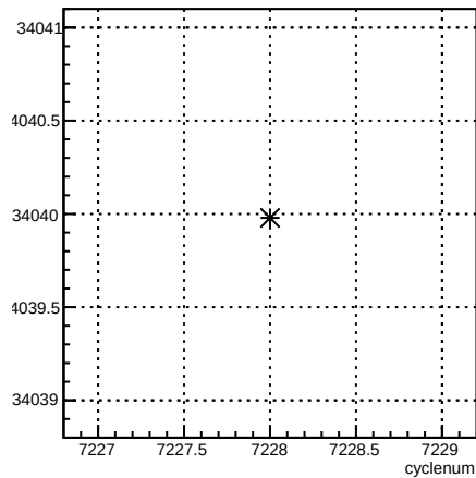
usl_coil6:cyclenum {run == 6886}
