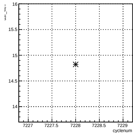
usr_4eY:cyclenum {run == 6886}
