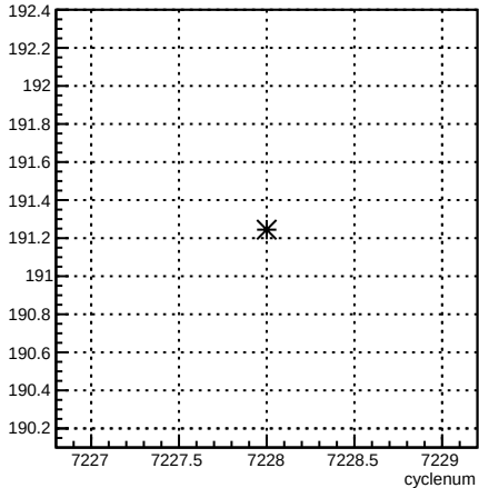
4eY_coil4:cyclenum {run == 6886}
