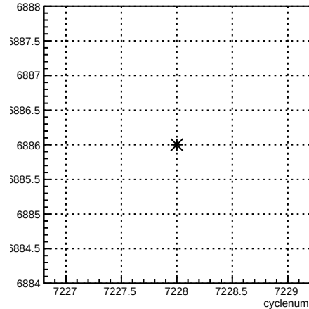
run:cyclenum {run == 6886}
