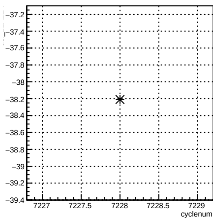
usl_11X12X:cyclenum {run == 6886}
