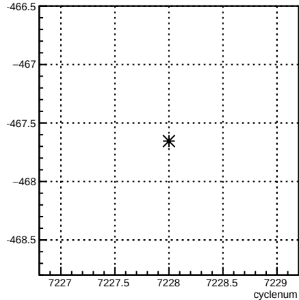
11X12X_coil7:cyclenum {run == 6886}
