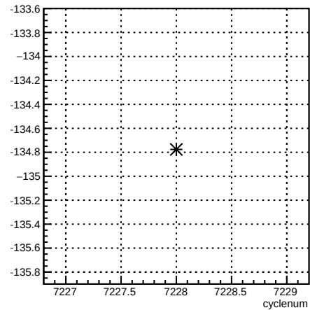
usr_4aX:cyclenum {run == 6886}
