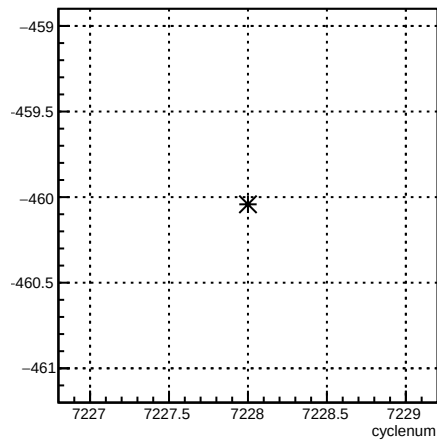
usr_coil6:cyclenum {run == 6886}
