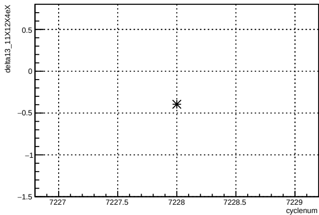
delta13_11X12X4eX:cyclenum {run == 6886}
