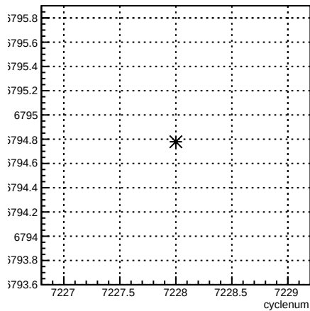
usl_coil7:cyclenum {run == 6886}
