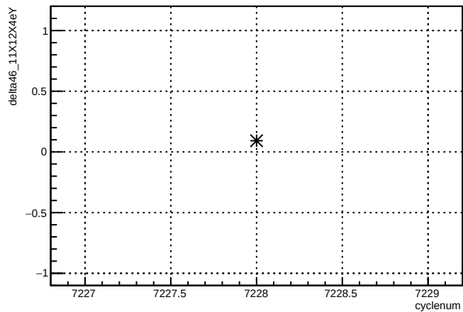
delta46_11X12X4eY:cyclenum {run == 6886}
