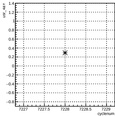
usr_4aY:cyclenum {run == 6886}
