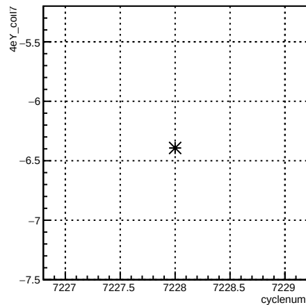
4eY_coil7:cyclenum {run == 6886}
