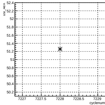
usl_4eX:cyclenum {run == 6886}
