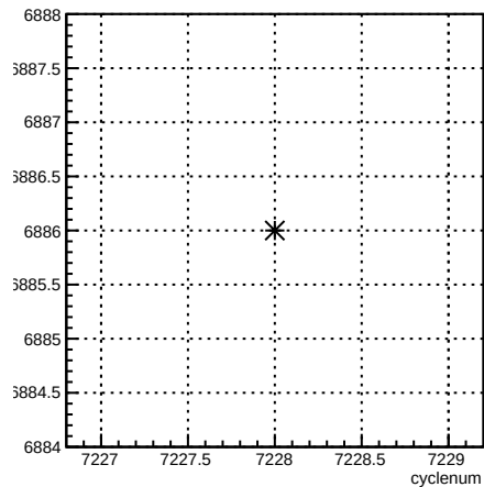
run:cyclenum {run == 6886}
