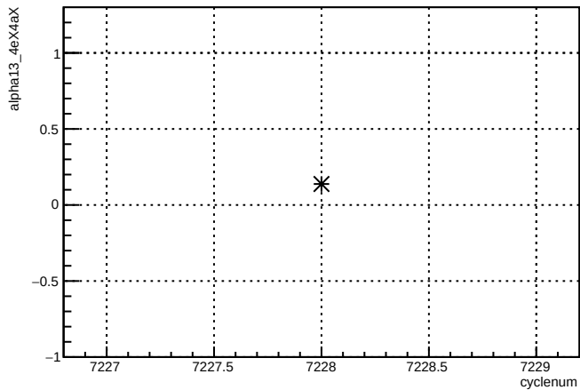
alpha13_4eX4aX:cyclenum {run == 6886}
