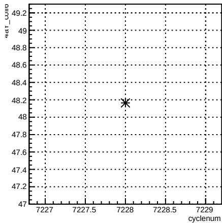
4eY_coil6:cyclenum {run == 6886}
