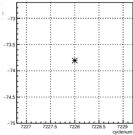
4eX_coil3:cyclenum {run == 6886}
