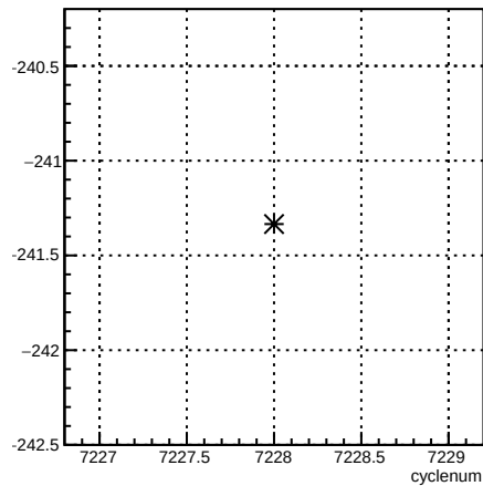
11X12X_coil1:cyclenum {run == 6886}
