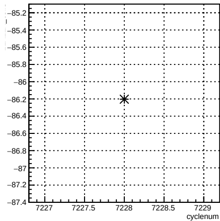
11X12X_coil3:cyclenum {run == 6886}
