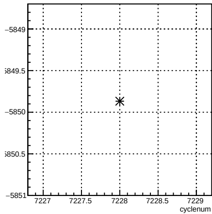
usr_coil7:cyclenum {run == 6886}
