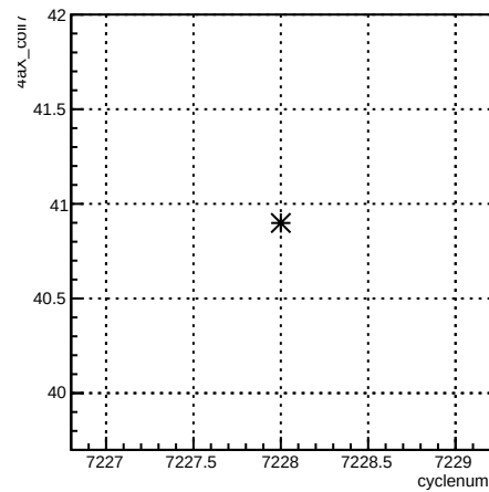
4aX_coil7:cyclenum {run == 6886}
