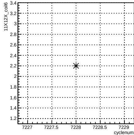
11X12X_coil6:cyclenum {run == 6886}
