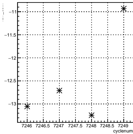
4eY_coil7:cyclenum {run == 6891}
