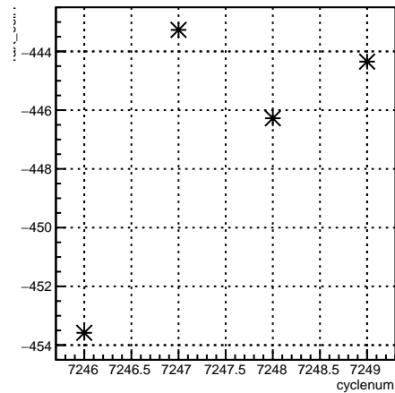
4aX_coil1:cyclenum {run == 6891}
