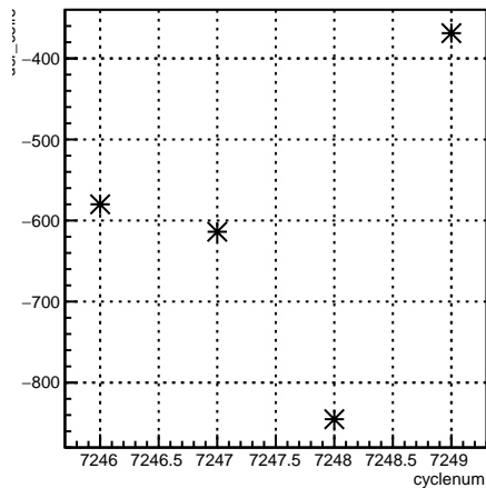
usr_coil6:cyclenum {run == 6891}
