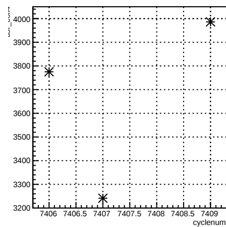
usr_coil4:cyclenum {run == 6943}
