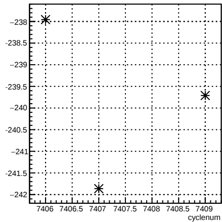
11X12X_coil1:cyclenum {run == 6943}
