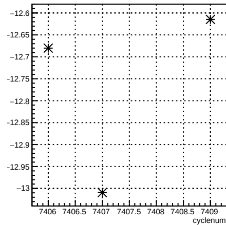
4eY_coil7:cyclenum {run == 6943}
