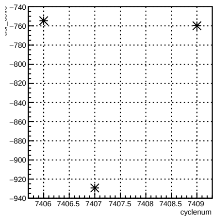
usr_coil6:cyclenum {run == 6943}
