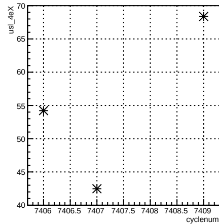
usl_4eX:cyclenum {run == 6943}
