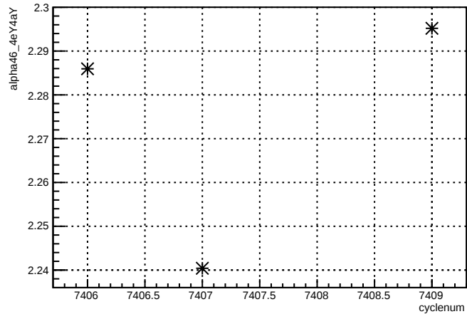
alpha46_4eY4aY:cyclenum {run == 6943}
