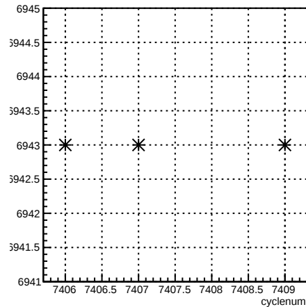
run:cyclenum {run == 6943}
