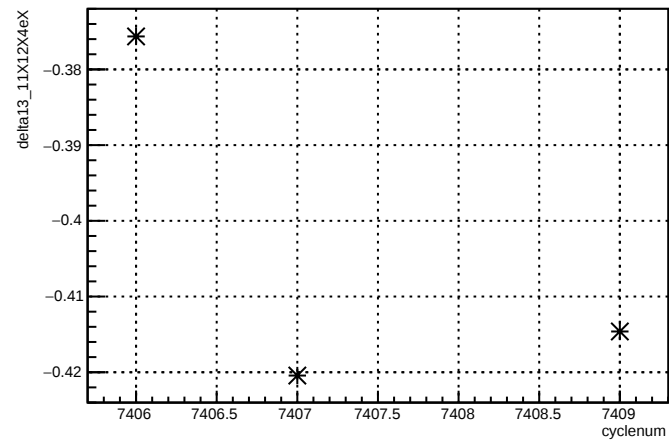
delta13_11X12X4eX:cyclenum {run == 6943}
