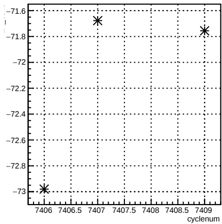
4eX_coil3:cyclenum {run == 6943}
