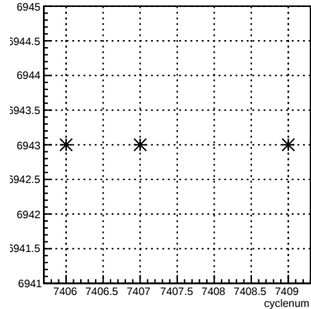
run:cyclenum {run == 6943}
