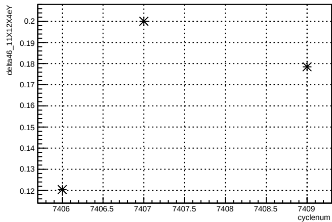
delta46_11X12X4eY:cyclenum {run == 6943}
