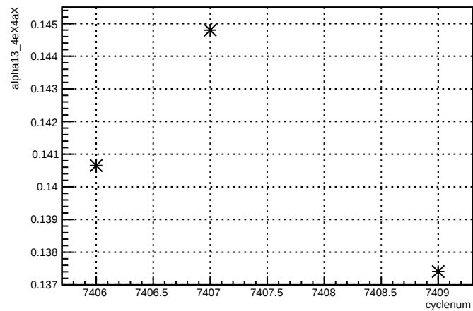
alpha13_4eX4aX:cyclenum {run == 6943}
