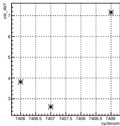
usr_4aY:cyclenum {run == 6943}
