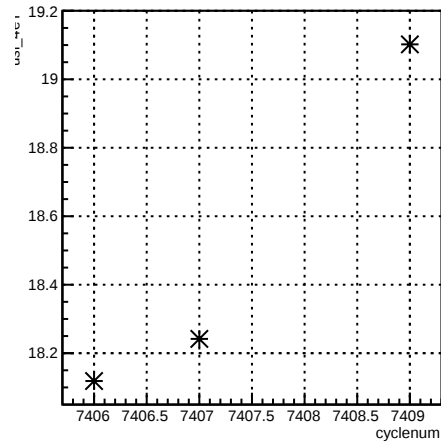
usl_4eY:cyclenum {run == 6943}
