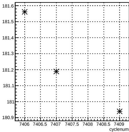
4eY_coil4:cyclenum {run == 6943}
