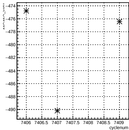
11X12X_coil7:cyclenum {run == 6943}
