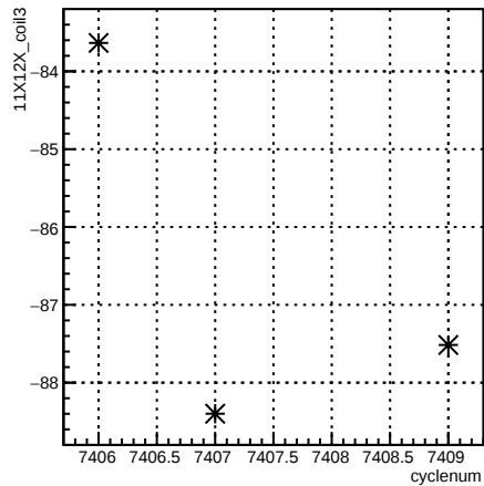
11X12X_coil3:cyclenum {run == 6943}
