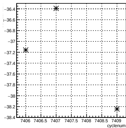
usr_11X12X:cyclenum {run == 6943}
