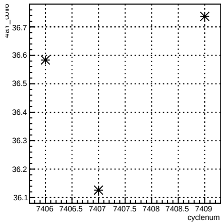
4eY_coil6:cyclenum {run == 6943}
