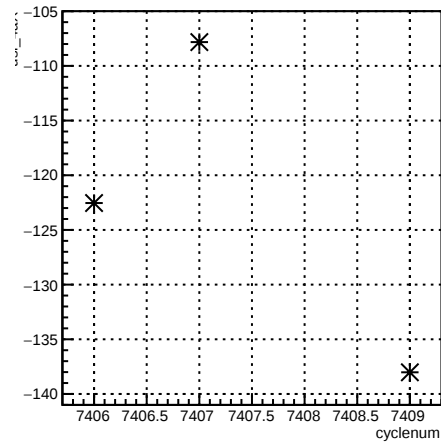
usl_4aX:cyclenum {run == 6943}
