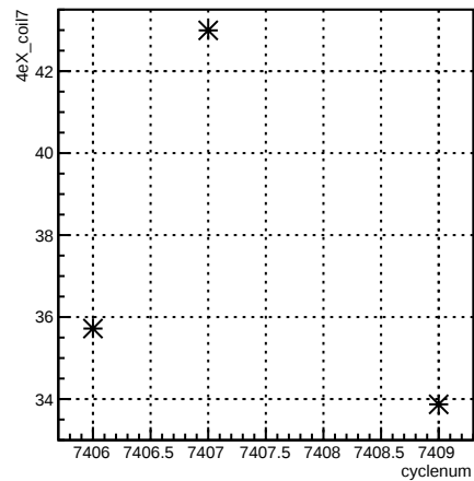
4eX_coil7:cyclenum {run == 6943}
