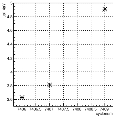
usl_4aY:cyclenum {run == 6943}
