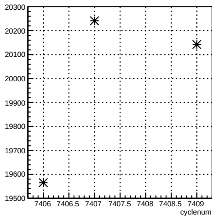
usr_coil7:cyclenum {run == 6943}
