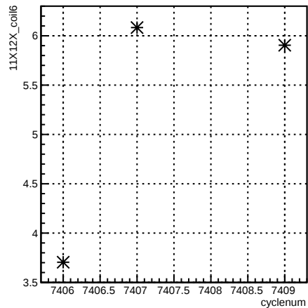
11X12X_coil6:cyclenum {run == 6943}
