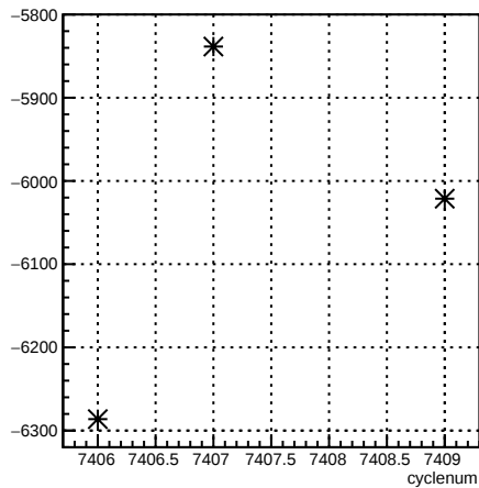
usr_coil3:cyclenum {run == 6943}
