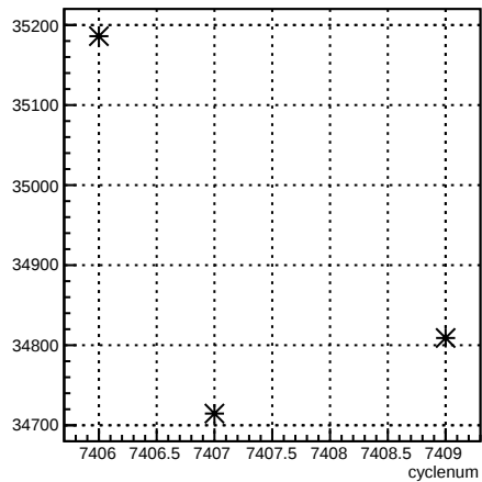
usl_coil6:cyclenum {run == 6943}
