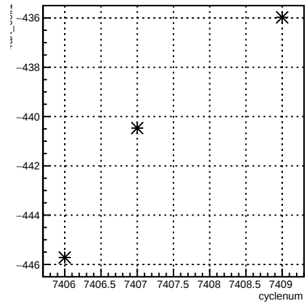
4eX_coil1:cyclenum {run == 6943}
