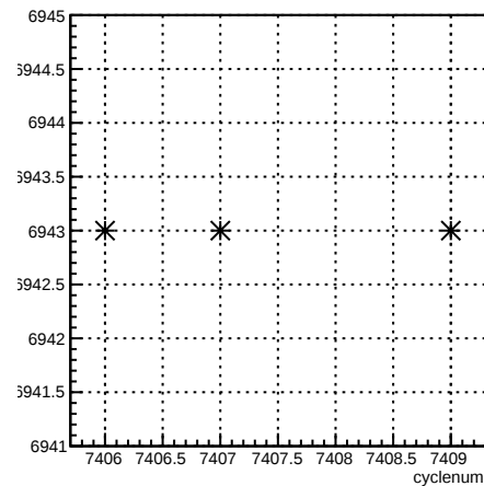
run:cyclenum {run == 6943}
