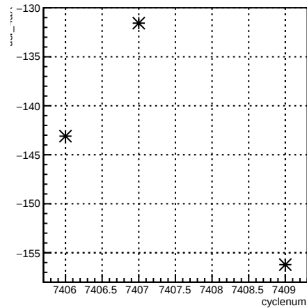
usr_4aX:cyclenum {run == 6943}
