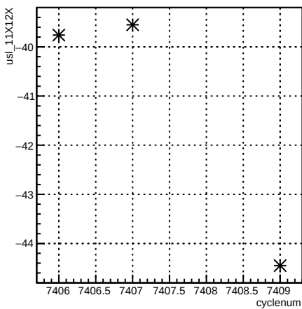
usl_11X12X:cyclenum {run == 6943}
