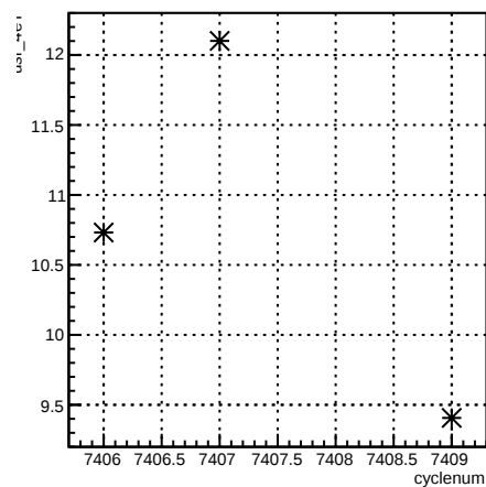
usr_4eY:cyclenum {run == 6943}
