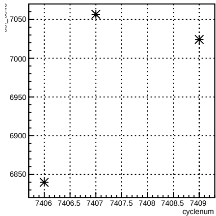
usl_coil7:cyclenum {run == 6943}
