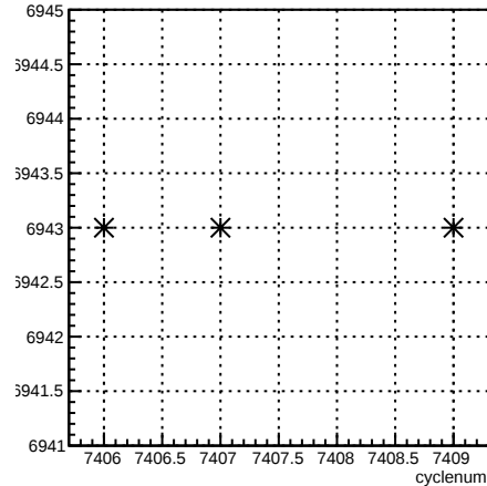
run:cyclenum {run == 6943}
