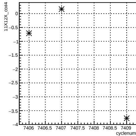
11X12X_coil4:cyclenum {run == 6943}
