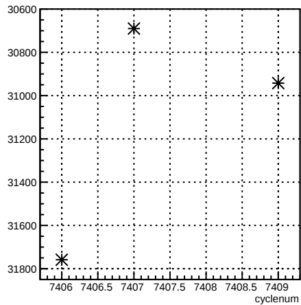
usr_coil1:cyclenum {run == 6943}
