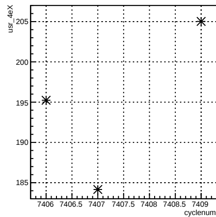
usr_4eX:cyclenum {run == 6943}
