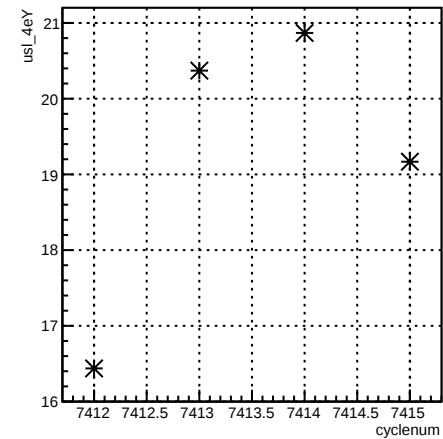
usl_4eY:cyclenum {run == 6944}
