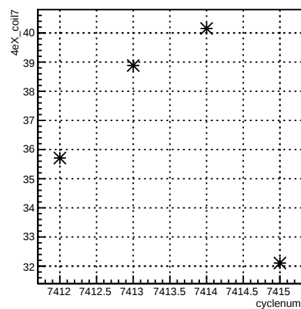
4eX_coil7:cyclenum {run == 6944}
