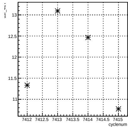
usr_4eY:cyclenum {run == 6944}
