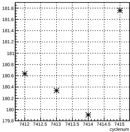
4eY_coil4:cyclenum {run == 6944}
