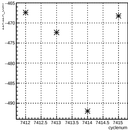
11X12X_coil7:cyclenum {run == 6944}
