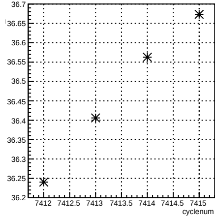
4eY_coil6:cyclenum {run == 6944}
