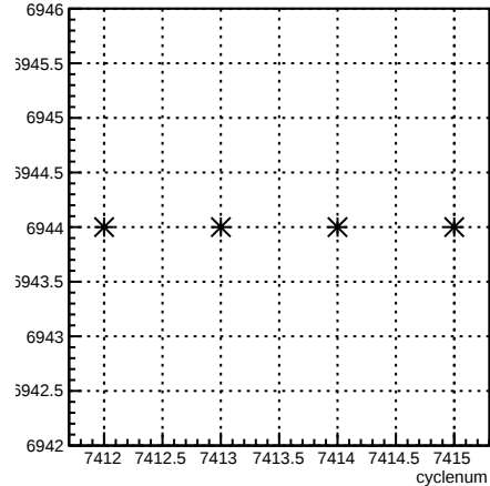
run:cyclenum {run == 6944}
