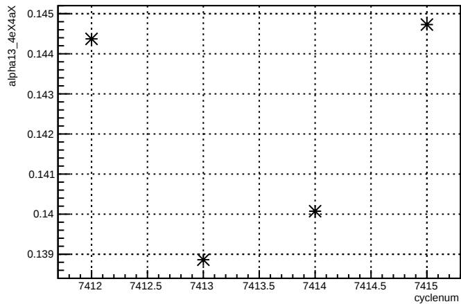
alpha13_4eX4aX:cyclenum {run == 6944}
