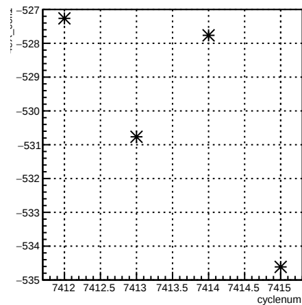
4eX_coil1:cyclenum {run == 6944}
