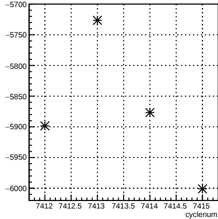
usr_coil7:cyclenum {run == 6944}
