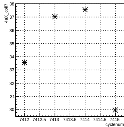
4aX_coil7:cyclenum {run == 6944}
