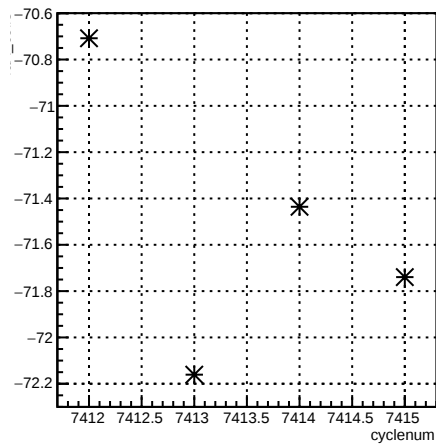
4aX_coil3:cyclenum {run == 6944}
