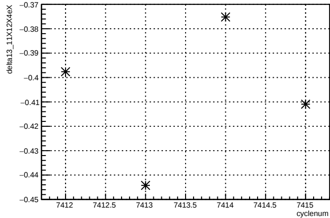
delta13_11X12X4eX:cyclenum {run == 6944}
