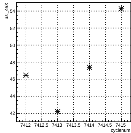
run:cyclenum {run == 6944}
