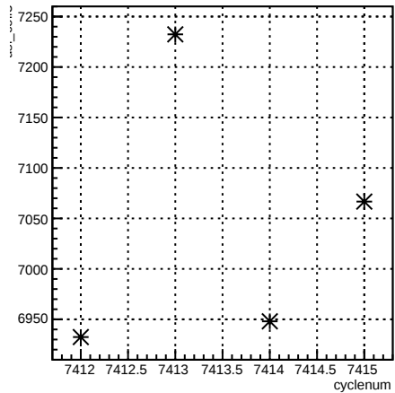
usl_coil7:cyclenum {run == 6944}
