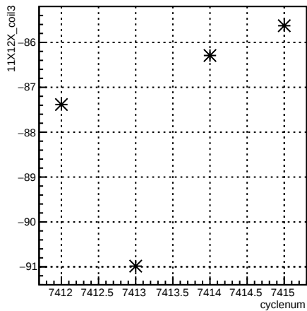
11X12X_coil3:cyclenum {run == 6944}
