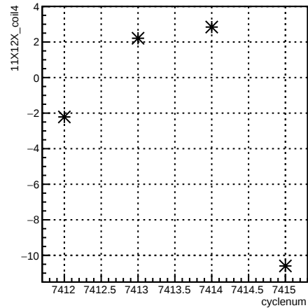
11X12X_coil4:cyclenum {run == 6944}
