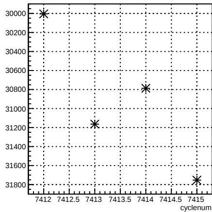
usr_coil6:cyclenum {run == 6944}
