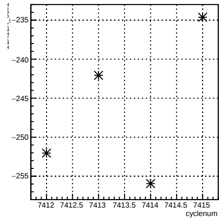
11X12X_coil1:cyclenum {run == 6944}
