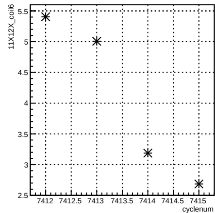
11X12X_coil6:cyclenum {run == 6944}
