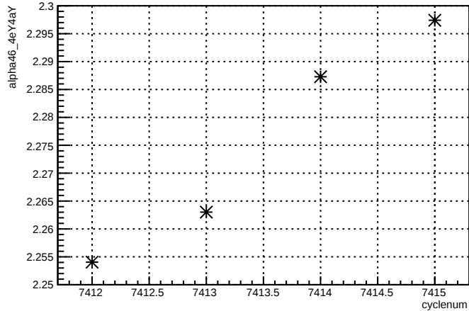
alpha46_4eY4aY:cyclenum {run == 6944}
