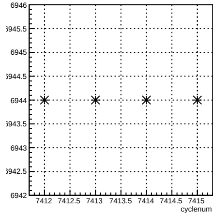
run:cyclenum {run == 6944}
