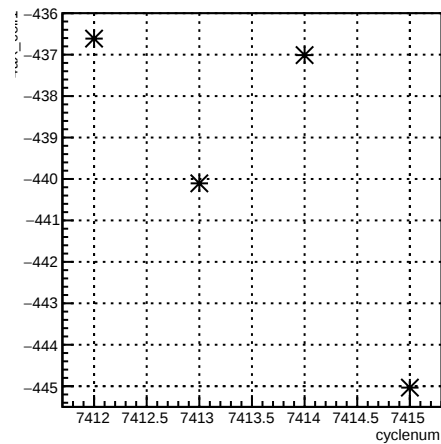
4aX_coil1:cyclenum {run == 6944}
