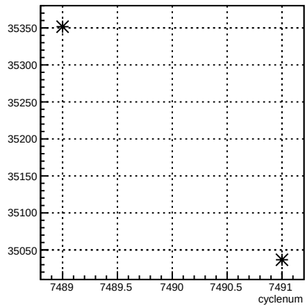
usl_coil6:cyclenum {run == 6960}
