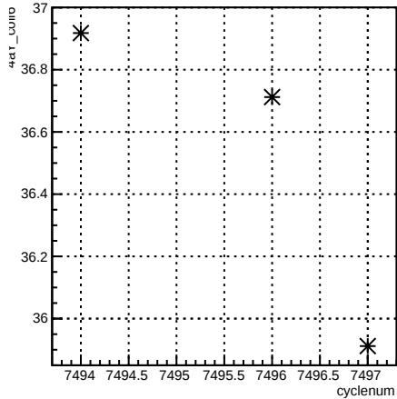
4eY_coil6:cyclenum {run == 6961}
