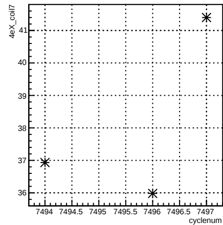
4eX_coil7:cyclenum {run == 6961}
