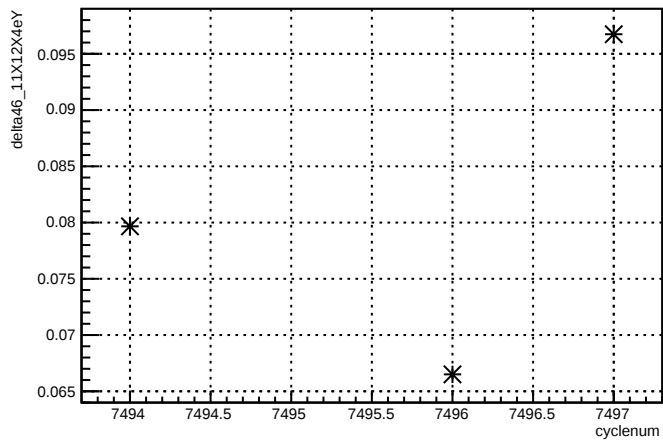
delta46_11X12X4eY:cyclenum {run == 6961}
