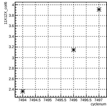
11X12X_coil6:cyclenum {run == 6961}
