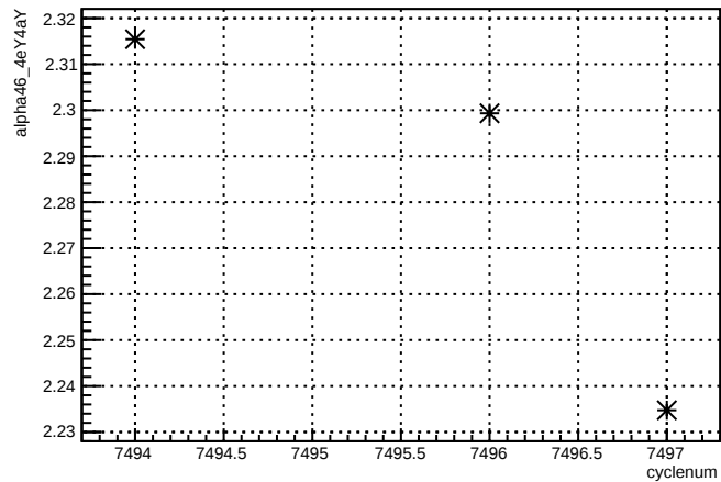
alpha46_4eY4aY:cyclenum {run == 6961}
