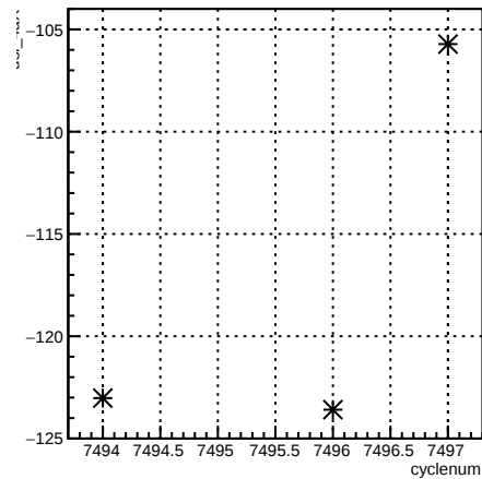
usl_4eY:cyclenum {run == 6961}
