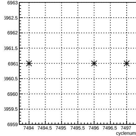
run:cyclenum {run == 6961}
