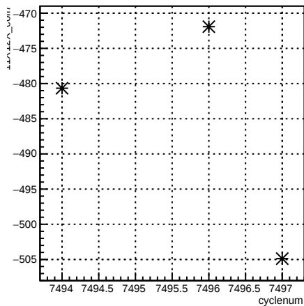
11X12X_coil7:cyclenum {run == 6961}
