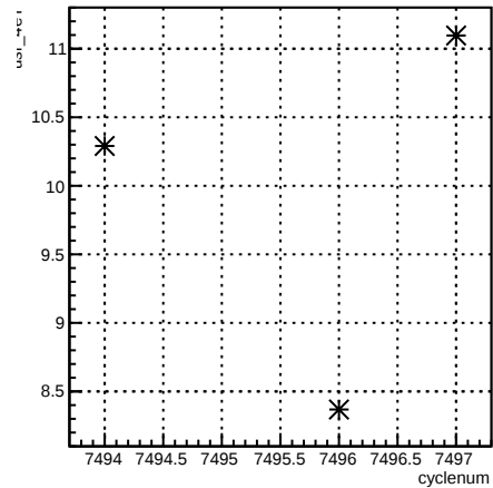
usr_4eY:cyclenum {run == 6961}
