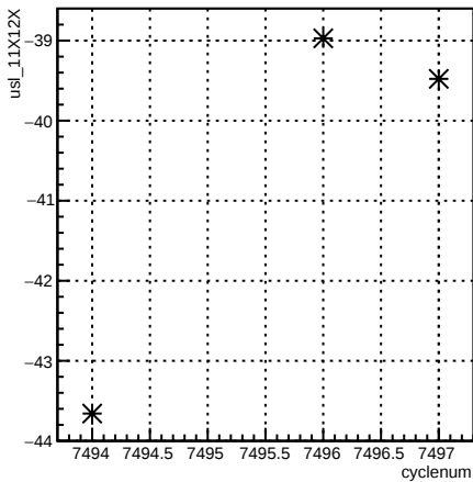
usl_11X12X:cyclenum {run == 6961}
