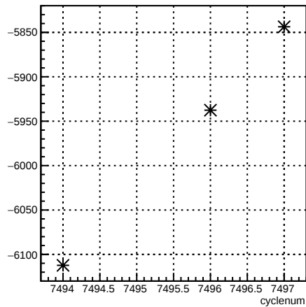
usr_coil3:cyclenum {run == 6961}
