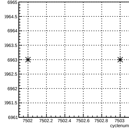
run:cyclenum {run == 6963}
