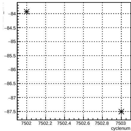
11X12X_coil3:cyclenum {run == 6963}
