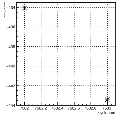
4eX_coil1:cyclenum {run == 6963}
