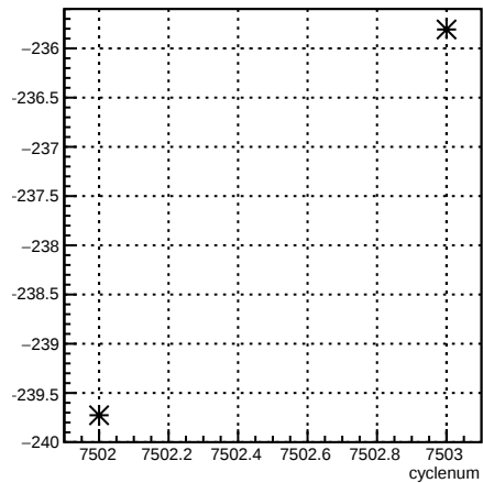
11X12X_coil1:cyclenum {run == 6963}
