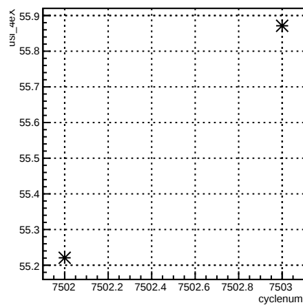
usl_4eX:cyclenum {run == 6963}
