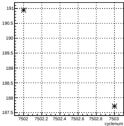
4eY_coil4:cyclenum {run == 6963}
