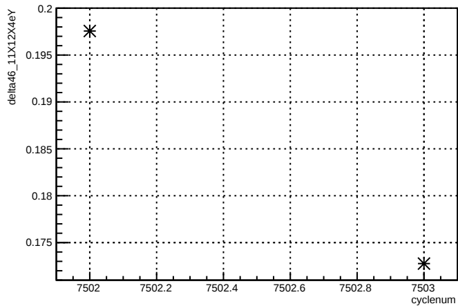
delta46_11X12X4eY:cyclenum {run == 6963}
