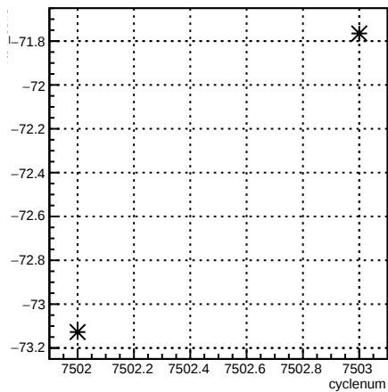
4eX_coil3:cyclenum {run == 6963}
