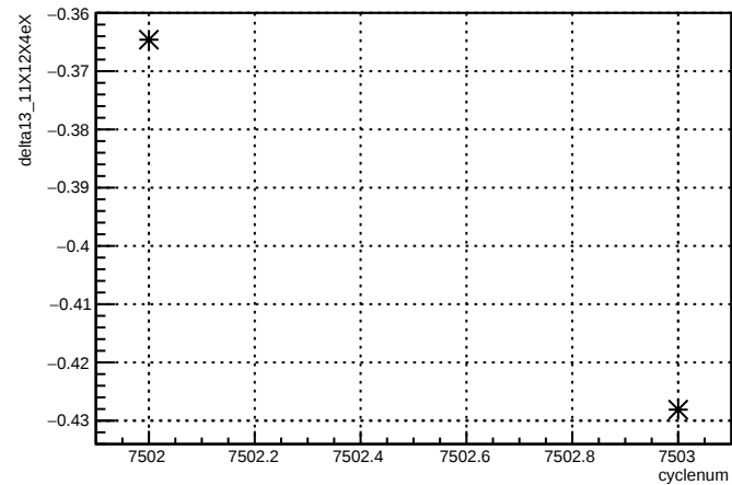
delta13_11X12X4eX:cyclenum {run == 6963}
