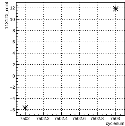
11X12X_coil4:cyclenum {run == 6963}
