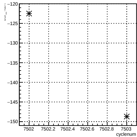
usr_4aX:cyclenum {run == 6963}
