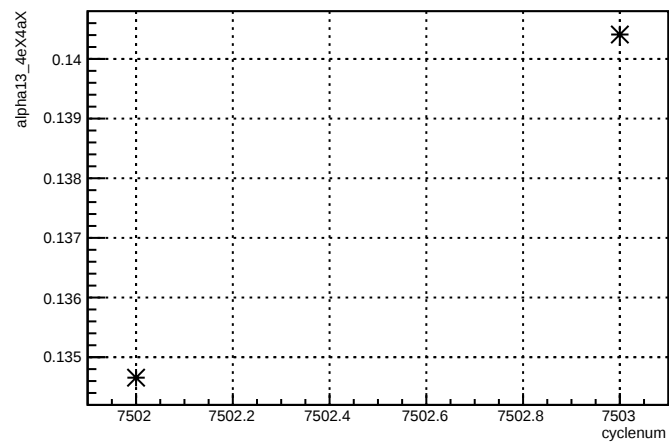
alpha13_4eX4aX:cyclenum {run == 6963}
