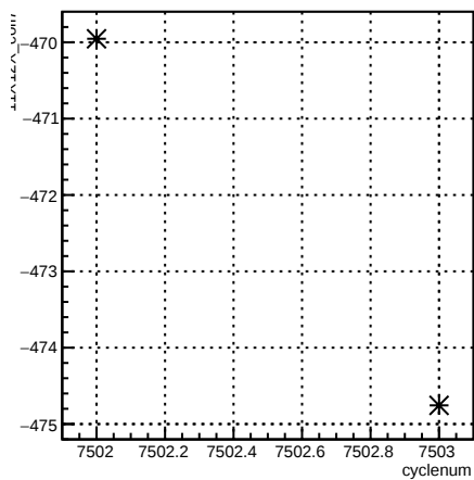
11X12X_coil7:cyclenum {run == 6963}
