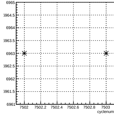
run:cyclenum {run == 6963}
