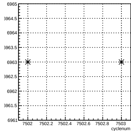
run:cyclenum {run == 6963}
