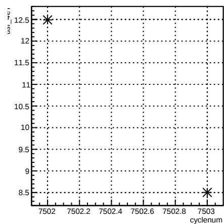
usr_4eY:cyclenum {run == 6963}
