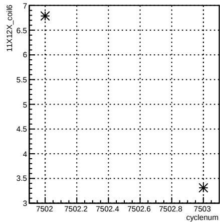
11X12X_coil6:cyclenum {run == 6963}
