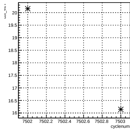
usl_4eY:cyclenum {run == 6963}
