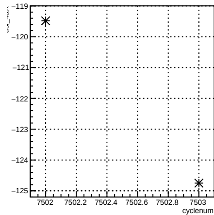
usl_4aX:cyclenum {run == 6963}
