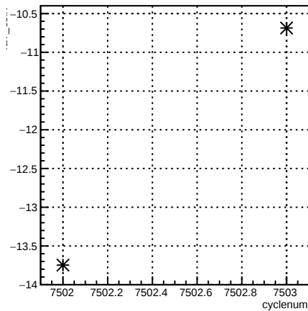
4eY_coil7:cyclenum {run == 6963}
