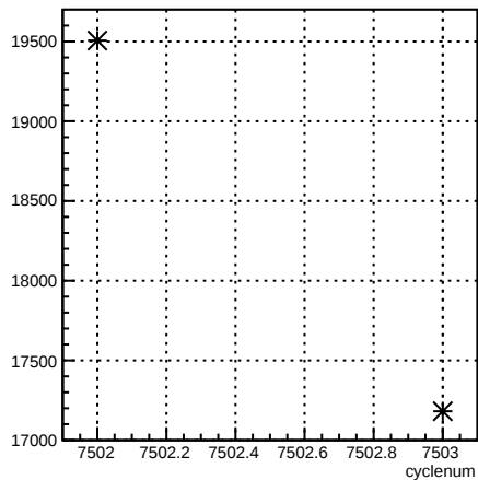
usl_coil7:cyclenum {run == 6963}
