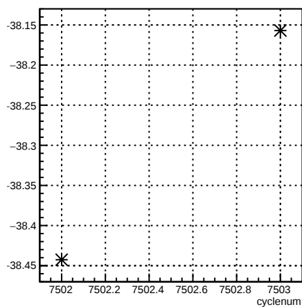
usr_11X12X:cyclenum {run == 6963}
