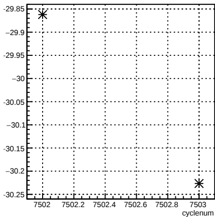
4eY_coil6:cyclenum {run == 6963}
