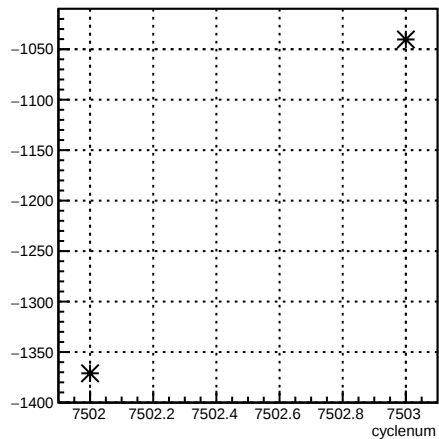
usl_coil6:cyclenum {run == 6963}
