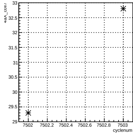
4eX_coil7:cyclenum {run == 6963}
