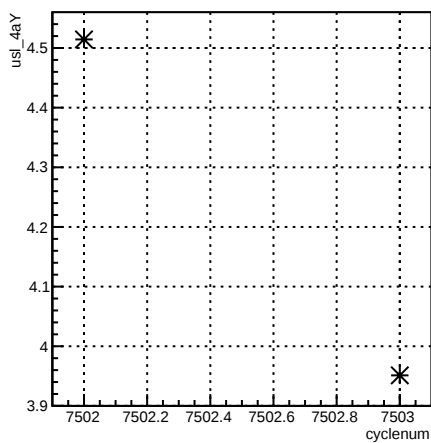
usl_4aY:cyclenum {run == 6963}
