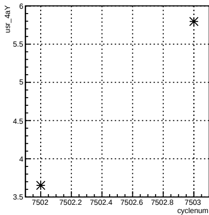
usr_4aY:cyclenum {run == 6963}
