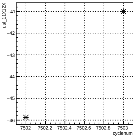
usl_11X12X:cyclenum {run == 6963}
