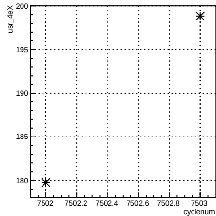
usr_4eX:cyclenum {run == 6963}
