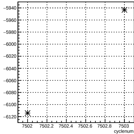
usr_coil7:cyclenum {run == 6963}
