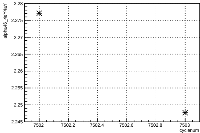
alpha46_4eY4aY:cyclenum {run == 6963}
