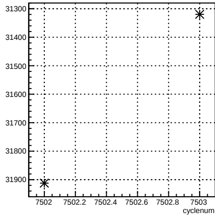
usr_coil6:cyclenum {run == 6963}
