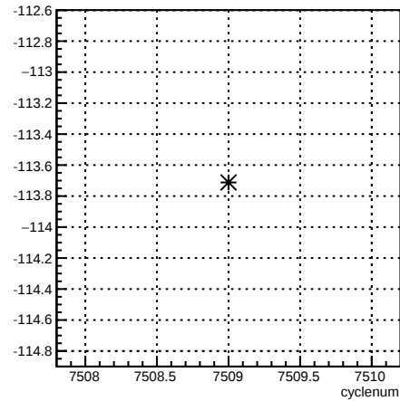
usl_4aX:cyclenum {run == 6964}
