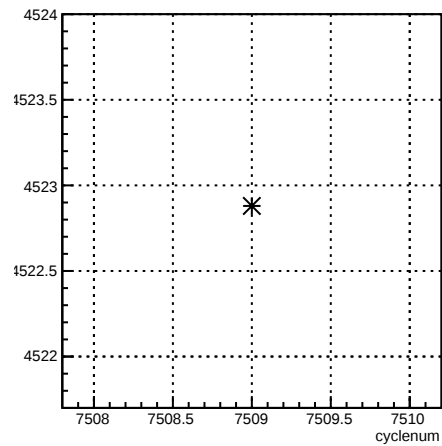
usl_coil4:cyclenum {run == 6964}
