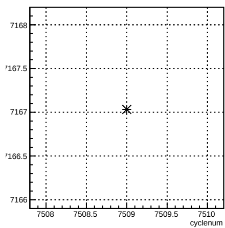
usl_coil3:cyclenum {run == 6964}
