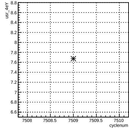
usr_4eY:cyclenum {run == 6964}
