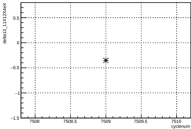
delta13_11X12X4eX:cyclenum {run == 6964}
