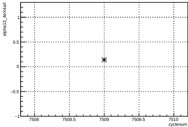
alpha13_4eX4aX:cyclenum {run == 6964}
