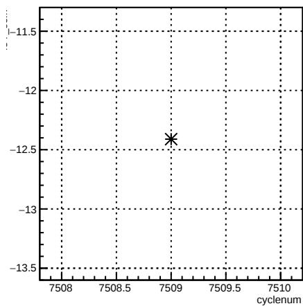
4eY_coil7:cyclenum {run == 6964}
