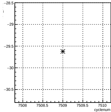
4eY_coil6:cyclenum {run == 6964}
