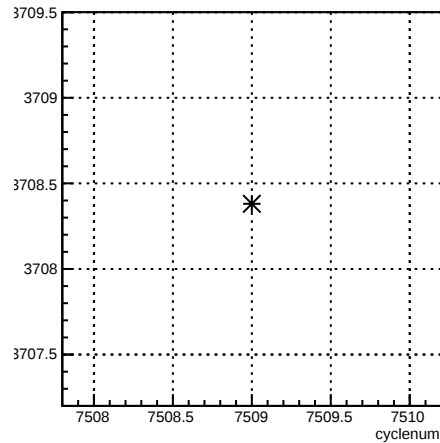
usr_coil4:cyclenum {run == 6964}
