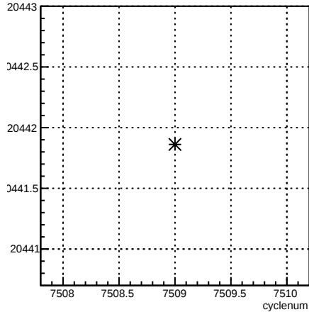
usr_coil7:cyclenum {run == 6964}
