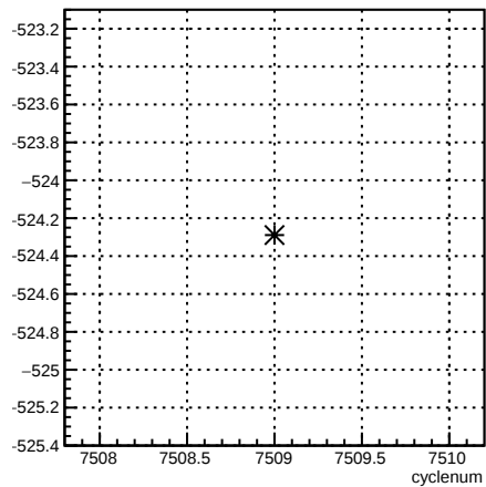
4eX_coil1:cyclenum {run == 6964}
