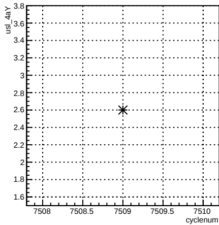
usl_4aY:cyclenum {run == 6964}
