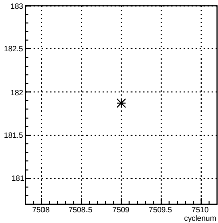
4aY_coil4:cyclenum {run == 6964}
