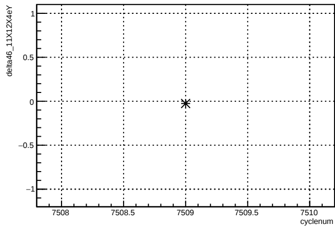
delta46_11X12X4eY:cyclenum {run == 6964}
