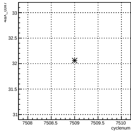
4eX_coil7:cyclenum {run == 6964}
