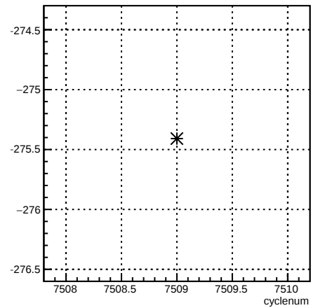
11X12X_coil6:cyclenum {run == 6964}
