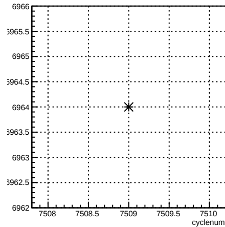
run:cyclenum {run == 6964}
