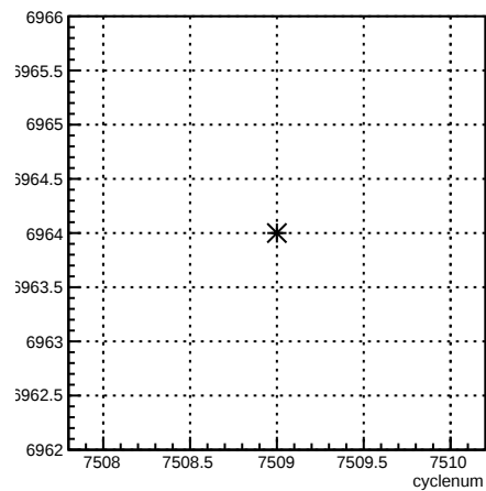
run:cyclenum {run == 6964}
