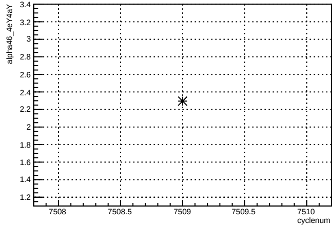
alpha46_4eY4aY:cyclenum {run == 6964}
