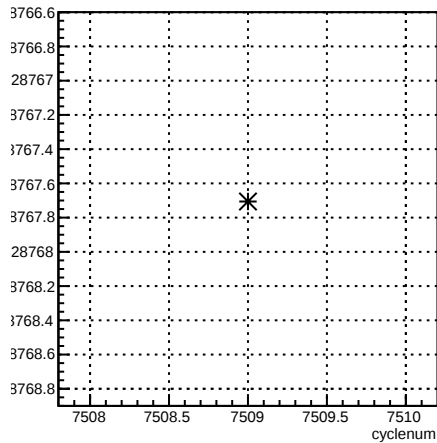
usr_coil1:cyclenum {run == 6964}
