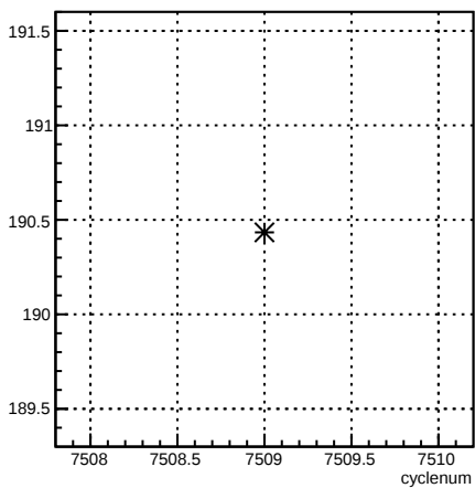
4eY_coil4:cyclenum {run == 6964}
