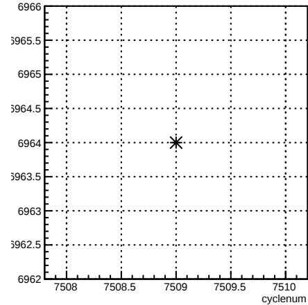
run:cyclenum {run == 6964}
