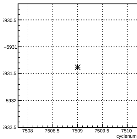
usr_coil3:cyclenum {run == 6964}
