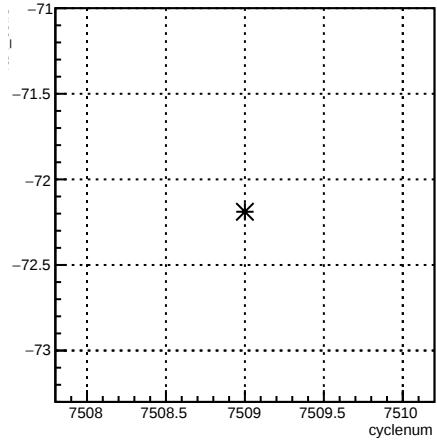
4eX_coil3:cyclenum {run == 6964}
