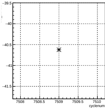
usl_11X12X:cyclenum {run == 6964}
