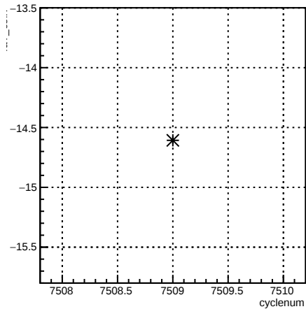
4aY_coil7:cyclenum {run == 6964}
