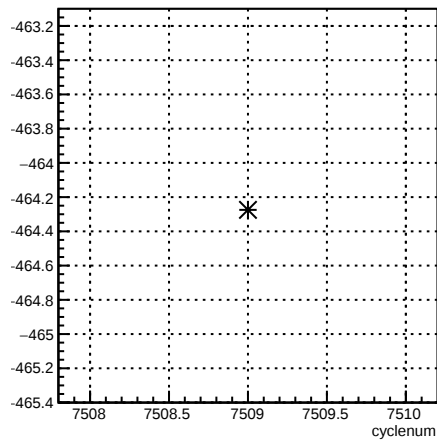
usr_coil6:cyclenum {run == 6964}
