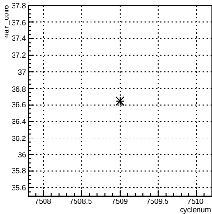
4aY_coil6:cyclenum {run == 6964}
