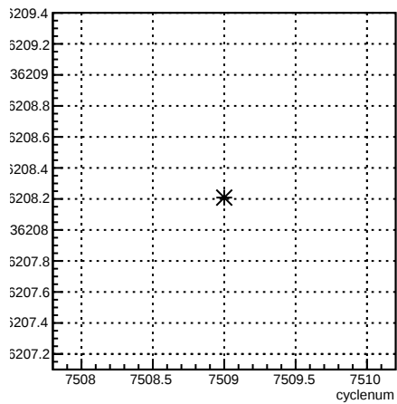
usl_coil1:cyclenum {run == 6964}
