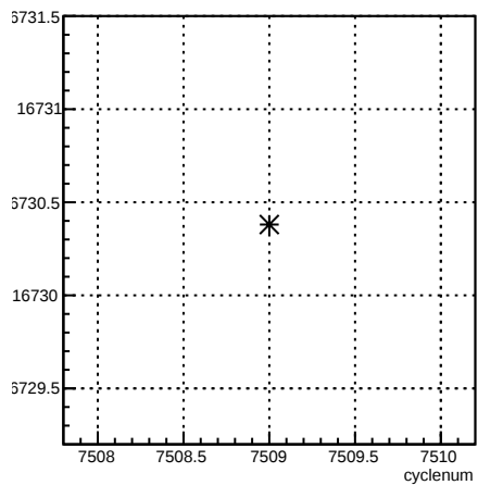
usl_coil7:cyclenum {run == 6964}
