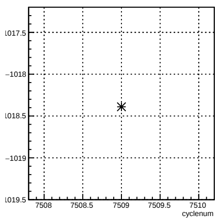
usl_coil6:cyclenum {run == 6964}
