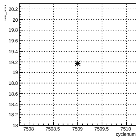
usl_4eY:cyclenum {run == 6964}
