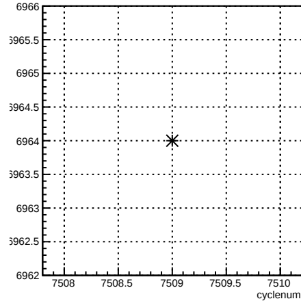
run:cyclenum {run == 6964}
