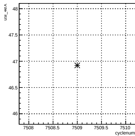
usl_4eX:cyclenum {run == 6964}
