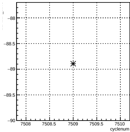
11X12X_coil7:cyclenum {run == 6964}
