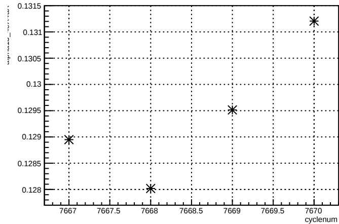
alpha13_4eX4aX:cyclenum {run == 7006}
