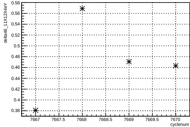
delta46_11X12X4eY:cyclenum {run == 7006}
