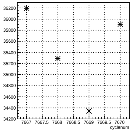
usl_coil6:cyclenum {run == 7006}
