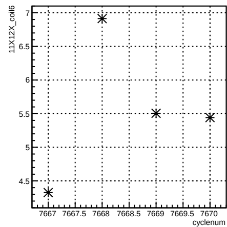
11X12X_coil6:cyclenum {run == 7006}
