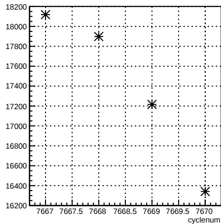
usr_coil7:cyclenum {run == 7006}
