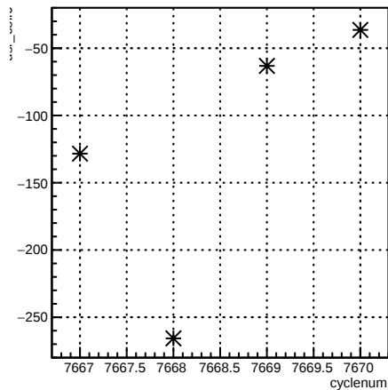
usr_coil6:cyclenum {run == 7006}
