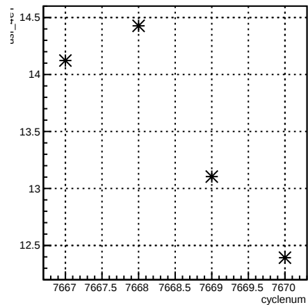
usr_4eY:cyclenum {run == 7006}
