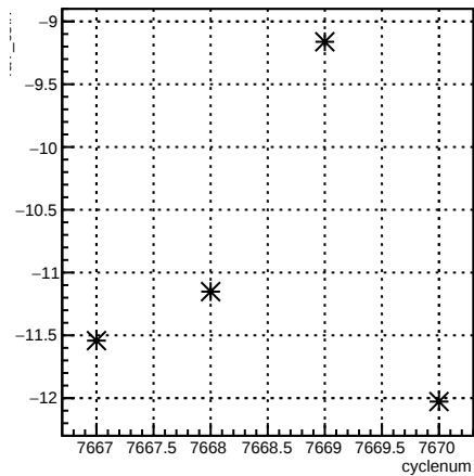
4eY_coil7:cyclenum {run == 7006}
