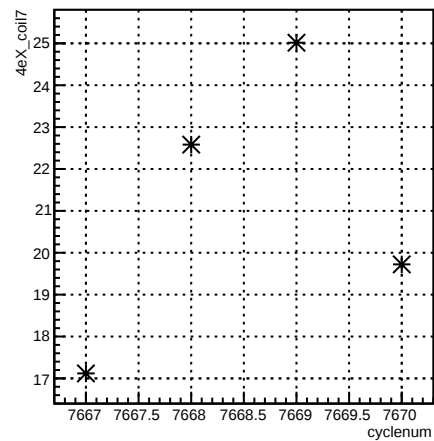
4eX_coil7:cyclenum {run == 7006}
