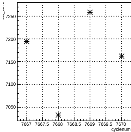
usl_coil7:cyclenum {run == 7006}
