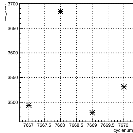
usr_coil4:cyclenum {run == 7006}
