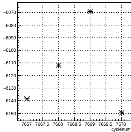
usr_coil7:cyclenum {run == 7006}
