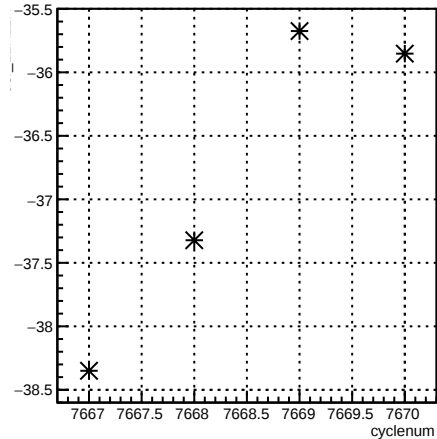
usr_11X12X:cyclenum {run == 7006}
