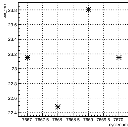
usl_4eY:cyclenum {run == 7006}
