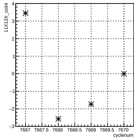
11X12X_coil4:cyclenum {run == 7006}
