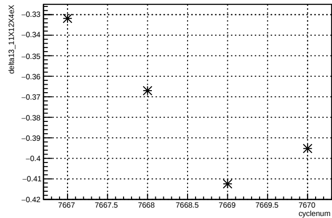
delta13_11X12X4eX:cyclenum {run == 7006}
