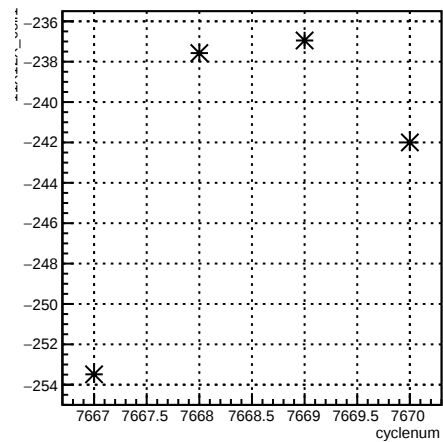
11X12X_coil1:cyclenum {run == 7006}
