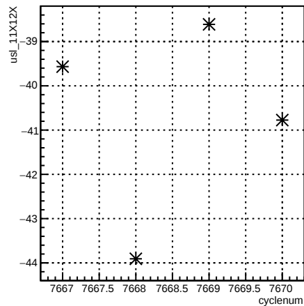
usl_11X12X:cyclenum {run == 7006}
