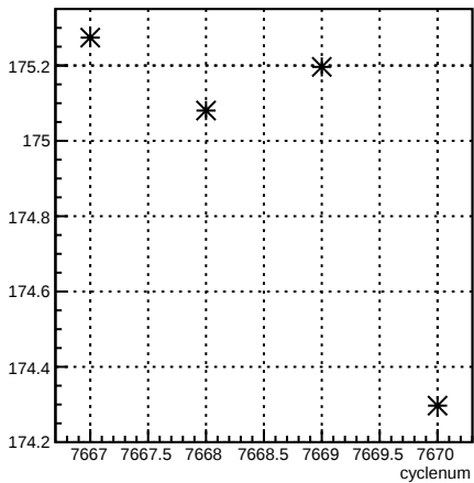
4eY_coil4:cyclenum {run == 7006}
