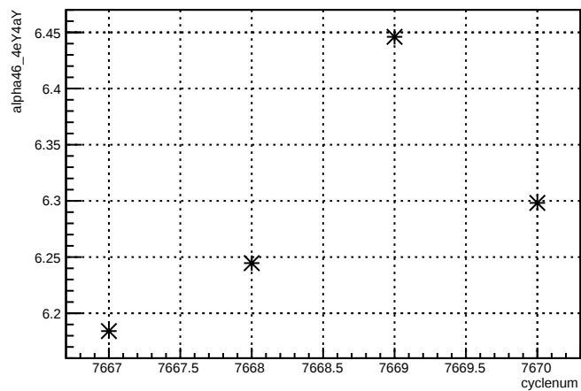
alpha46_4eY4aY:cyclenum {run == 7006}
