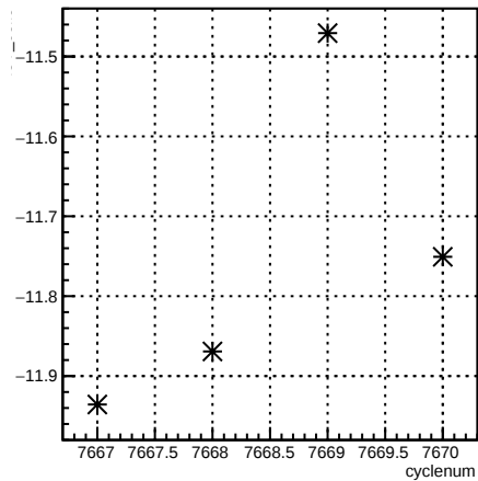
4eY_coil6:cyclenum {run == 7006}
