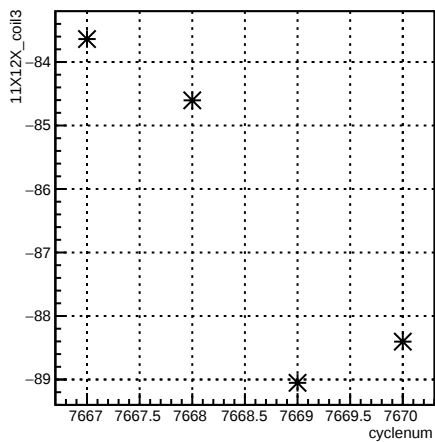
11X12X_coil3:cyclenum {run == 7006}
