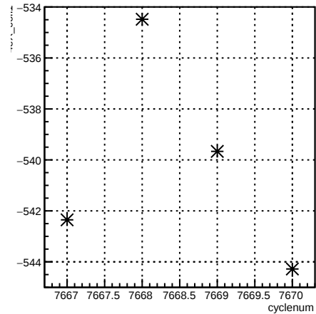
4eX_coil1:cyclenum {run == 7006}
