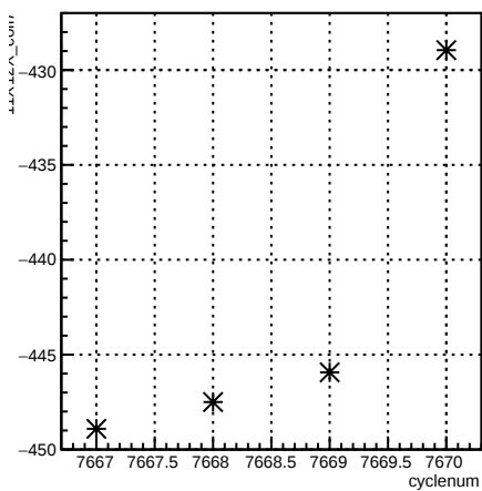
11X12X_coil7:cyclenum {run == 7006}
