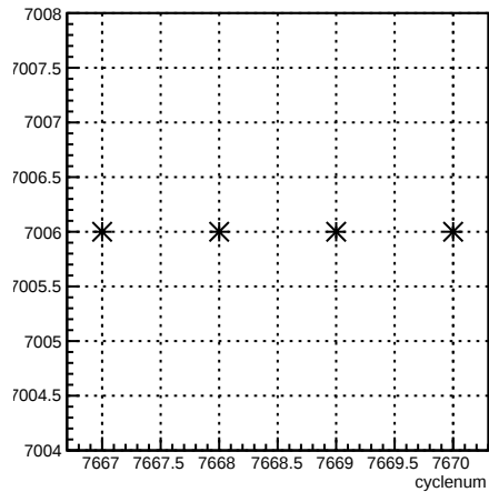
run:cyclenum {run == 7006}
