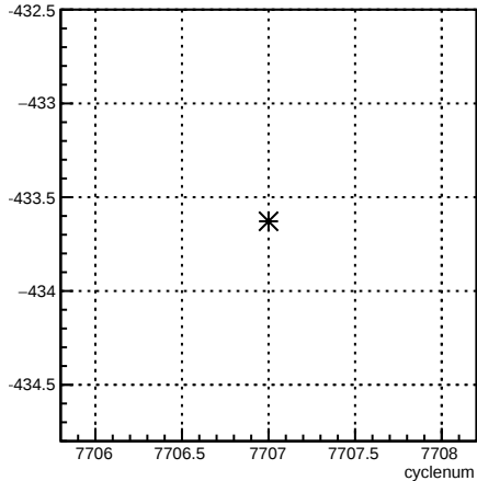
11X12X_coil7:cyclenum {run == 7015}
