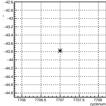
usl_11X12X:cyclenum {run == 7015}
