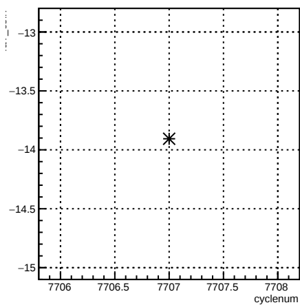
4aY_coil7:cyclenum {run == 7015}
