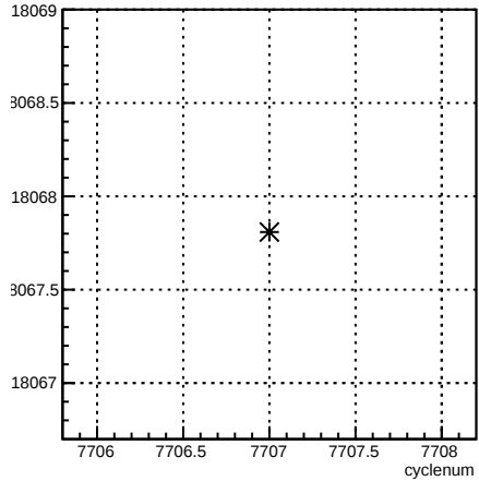
usl_coil7:cyclenum {run == 7015}
