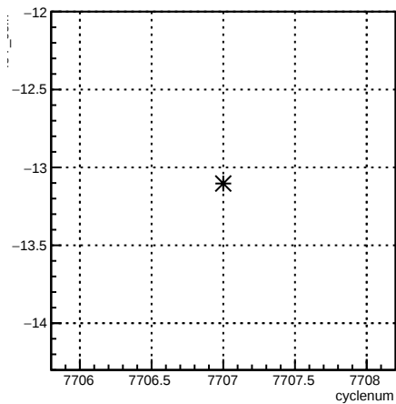
4eY_coil7:cyclenum {run == 7015}
