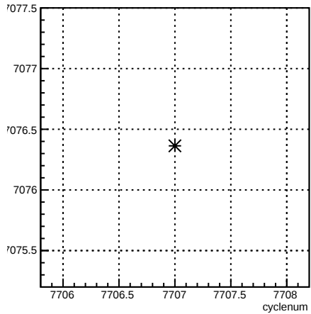
usl_coil3:cyclenum {run == 7015}
