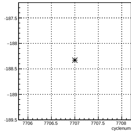
usr_coil6:cyclenum {run == 7015}
