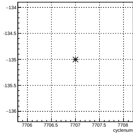
usl_4eY:cyclenum {run == 7015}
