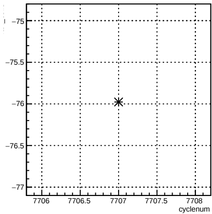
4eX_coil3:cyclenum {run == 7015}
