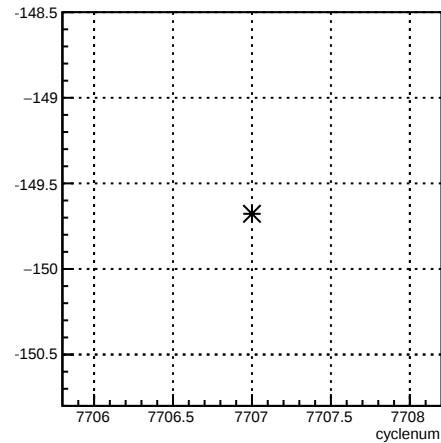
usr_4aX:cyclenum {run == 7015}
