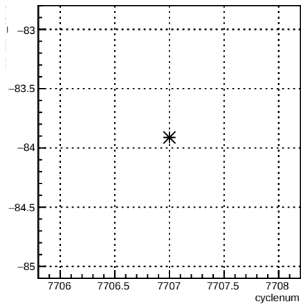
11X12X_coil3:cyclenum {run == 7015}
