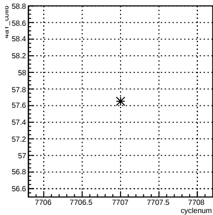
4aY_coil6:cyclenum {run == 7015}
