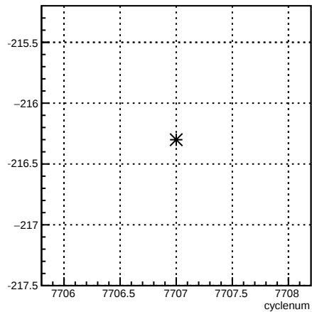
11X12X_coil1:cyclenum {run == 7015}
