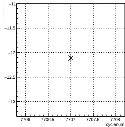
4eY_coil6:cyclenum {run == 7015}
