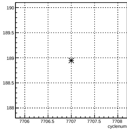
4eY_coil4:cyclenum {run == 7015}
