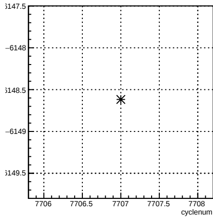
usr_coil3:cyclenum {run == 7015}
