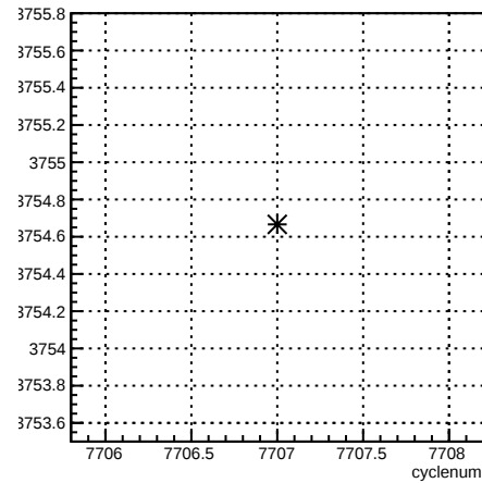
usr_coil4:cyclenum {run == 7015}
