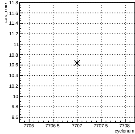
4eX_coil7:cyclenum {run == 7015}
