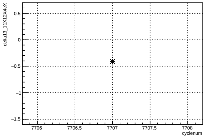
delta13_11X12X4eX:cyclenum {run == 7015}
