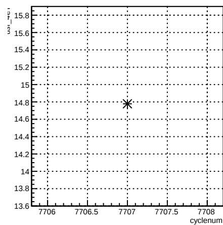
usr_4eY:cyclenum {run == 7015}
