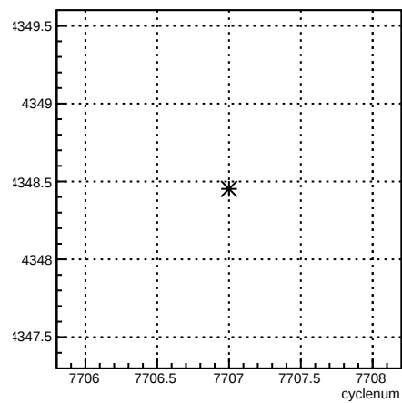
usl_coil4:cyclenum {run == 7015}
