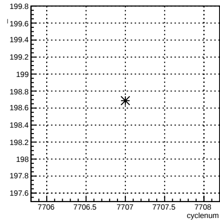
usr_4eX:cyclenum {run == 7015}
