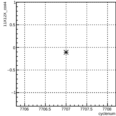
11X12X_coil4:cyclenum {run == 7015}
