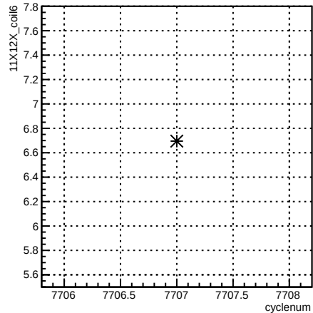
11X12X_coil6:cyclenum {run == 7015}
