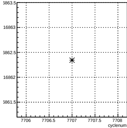
usr_coil7:cyclenum {run == 7015}
