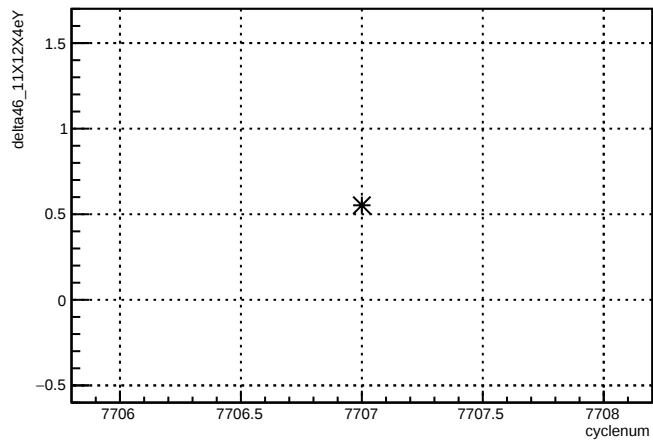
delta46_11X12X4eY:cyclenum {run == 7015}
