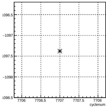
usl_coil6:cyclenum {run == 7015}
