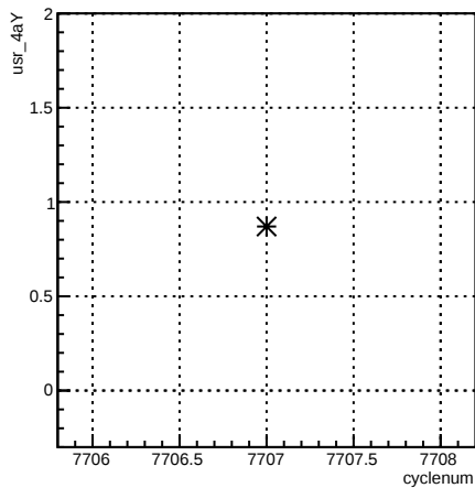
usr_4aY:cyclenum {run == 7015}
