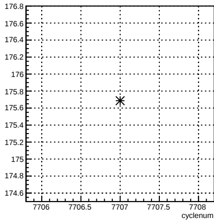
4aY_coil4:cyclenum {run == 7015}
