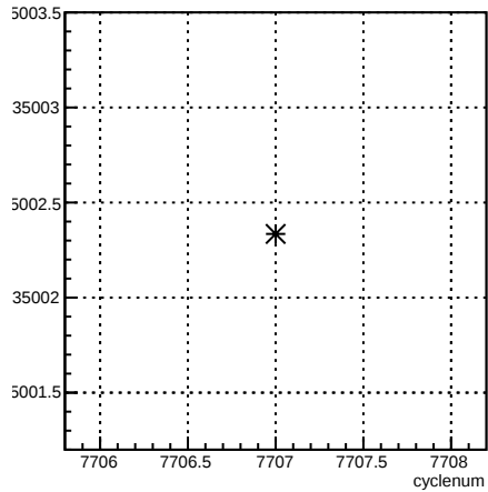
usl_coil1:cyclenum {run == 7015}
