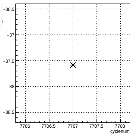
usr_11X12X:cyclenum {run == 7015}
