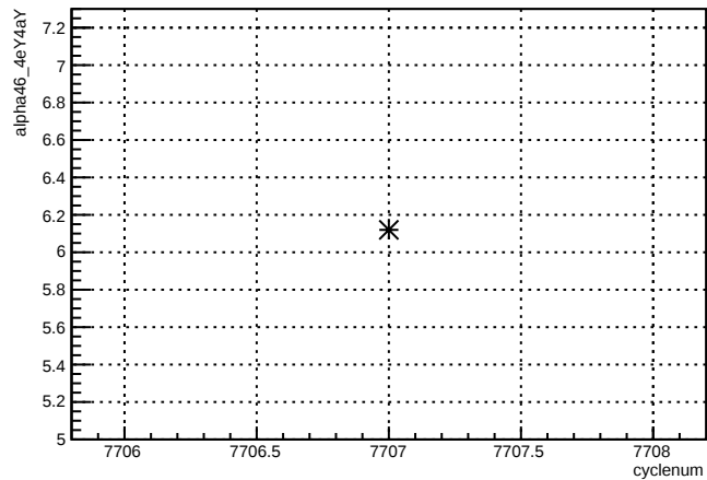
alpha46_4eY4aY:cyclenum {run == 7015}
