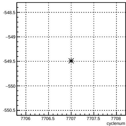
4eX_coil1:cyclenum {run == 7015}
