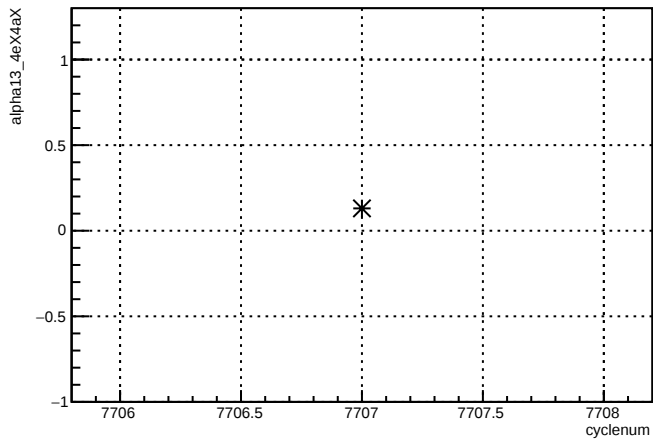
alpha13_4eX4aX:cyclenum {run == 7015}
