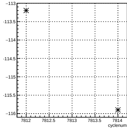
usl_4aX:cyclenum {run == 7044}
