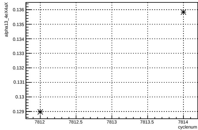
alpha13_4eX4aX:cyclenum {run == 7044}
