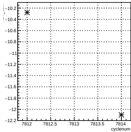
4eY_coil7:cyclenum {run == 7044}
