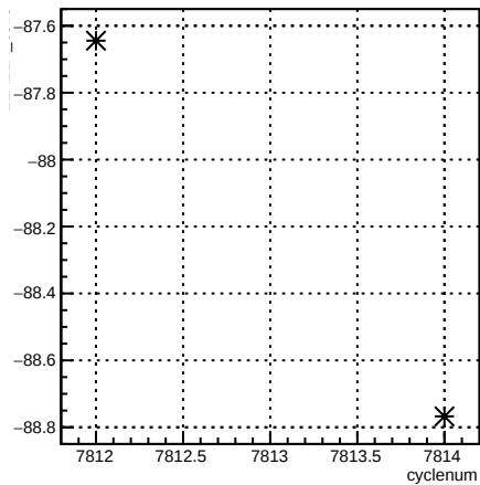
11X12X_coil3:cyclenum {run == 7044}
