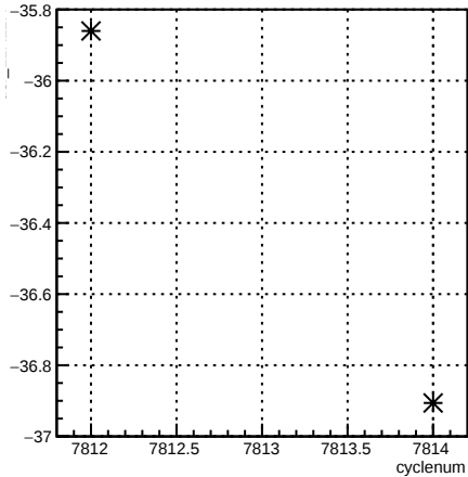
usr_11X12X:cyclenum {run == 7044}
