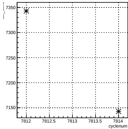
usl_coil7:cyclenum {run == 7044}
