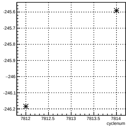
11X12X_coil1:cyclenum {run == 7044}
