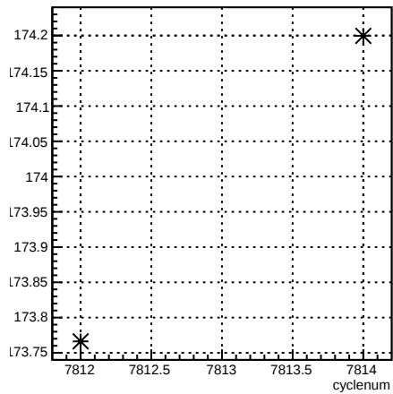
4eY_coil4:cyclenum {run == 7044}
