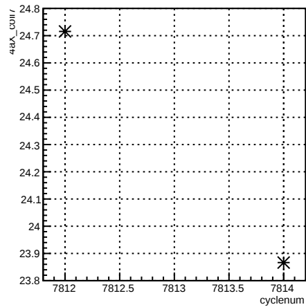
4aX_coil7:cyclenum {run == 7044}
