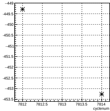
4aX_coil1:cyclenum {run == 7044}
