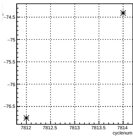
4aX_coil3:cyclenum {run == 7044}
