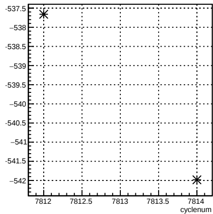
4eX_coil1:cyclenum {run == 7044}
