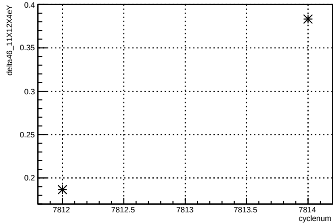
delta46_11X12X4eY:cyclenum {run == 7044}
