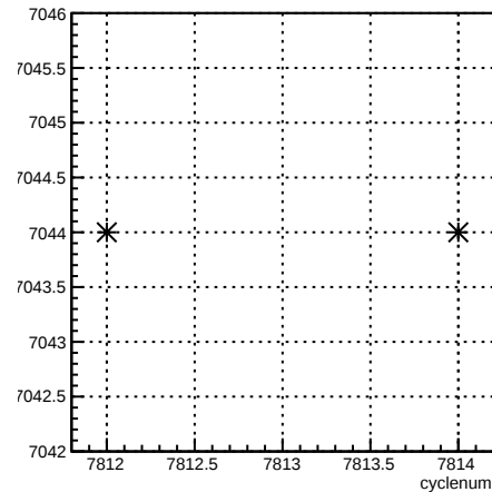
run:cyclenum {run == 7044}
