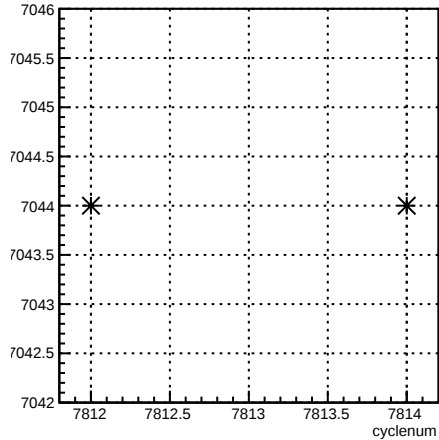
run:cyclenum {run == 7044}
