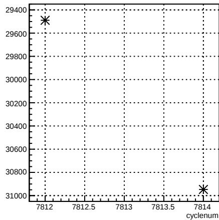
usr_coil6:cyclenum {run == 7044}
