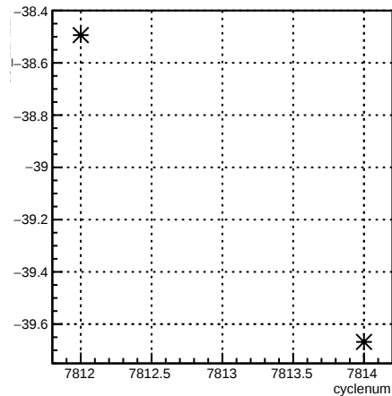
usl_11X12X:cyclenum {run == 7044}
