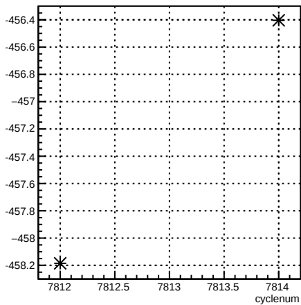
11X12X_coil7:cyclenum {run == 7044}
