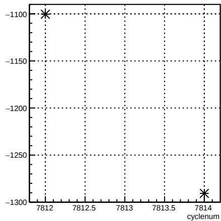
usl_coil6:cyclenum {run == 7044}
