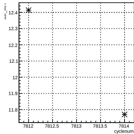
usr_4eY:cyclenum {run == 7044}
