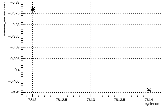
delta13_11X12X4eX:cyclenum {run == 7044}
