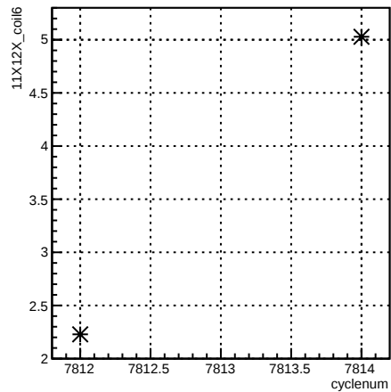
11X12X_coil6:cyclenum {run == 7044}
