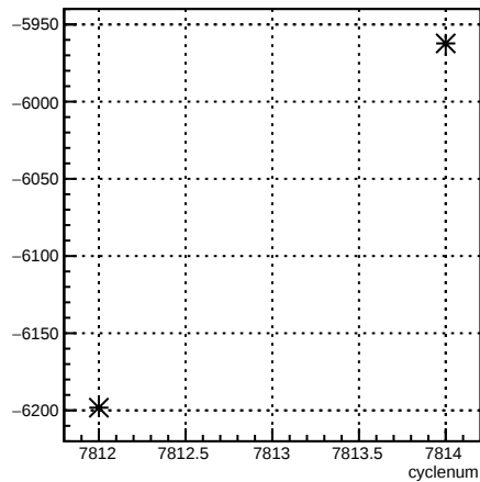
usr_coil7:cyclenum {run == 7044}
