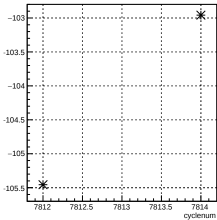
4eX_coil3:cyclenum {run == 7044}
