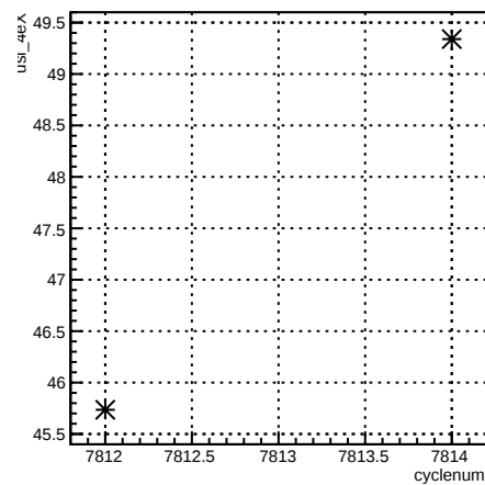
usl_4eX:cyclenum {run == 7044}
