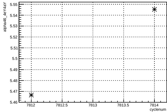
alpha46_4eY4aY:cyclenum {run == 7044}
