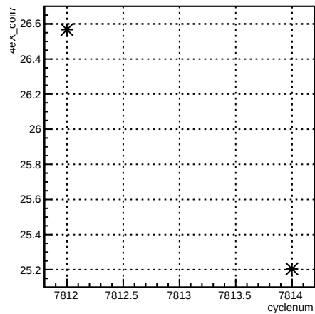
4eX_coil7:cyclenum {run == 7044}
