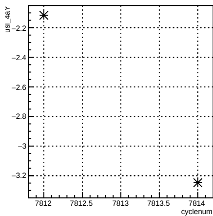
usl_4aY:cyclenum {run == 7044}
