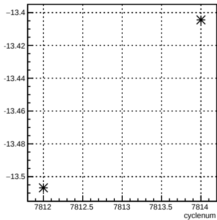
4eY_coil6:cyclenum {run == 7044}
