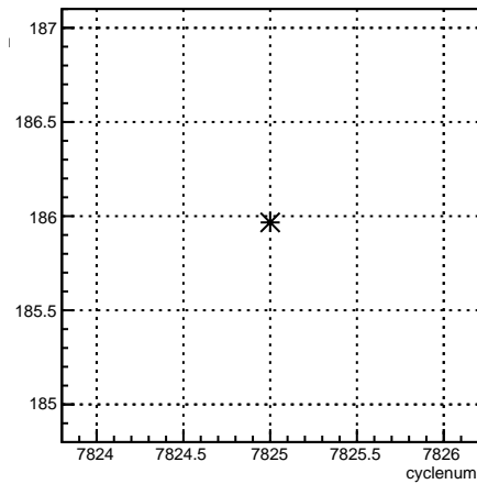
run:cyclenum {run == 7046}
