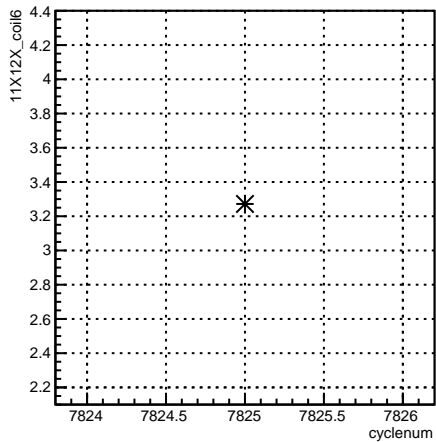
11X12X_coil6:cyclenum {run == 7046}
