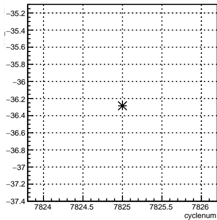
usr_11X12X:cyclenum {run == 7046}
