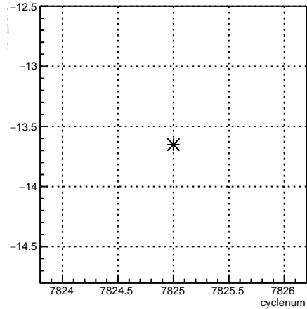
4eY_coil6:cyclenum {run == 7046}
