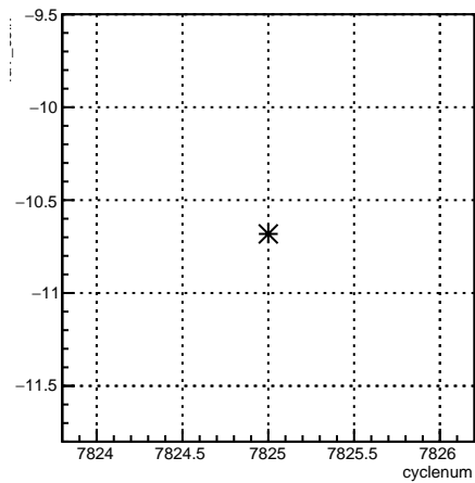
4aY_coil7:cyclenum {run == 7046}
