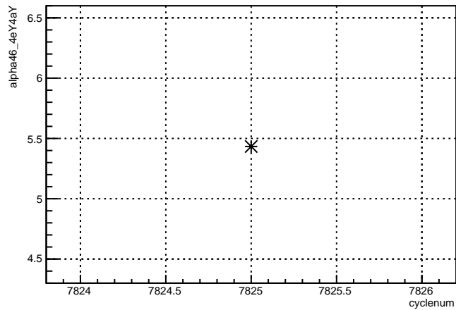
alpha46_4eY4aY:cyclenum {run == 7046}
