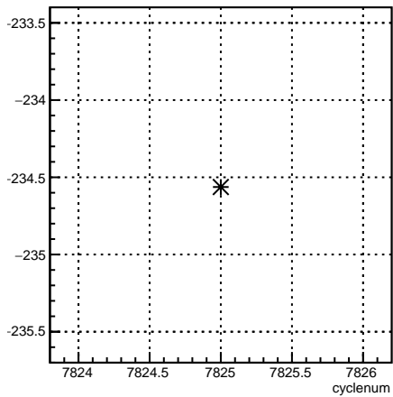
11X12X_coil6:cyclenum {run == 7046}
