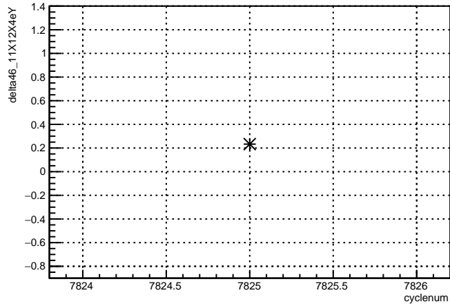
delta46_11X12X4eY:cyclenum {run == 7046}
