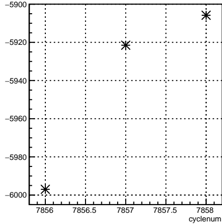
usr_coil7:cyclenum {run == 7062}
