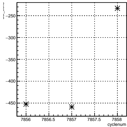
usl_coil6:cyclenum {run == 7062}
