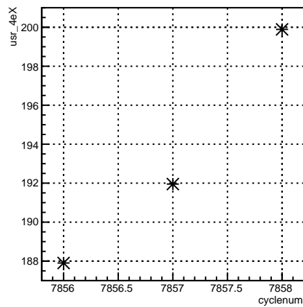
usr_4eX:cyclenum {run == 7062}
