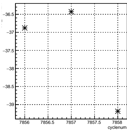
usr_11X12X:cyclenum {run == 7062}
