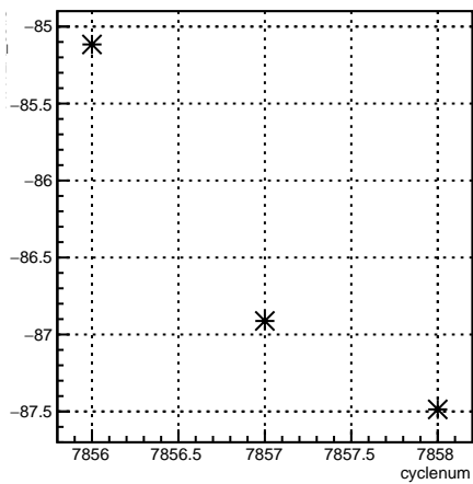
11X12X_coil3:cyclenum {run == 7062}
