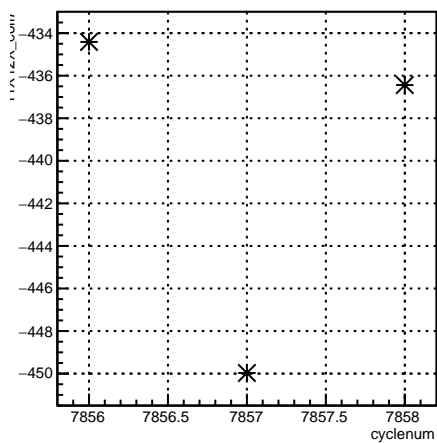
11X12X_coil7:cyclenum {run == 7062}
