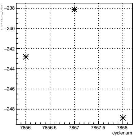
11X12X_coil1:cyclenum {run == 7062}
