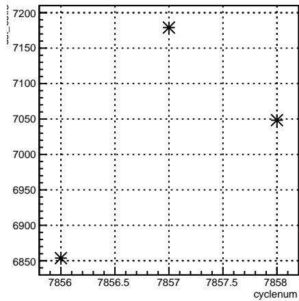
usl_coil7:cyclenum {run == 7062}
