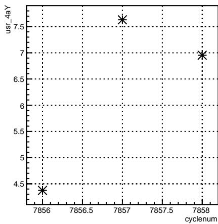
usr_4aY:cyclenum {run == 7062}
