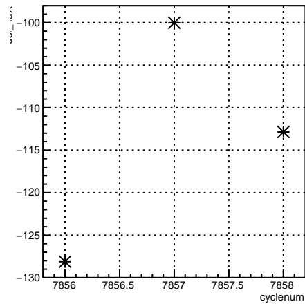
usl_4eY:cyclenum {run == 7062}
