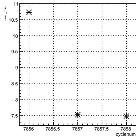
usr_4eY:cyclenum {run == 7062}
