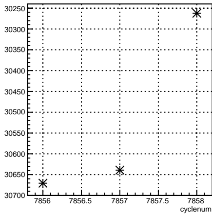
usr_coil6:cyclenum {run == 7062}
