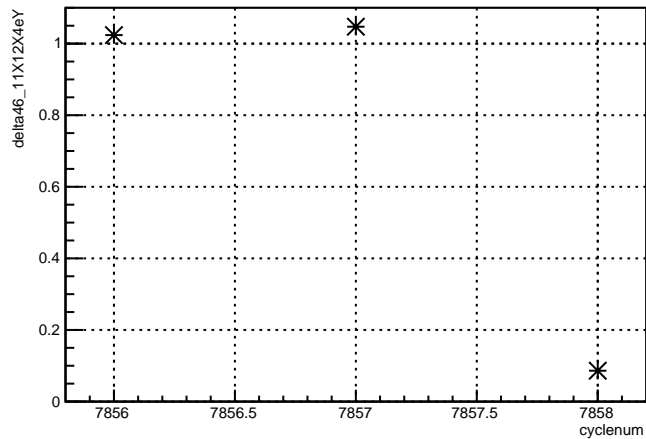
delta46_11X12X4eY:cyclenum {run == 7062}
