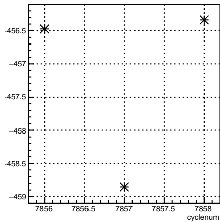
4eX_coil1:cyclenum {run == 7062}
