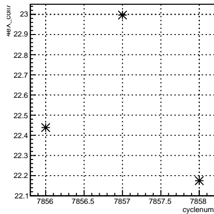
4eX_coil7:cyclenum {run == 7062}
