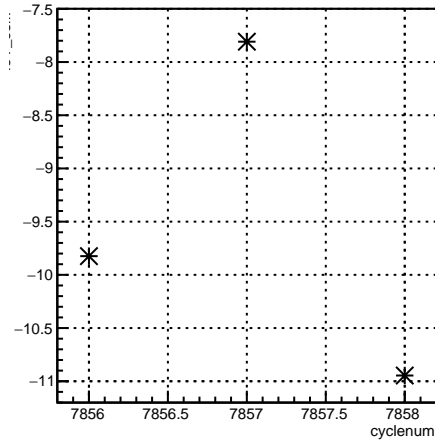
4eY_coil7:cyclenum {run == 7062}
