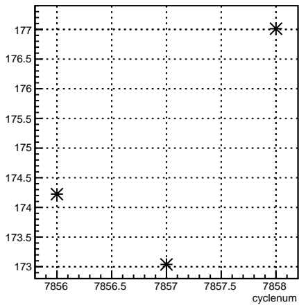
4eY_coil4:cyclenum {run == 7062}
