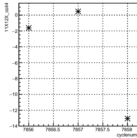
11X12X_coil4:cyclenum {run == 7062}
