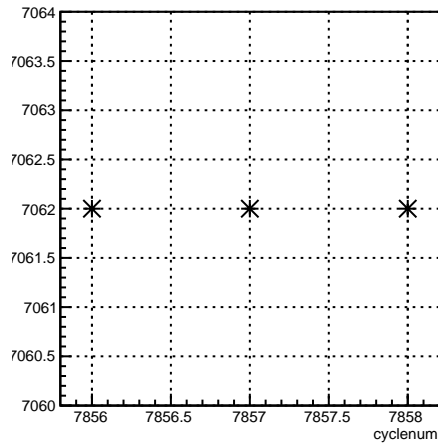
run:cyclenum {run == 7062}
