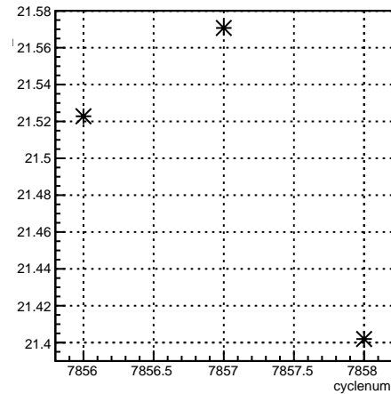
4aX_coil7:cyclenum {run == 7062}
