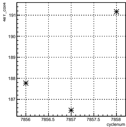
4eY_coil4:cyclenum {run == 7062}
