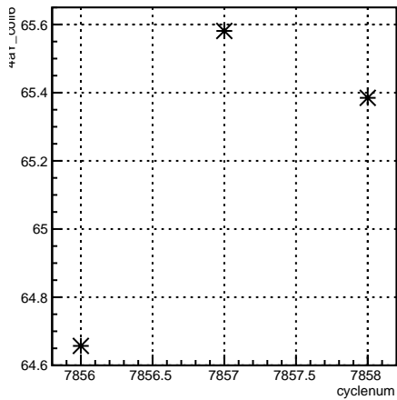
4eY_coil6:cyclenum {run == 7062}
