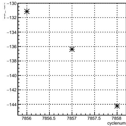
usr_4aX:cyclenum {run == 7062}
