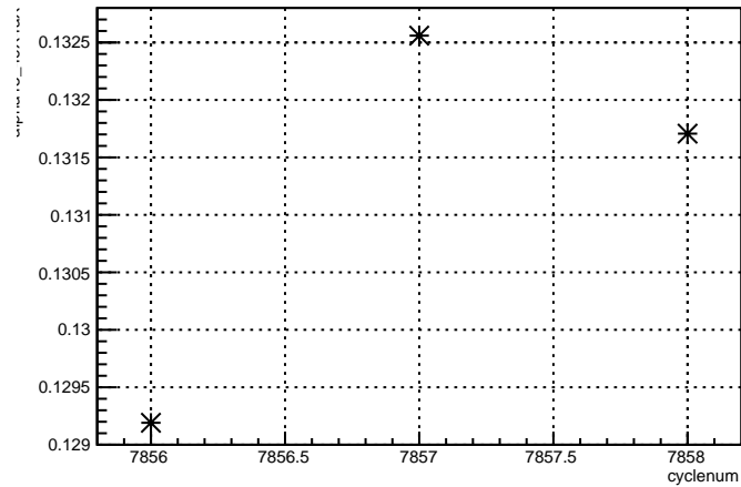
delta13_11X12X4eX:cyclenum {run == 7062}
