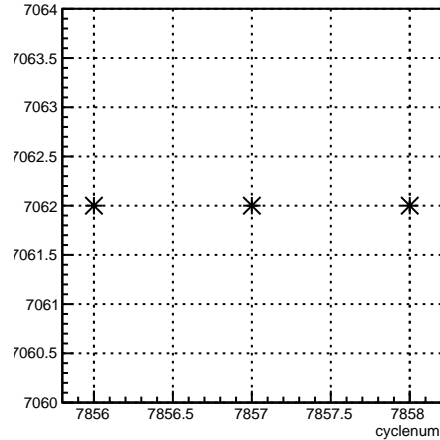
run:cyclenum {run == 7062}
