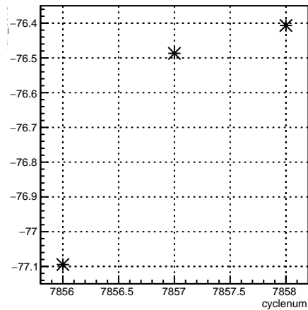
4eX_coil3:cyclenum {run == 7062}
