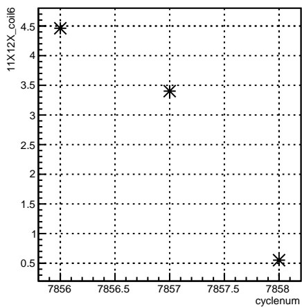
11X12X_coil6:cyclenum {run == 7062}
