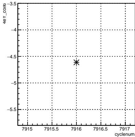
4eY_coil6:cyclenum {run == 7074}
