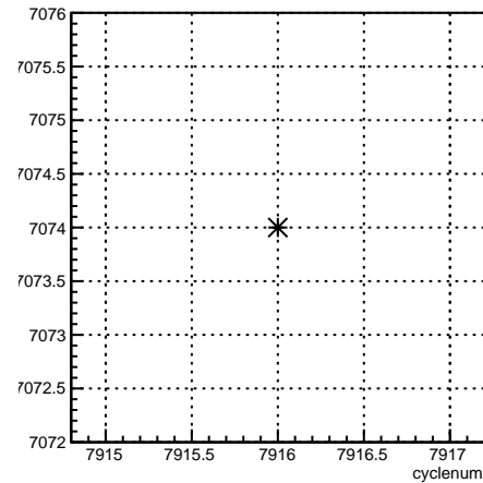
run:cyclenum {run == 7074}
