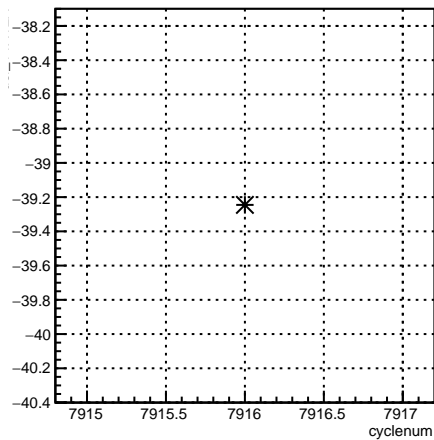
usl_11X12X:cyclenum {run == 7074}
