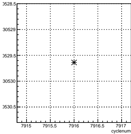
usr_coil1:cyclenum {run == 7074}
