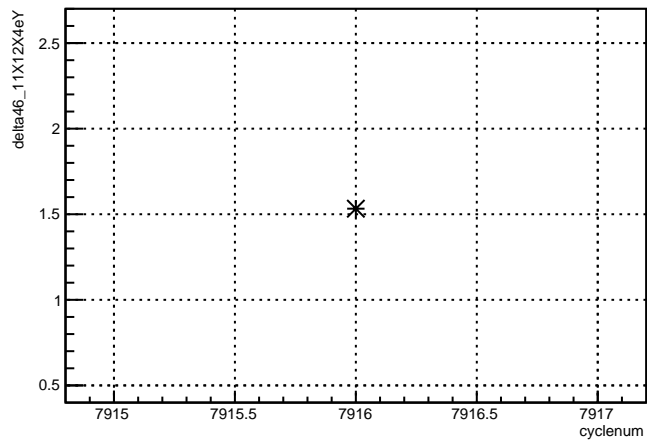
delta46_11X12X4eY:cyclenum {run == 7074}
