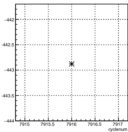
11X12X_coil7:cyclenum {run == 7074}
