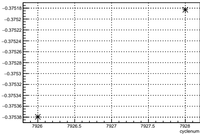
delta13_11X12X4eX:cyclenum {run == 7077}
