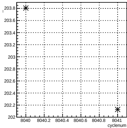
run:cyclenum {run == 7110}
