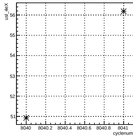
run:cyclenum {run == 7110}
