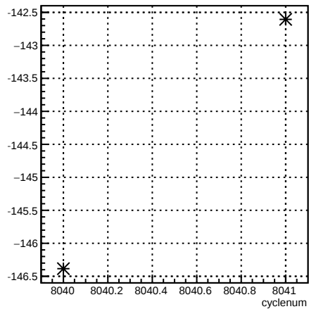
usr_4eY:cyclenum {run == 7110}
