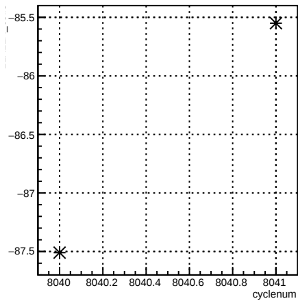
11X12X_coil3:cyclenum {run == 7110}
