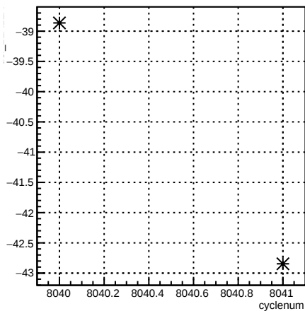
usl_11X12X:cyclenum {run == 7110}
