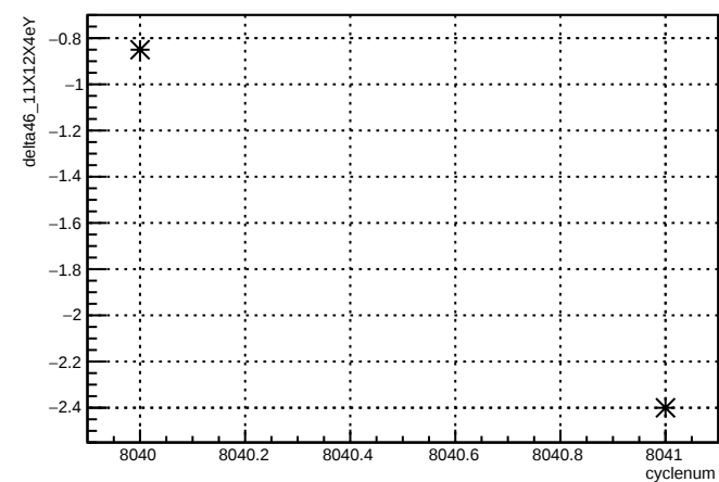
delta46_11X12X4eY:cyclenum {run == 7110}
