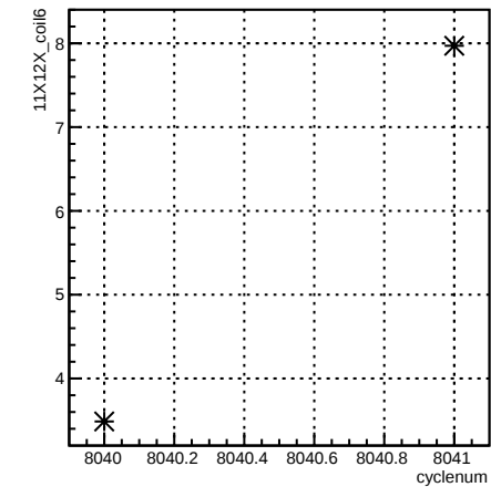
11X12X_coil6:cyclenum {run == 7110}
