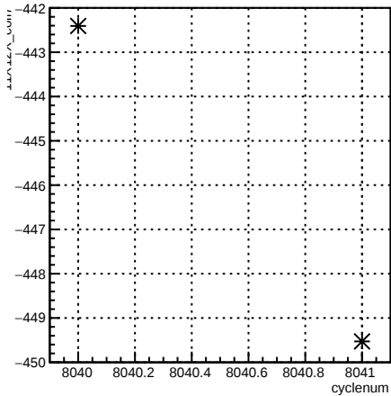
11X12X_coil7:cyclenum {run == 7110}
