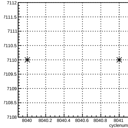
run:cyclenum {run == 7110}
