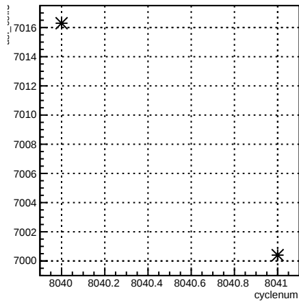
usl_coil7:cyclenum {run == 7110}
