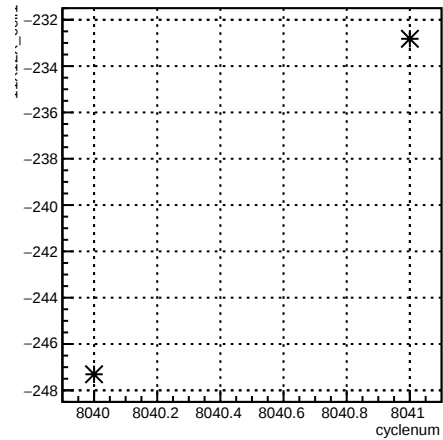
11X12X_coil1:cyclenum {run == 7110}
