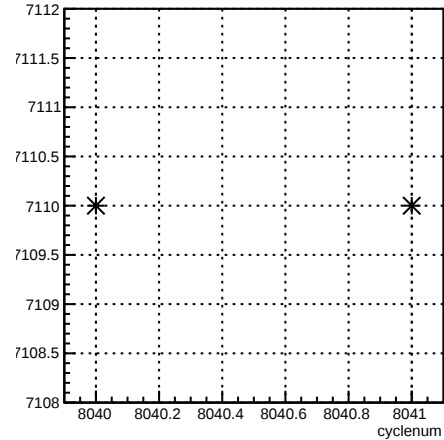
run:cyclenum {run == 7110}
