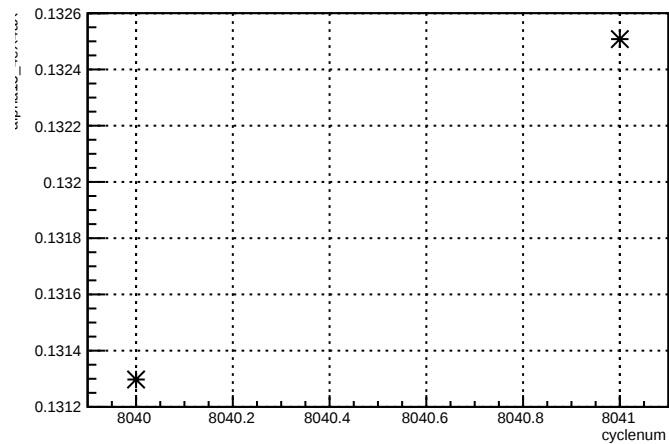
alpha13_4eX4aX:cyclenum {run == 7110}
