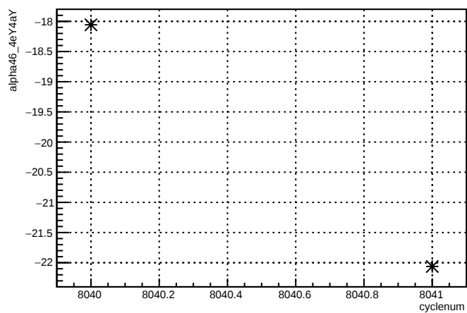
alpha46_4eY4aY:cyclenum {run == 7110}
