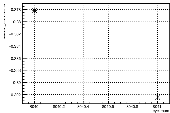
delta13_11X12X4eX:cyclenum {run == 7110}
