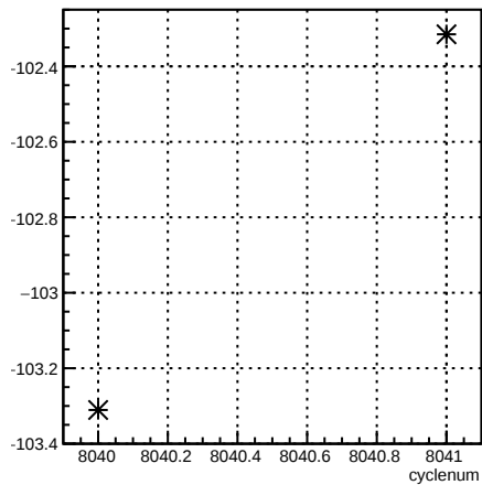
4eX_coil3:cyclenum {run == 7110}
