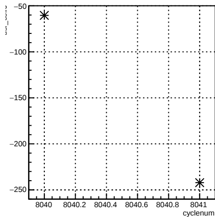
usr_coil6:cyclenum {run == 7110}
