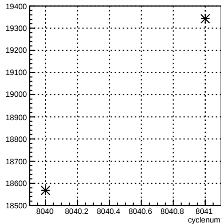
usr_coil7:cyclenum {run == 7110}
