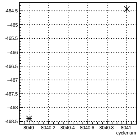
4eX_coil1:cyclenum {run == 7110}
