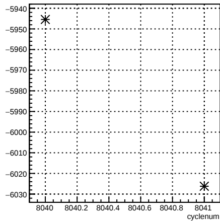
usr_coil7:cyclenum {run == 7110}
