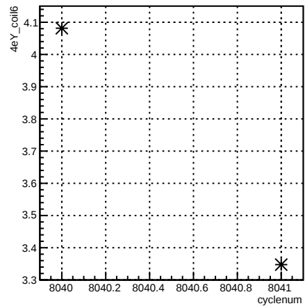
4eY_coil6:cyclenum {run == 7110}
