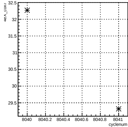
4eX_coil7:cyclenum {run == 7110}
