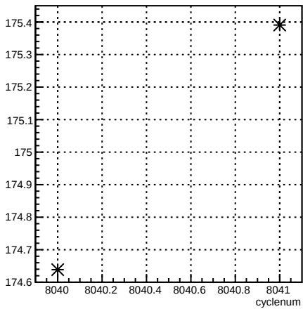
4eY_coil4:cyclenum {run == 7110}
