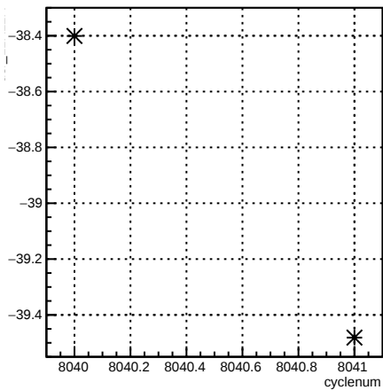
usr_11X12X:cyclenum {run == 7110}
