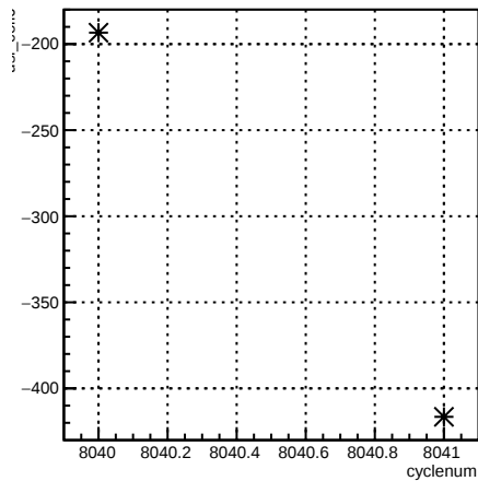
usl_coil6:cyclenum {run == 7110}
