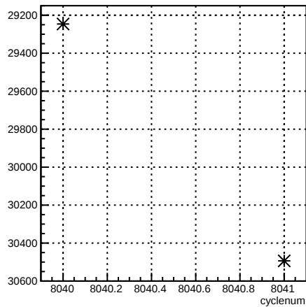
usr_coil6:cyclenum {run == 7110}
