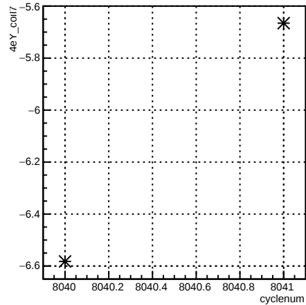
4eY_coil7:cyclenum {run == 7110}
