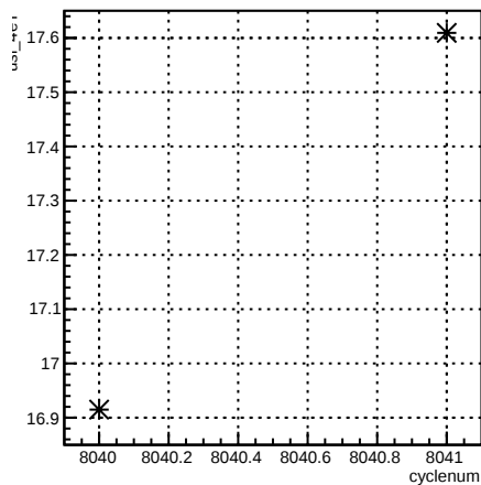
usl_4eY:cyclenum {run == 7110}
