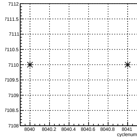
run:cyclenum {run == 7110}
