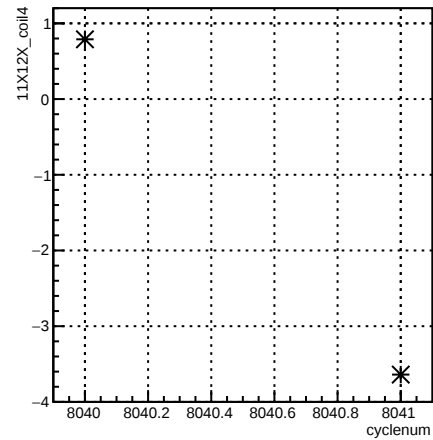
11X12X_coil4:cyclenum {run == 7110}
